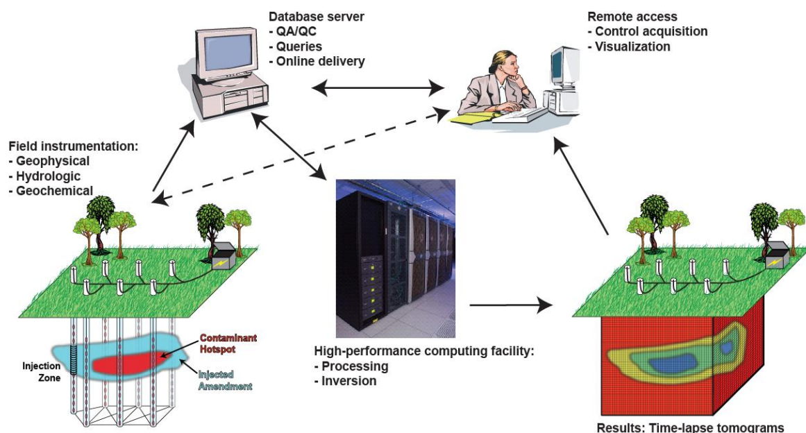
Figure 2-1 Schematic of the HPMS. Data is collected in the field, and transmitted to a server for qa/qc and parsing in a relational database. Processing and inversion is done on a HPC cluster. Results (including time lapse tomograms) are accessible to endusers through a browser interface).
