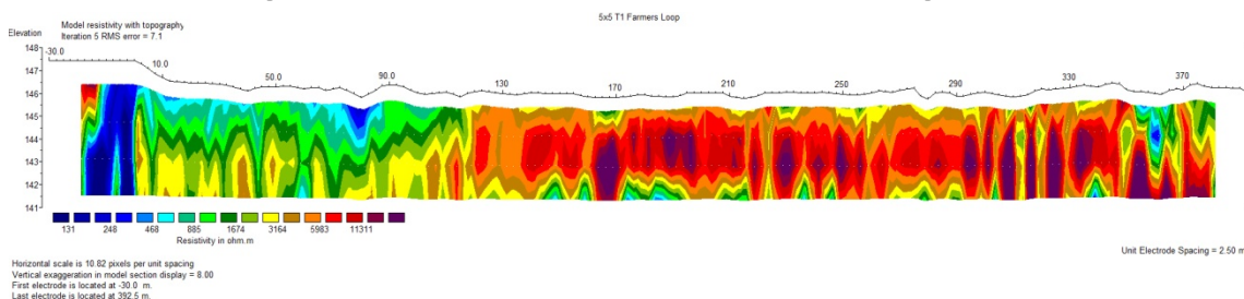
Figure 25. The Farmers Loop T1 CCR with a 5 \times 5 configuration.
