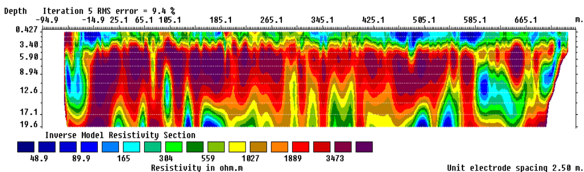
Figure 33. The composite Tunnel CCR survey conducted upslope from the tunnel portal.
