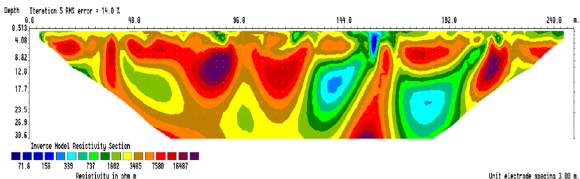
Figure 21. The first section of the Permafrost Tunnel transect composite ERT pseudo-section.
