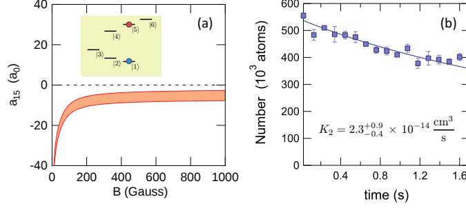
Figure 10: Stable, weakly-interacting two-state mixture of ^6\text{Li} fermions. (a) The s -wave scattering length a_{15} for a |1\rangle - |5\rangle mixture of ^6\text{Li} atoms as a function of field as predicted by a simple coupled channels model. The range of scattering lengths shown are for different choices of model parameters. (b) Decay of the |1\rangle - |5\rangle mixture in a gas with an initial density of 2.5 \times 10^{13} atoms/cm ^3 in each spin state. The decay is due to a weak dipolar loss with a measured two-body inelastic loss rate coefficient K_2 = 2.3^{+0.9}_{-0.4} \times 10^{-14} cm ^3 /s.
