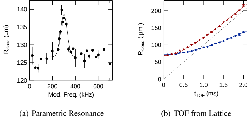
Figure 7: Realization of 1D thermal gases of ^6\text{Li} fermions by confinement in a 2D triangular lattice. (a) Parametric resonance demonstrating that the oscillation frequency in the tight radial direction of each lattice site \omega_{\perp} \simeq 2\pi \times 150 kHz. (b) Time-of-flight expansion of ^6\text{Li} atoms from the 2D optical lattice. The clear anisotropic expansion of this non-interacting Fermi gas results from the fact that the zero-point energy in the radial direction of each tube (red) is larger than the thermal energy along the axis of the tube (blue) indicating that the 1D regime has been achieved. The dashed line shows the predicted expansion for a single tube occupying the harmonic oscillator ground state for \omega_{\perp} = 2\pi \times 150 kHz (i.e. the dashed line corresponds to R_{\text{cloud}} = \sqrt{\frac{\hbar\omega_{\perp}}{m}} t_{\text{TOF}} ).
