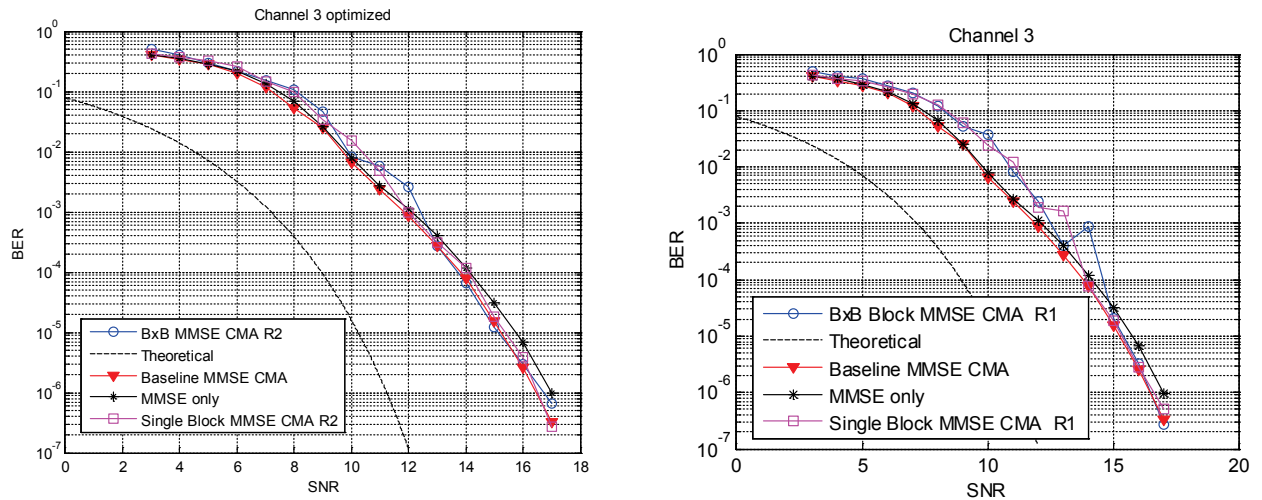
Fig. 4: Single Packet Processing and Block-by-Block CMA Equalizer for channel 3 R_2 = 2 (left) versus R_l = 1 (right)
