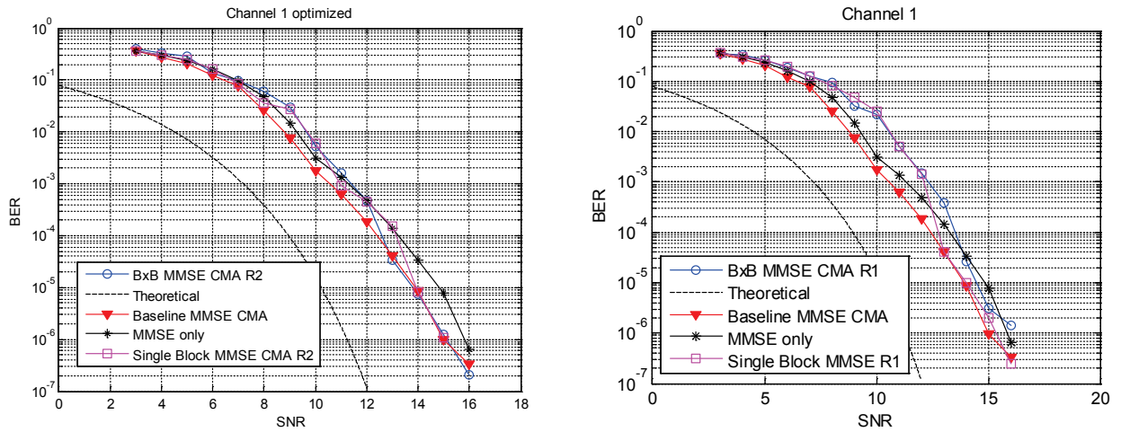
Fig. 3: Single Packet Processing vs. Block-by-Block CMA Equalizer for Channel 1 R_2 = 2 (left) versus R_l = 1 (right)
