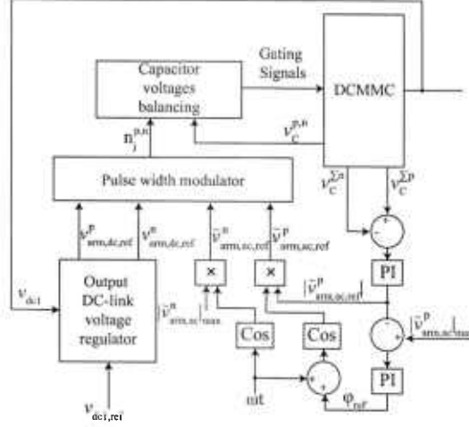
Figure 27: Overall block diagram of the proposed PCC.
