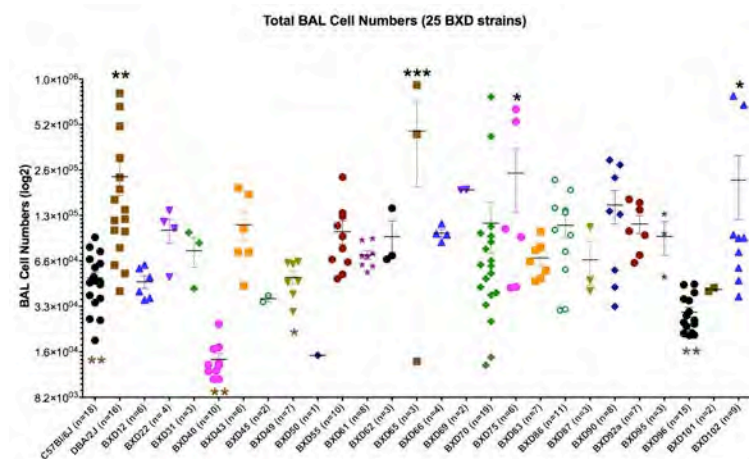
Figure 2. Differential recruitment of immune cells into the lungs of BXD strains following pulmonary infection with Acinetobacter baumannii . BXD mice were challenged with 1 \times 10^7 CFU Ab via the intranasal route. The mice were sacrificed 24 hr later and bronchiolar lavage (BAL) was performed. BAL cells were counted using a Scepter cell counter. Statistical analysis was performed using one-way ANOVA using Dunnett post tests to compare each of the BXD strains with the C57Bl/6 (statistical significance is indicated in black) and with the DBA/2J mice (statistical significance indicated in brown). Statistical significance is as follows: p < 0.05 *, p < 0.01 **, and p < 0.001 ***.
