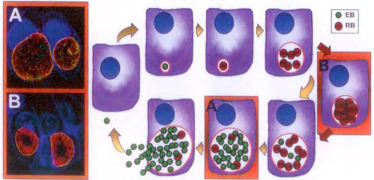
FIGURE 1 Schematic diagram of the chlamydial developmental cycle. Red arrows indicate altered intracellular chlamydial development mediated by environmental factors. (A) Immunofluorescence images and schematic show mature C. trachomatis serovar B inclusions with elementary bodies (EBs) in green (anti-OmcB), reticulate bodies (RBs) in red (anti-major outer membrane protein), and the inclusion membrane in orange (anti-incG). (B) Persistence in vitro in response to IFN-γ results in enlarged, aberrant RBs that can be maintained in this state for extended periods of time, with subsequent reversion to normal intracellular development. doi:10.1128/9781555817329.ch12.f1
