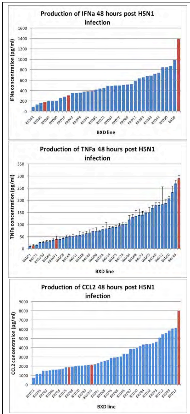
Figure 1: Production of pro-inflammatory cytokines 48 hours post inoculation with Highly pathogenic H5N1 influenza A virus. The production of IFNα 1 (top), TNFα (middle) and CCL2 (bottom) in 43 different BXD lines and the parental DBA/2, C57BL/6 plus the F1 strain. The red bars indicate (from left to right) C57BL/6, B6D2F1 and DBA/2J. Fewer strains were tested for the production of IFNα.
