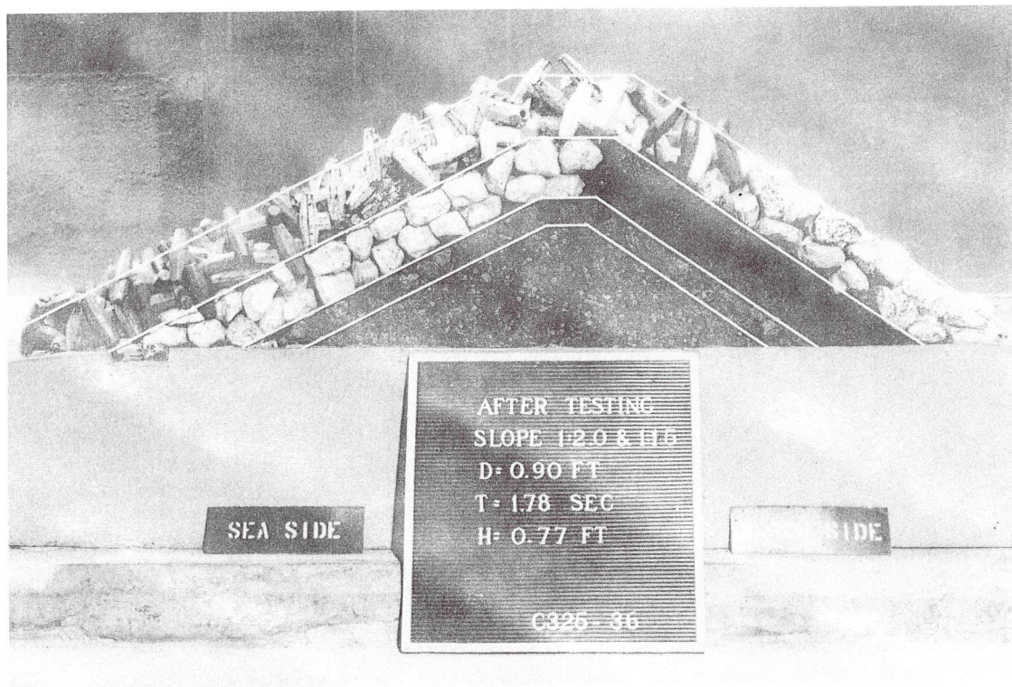
Photo 8. End view after attack of 1.78-sec, 0.77-ft waves; d = 0.90 ft; W_a = 0.589 lb; 1V-on-2H structure slope; dolos armor
