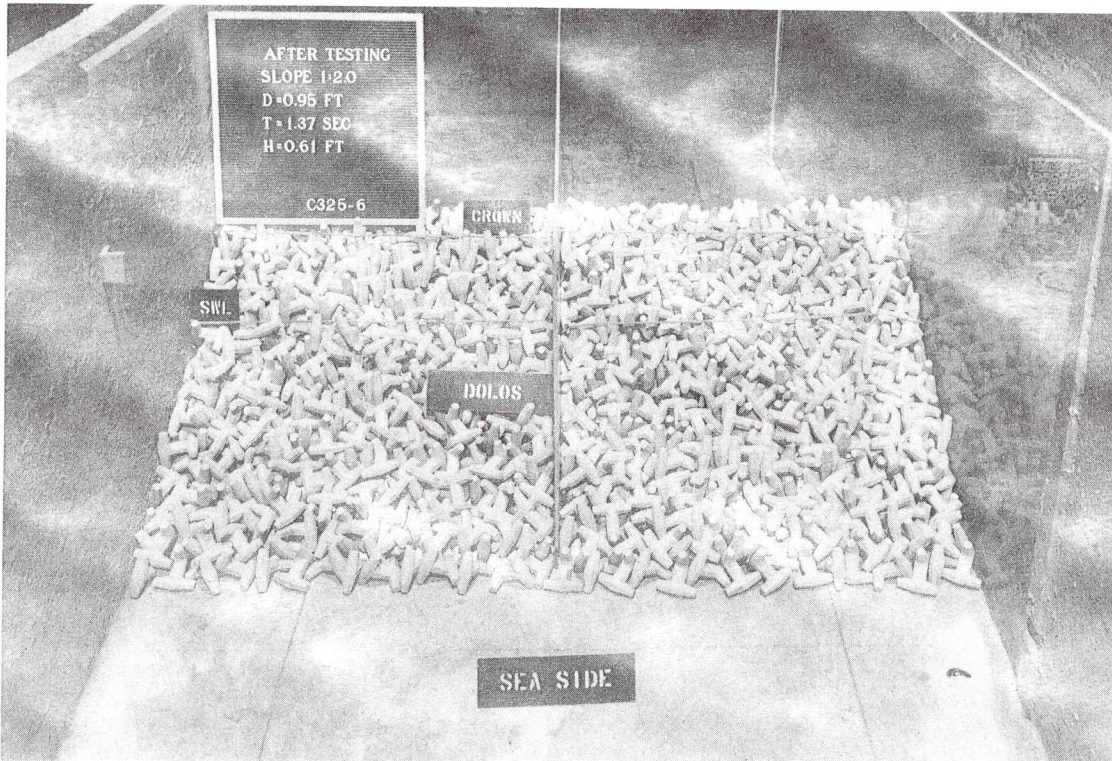
Photo 5. Sea-side view after attack of 1.37-sec, 0.61-ft waves; d = 0.95 ft; W_a = 0.276 lb; 1V-on-2H structure slope; dolos armor
