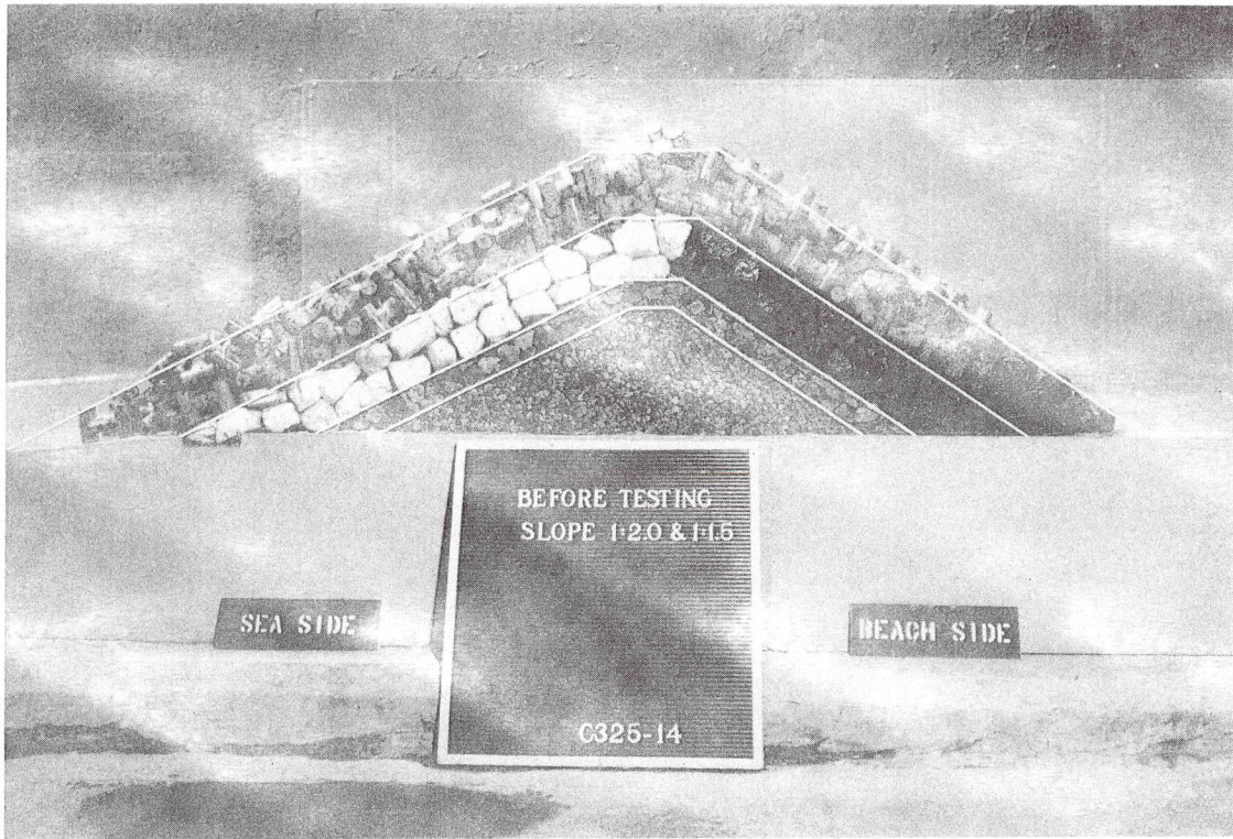
Photo 3. End view of a typical tribar section before wave attack at a 1V-on-2H sea-side structure slope; W_a = 0.627 \text{ lb}
