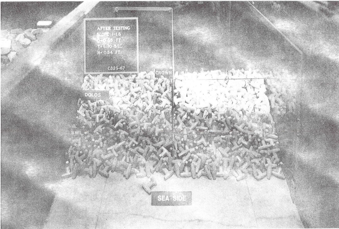
Photo 13. Sea-side view after attack of 1.70-sec, 0.54-ft waves; d = 0.55 ft; W_a = 0.589 lb; 1V-on-1.5H structure slope; dolos armor
