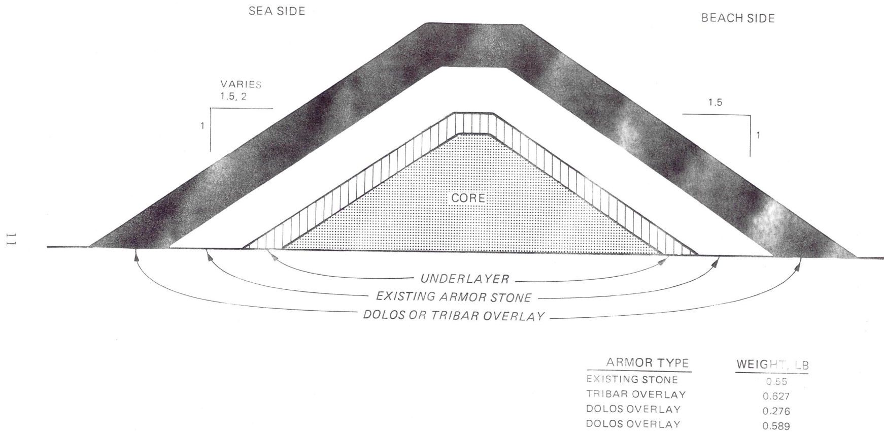
Figure 1. Typical breakwater cross section
