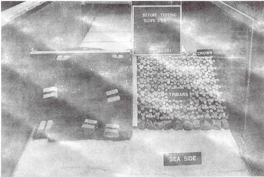
Photo 17. Sea-side view of uniformly placed tribar armor before wave attack at a 1V-on-1.5H structure slope
