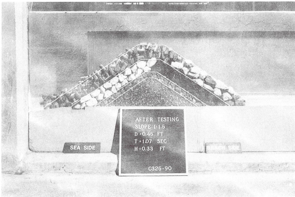
Photo 16. End view after attack of 1.07-sec, 0.33-ft waves; d = 0.45 ft; W_a = 0.627 lb; 1V-on-1.5H structure slope; tribar armor
