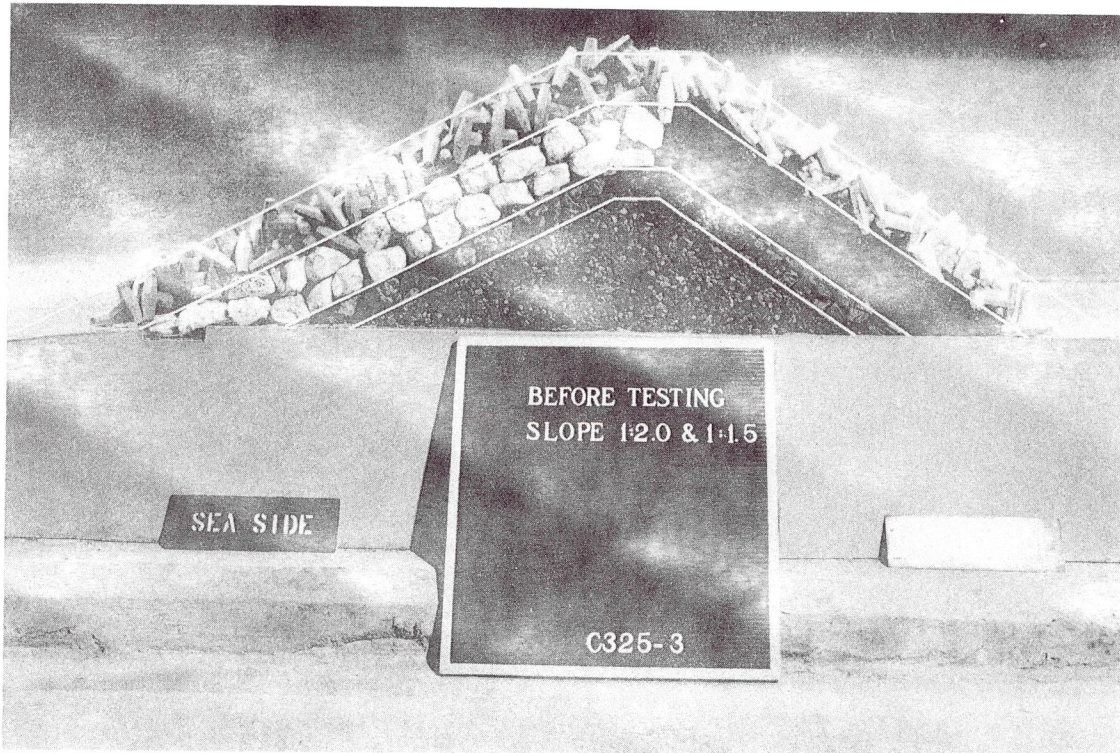
Photo 1. End view of a typical dolos section before wave attack at a 1V-on-2H sea-side structure slope; W_a = 0.276 \text{ lb}
