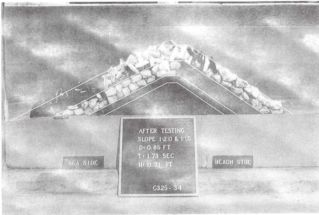
Photo 7. End view after attack of 1.73-sec, 0.71-ft waves; d = 0.85 ft; W_a = 0.589 lb; 1V-on-2H structure slope; dolos armor
