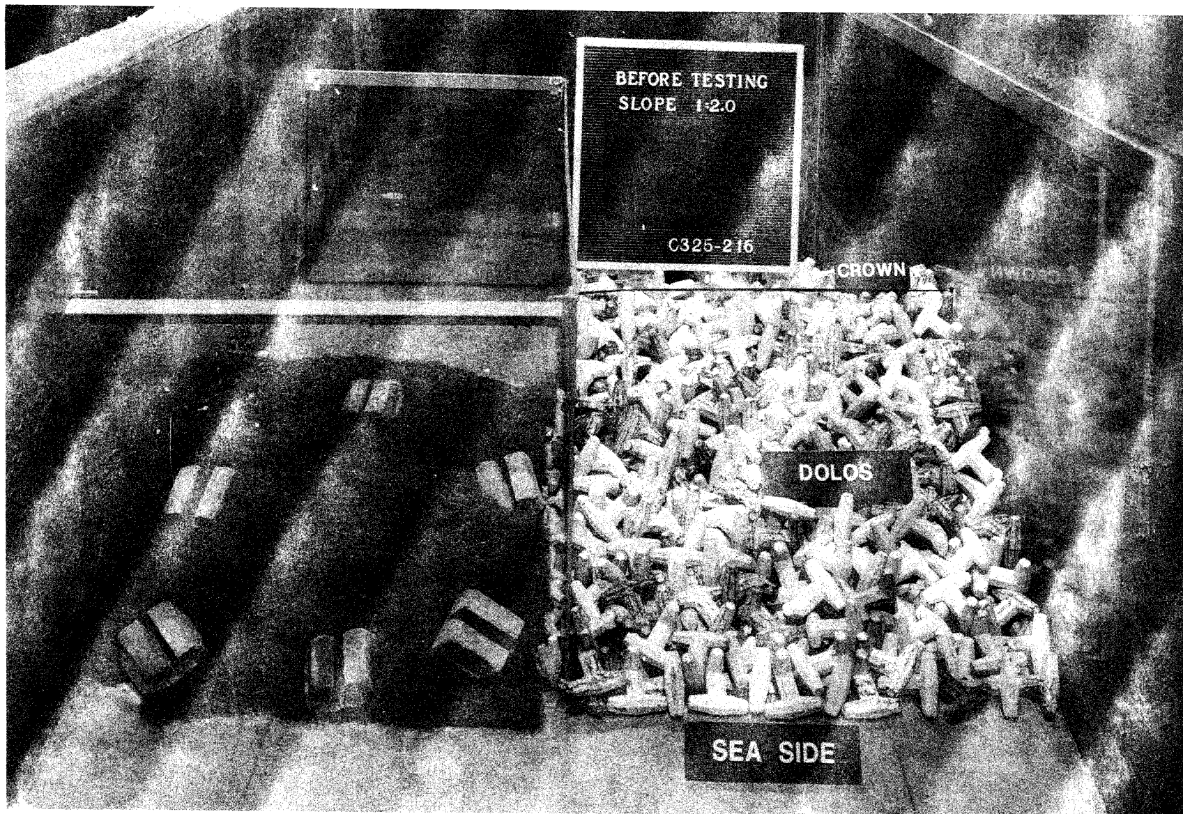
Photo 4. Sea-side view of a typical test section before wave attack at a 1V-on-2H sea-side structure slope; W_a = 0.589 \text{ lb}
