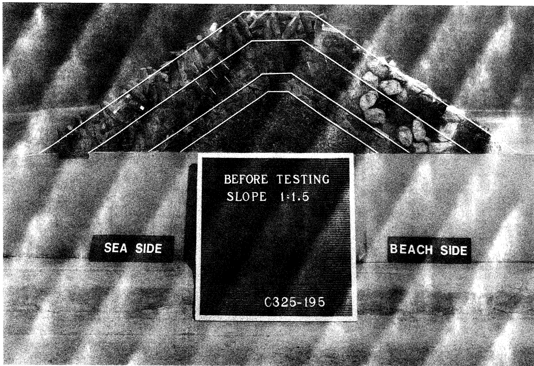
Photo 1. End view of a typical test section before wave attack at a 1V-on-1.5H sea-side structure slope; W_a = 0.442 \text{ lb}
