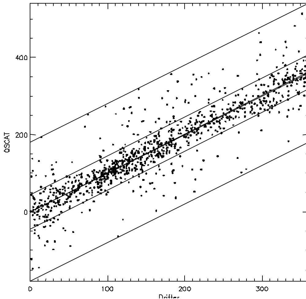
Figure 1. Comparison of QuikSCAT and observed wind direction in the Japan East Sea [Scatter plot shows agreement between QuikSCAT wind direction and observed wind direction from drifters.]
