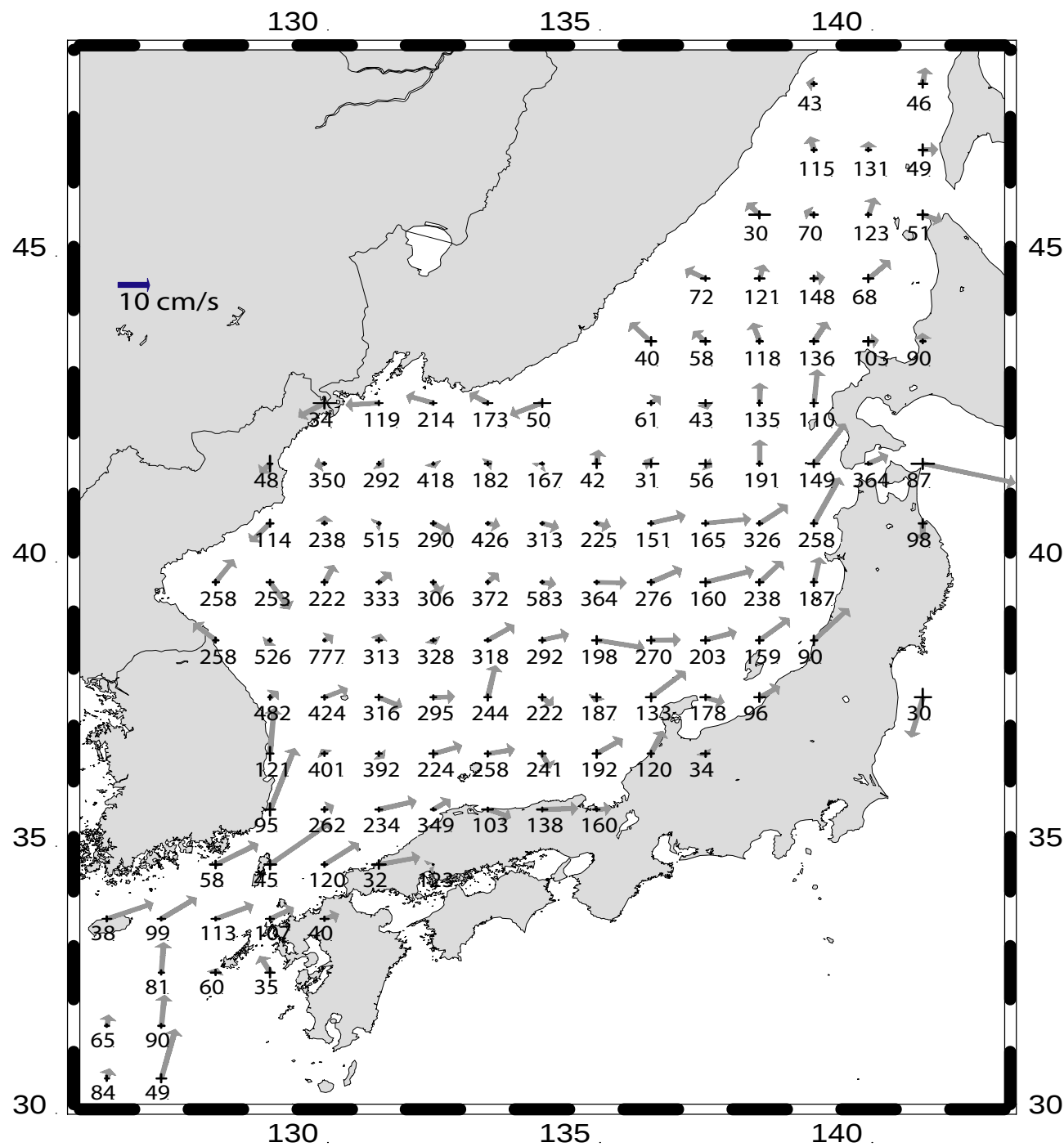
Figure 2. Mean Current and Standard Error [Plot of mean current and standard error. Computation of the mean velocity and the eddy energy is now more complete spatially]
