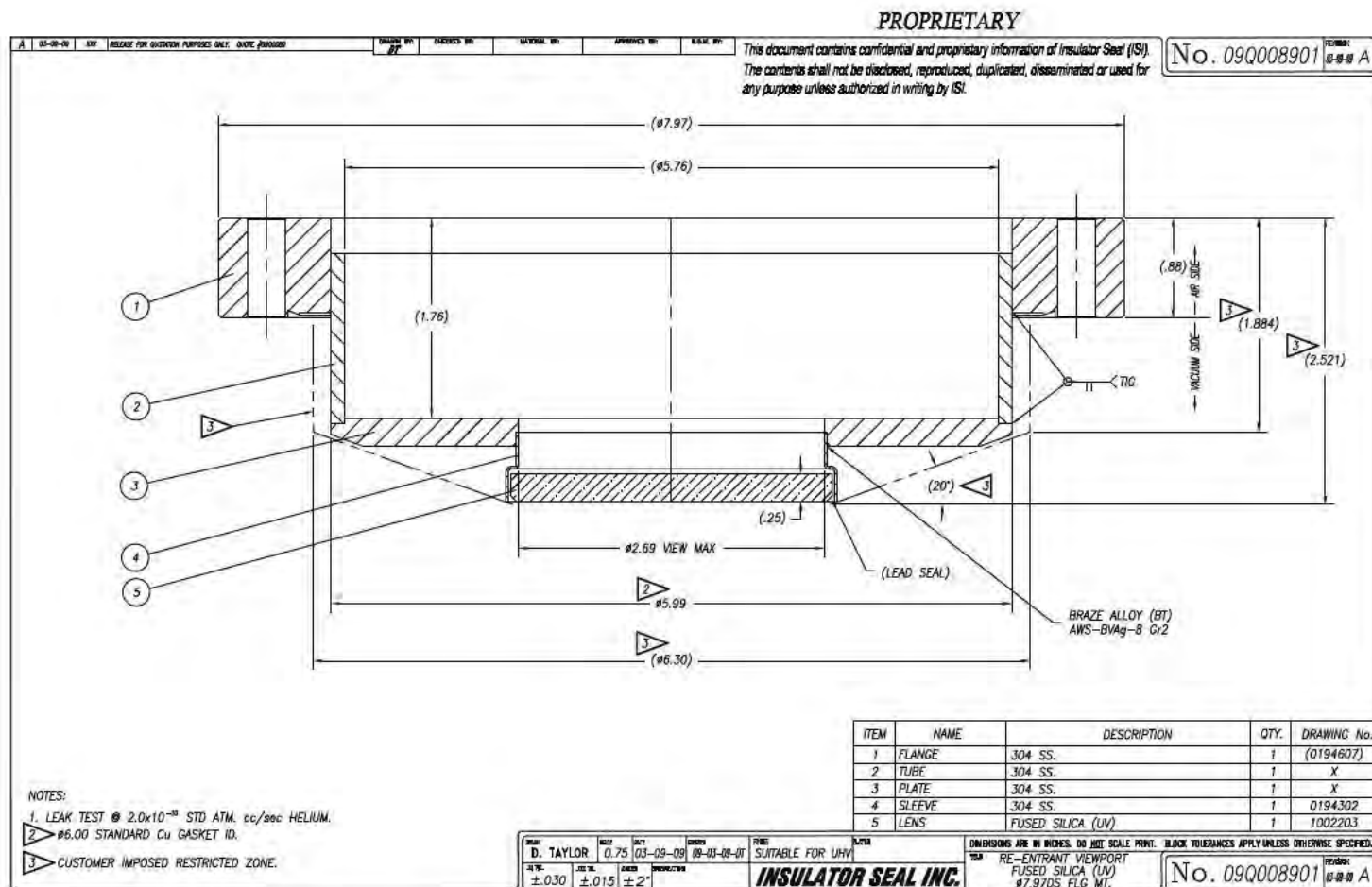
Figure A.1: Manufacturer's drawing for the recessed "bucket" windows. While a standard 8" copper gasket does fit per note 2, the clearance is so tight it would be easier to use a larger ID gasket, such as those sold by Kimball Physics. The lead glass-to-metal seal limits bakeout temperature to 150 °C. Written permission was obtained to include the drawing in this dissertation.
