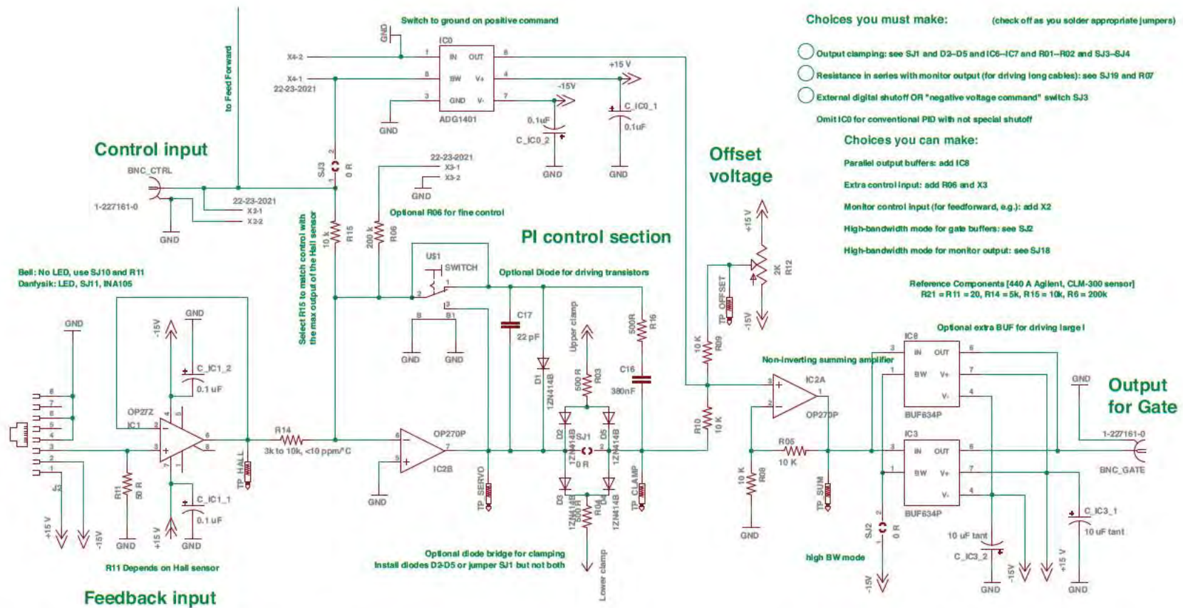
Figure 3.16: PI circuit for magnet coil current control. The corresponding monitor, power, and feed-forward circuits are in Fig. 3.17.
