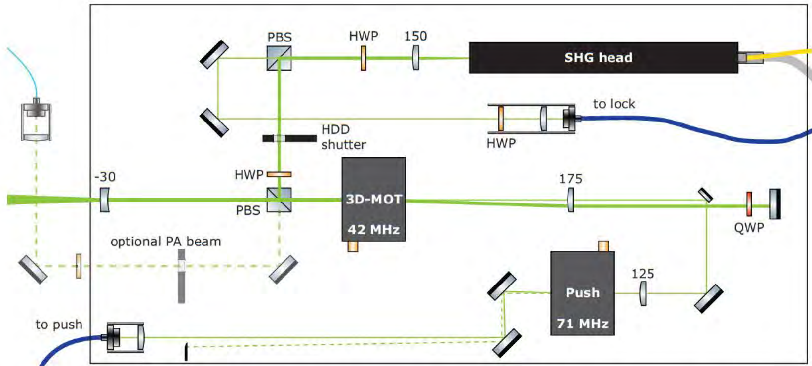
Figure 3.29: Optical schematic for distribution of 555.8 nm cooling light. Lens focal lengths are given in mm. On the left-hand side is an optional fiber launch for a photoassociation (PA) beam.
