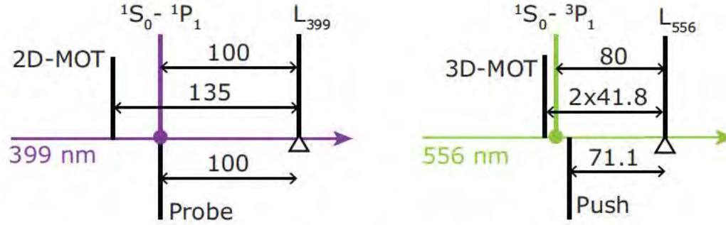
Figure 3.26: AOM shifts and lock-points for the Yb laser systems. All frequencies are given in MHz and 2× represents a double-passed AOM.
