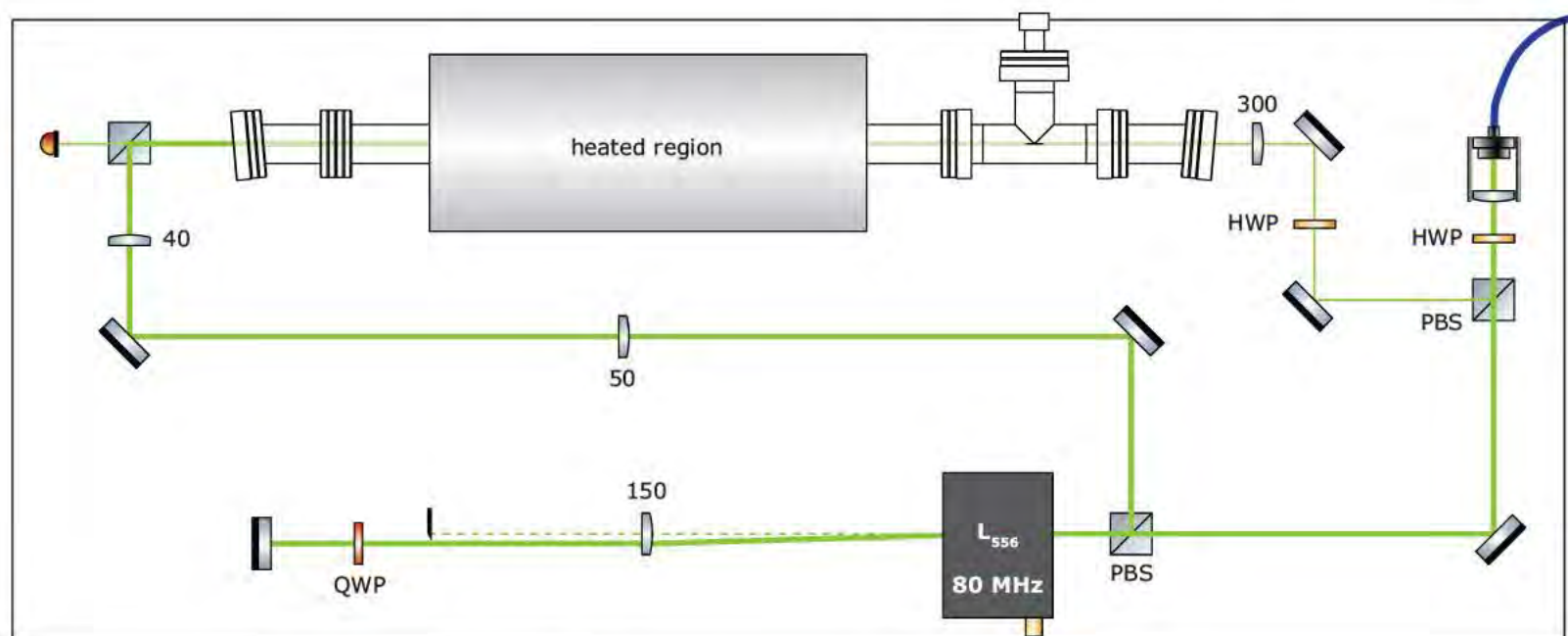
Figure 3.30: Optical schematic for the 555.6 nm lock.
