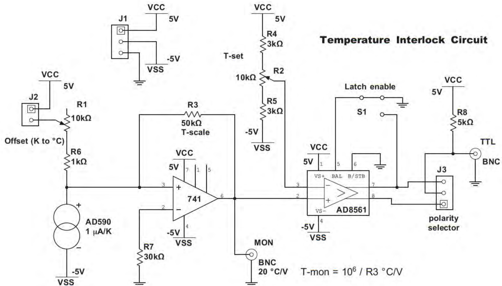
Figure 3.11: Schematic of the temperature interlock for the Rb oven cold cup. The (remote) temperature sensor is an AD590, which acts as a current source. The optional offset (J2) makes the current 1 \mu A/°C with the appropriate adjustment of R1. With R3 = 50 \text{ k}\Omega , the transimpedance amplifier (741) produces a 20 °C/V signal. Finally, this is compared to the setpoint (adjusted with R2) with an AD8561 comparator, which provides a TTL level output to control an SSR.
