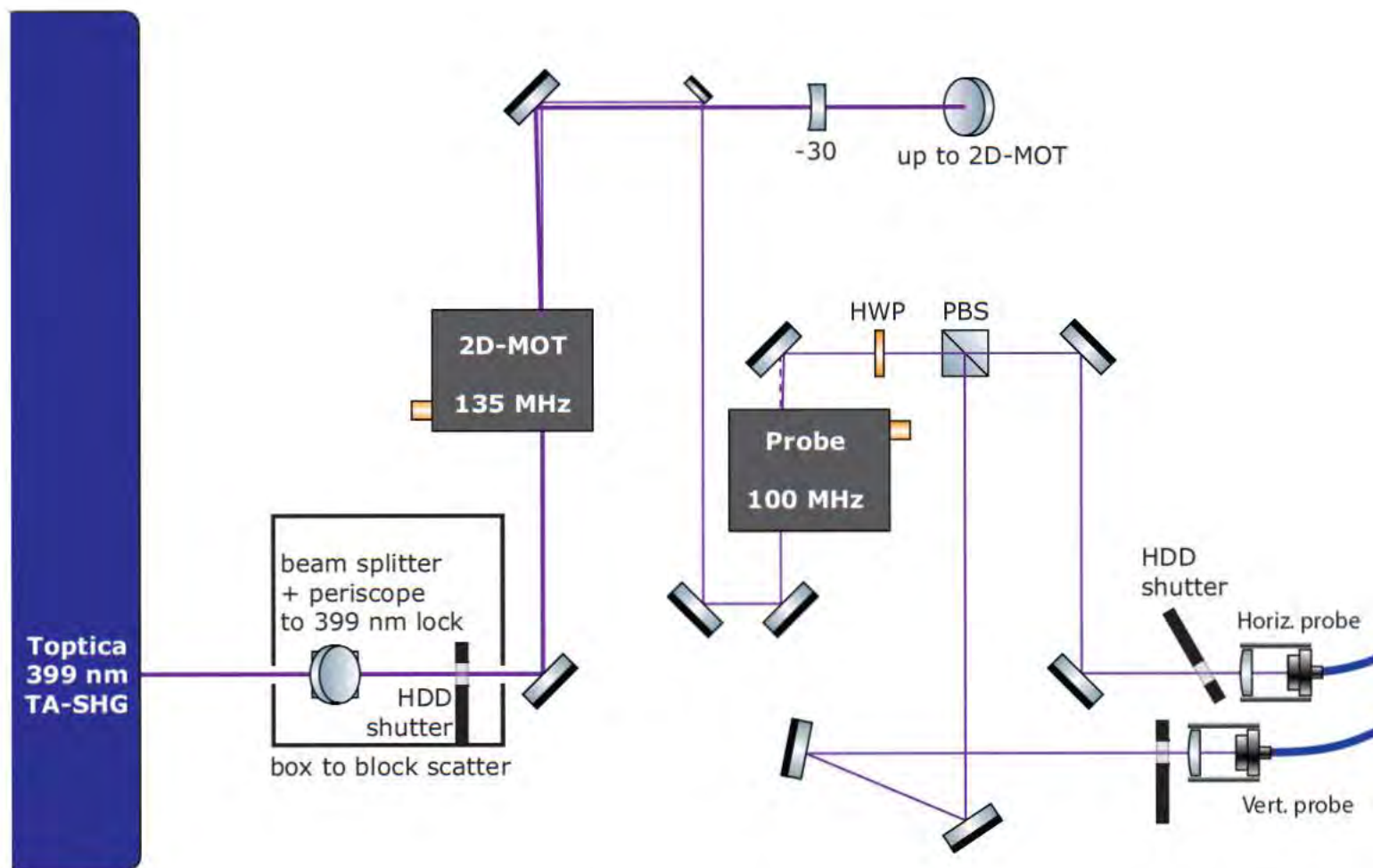
Figure 3.25: Division of the 398.9 nm light.
