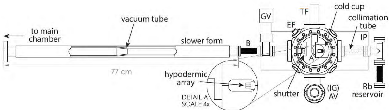
Figure 3.10: Rb source vacuum chamber. On the left, the center of the slower form has been cut away to reveal the diameter reduction in the vacuum tube. The slower tube is attached to the oven with a bellows (B) to relieve mechanical strain. Separate heaters are wrapped around the Rb reservoir and collimation tube and held at 110 and 140 °C, respectively. The length of the collimation tube is shown with a dotted line. Key —AV: angle valve, B: bellows, EF: electrical feedthrough for the shutter, GV: gate valve, IG: ion gauge (back), IP: ion pump, TF: thermal feedthrough.
