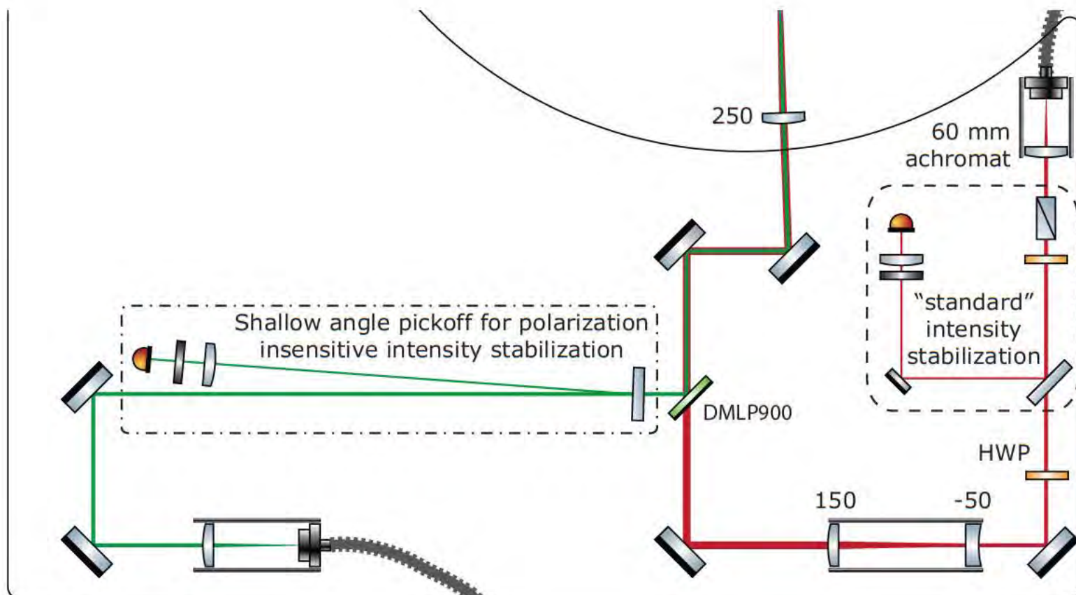
Figure 4.2: Fiber delaunch, combination and focussing optics for the 532 nm and 1064 nm coaxial dipole trap along the horizontal direction. The boxed regions show two implementations of intensity pick-offs for intensity stabilization. The reflectivity of the beam samplers is polarization dependent, so a Glan-laser polarizer defines a fixed pick-off fraction of the 1064 nm intensity (dashed box). As discussed later, the 532 nm polarization varies widely requiring the less precise shallow-angle pickoff shown in the dot-dashed box.
