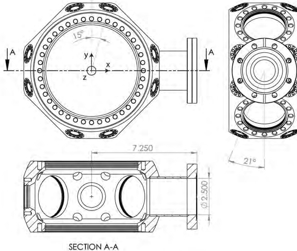
Figure 3.1: Customized main chamber (Kimball Physics MCF800-Cust-G2E5C3A16). Chosen laboratory coordinates are shown as well as polar and azimuthal angles for the mini-viewports.
