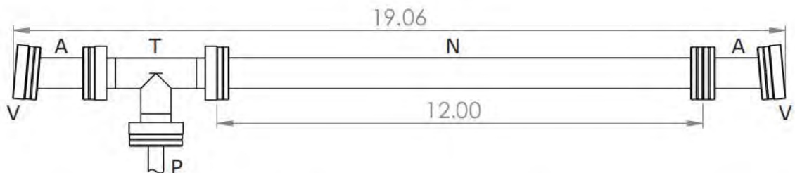
Figure 3.28: Yb heat pipe cell for 555.8 nm spectroscopy, with dimensions in inches. See the main text for a description of the labels.
