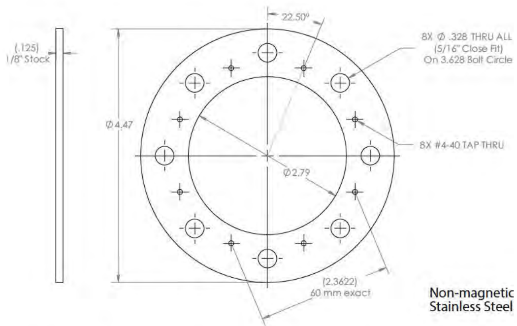
Figure A.3: 4.5" CF vacuum viewport "cage washers" to adapt to 60 mm cage system.
