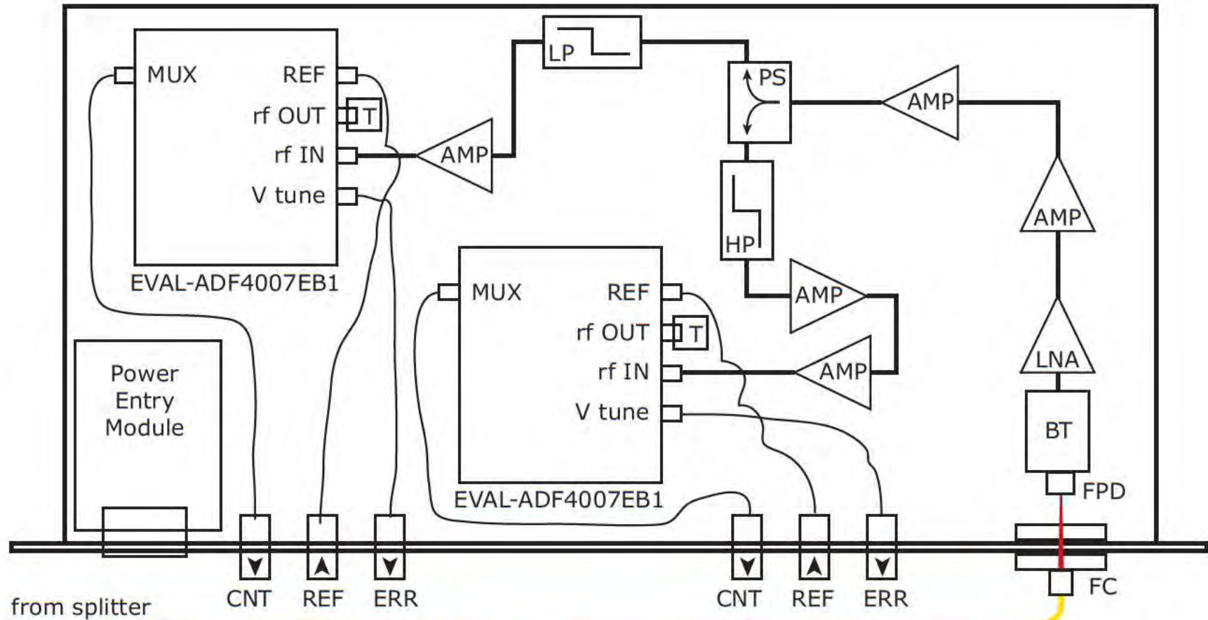
Figure 3.21: Rb beatnote lock schematic. Following schematic from bottom right— FC: FC-APC fiber port and asphere (Thorlabs A375TM-B), FPD: fast photo-detector (Hamamatsu G4176-03), BT: bias tee (Mini-Circuits ZX85-12G-S+), LNA: low-noise amp. 0.1 – 6 GHz (B&Z Technologies BZP106UB1X3), AMP: 12-16 dB amp. (Mini-Circuits ZX60-6013E+), PS: power splitter (Mini-Circuits ZFRSC-123-S+), LP: low-pass filter < 2.4 GHz (Mini-Circuits SLP-2400+), HP: high-pass filter > 2.5 GHz (Mini-Circuits VHF-2700+), T: 50 \Omega terminator.
