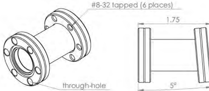
Figure 3.5: Short, angled 1.33 inch CF adapter nipple to eliminate back-reflection for dipole beams. The part was designed and manufactured by Nor-Cal, to our specifications.
