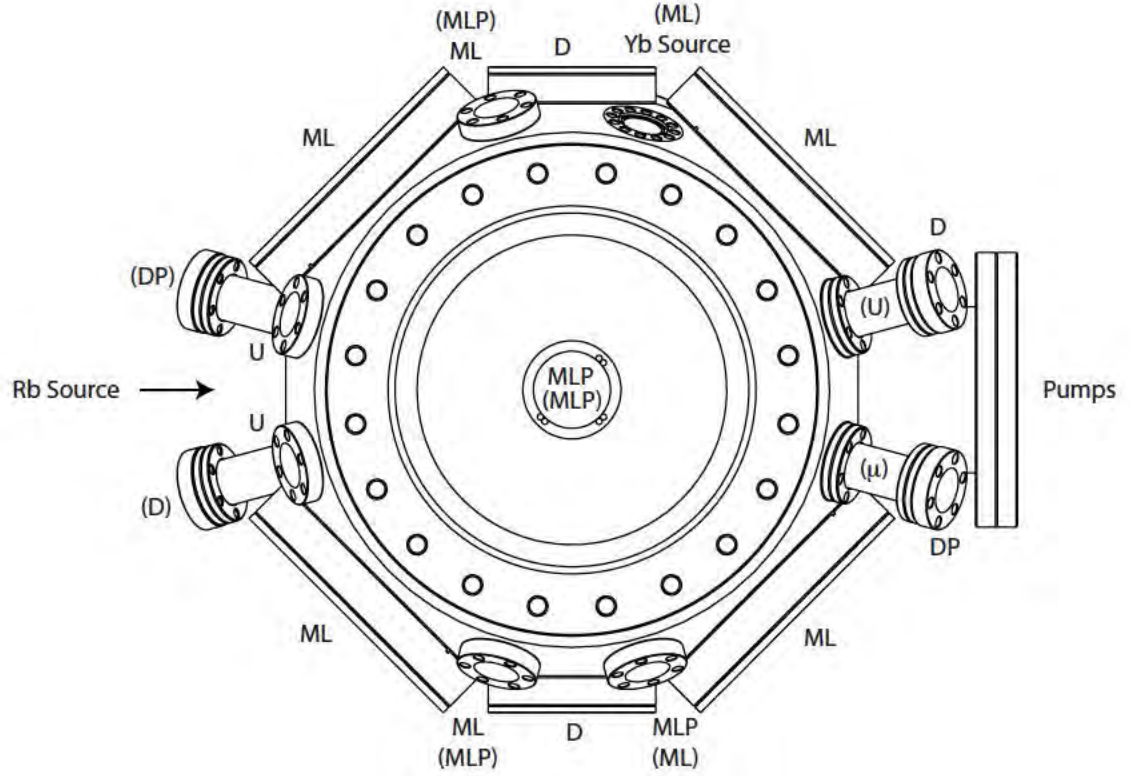
Figure 3.4: Schematic diagram (top view) of AR coatings on the main chamber vacuum windows. Windows are coated on both sides and matched with their opposing partner to reduce back-reflections. Coating key —D: dipole trap (532/1064 nm), L: lattice (423 nm), M: MOT (556/780 nm), P: probe (399/780 nm), U: uncoated, \mu : microwave feedthrough. Objects on the bottom are labeled in parenthesis. The Rb slower beam window at the end of the pump cross is coated for 780 nm.
