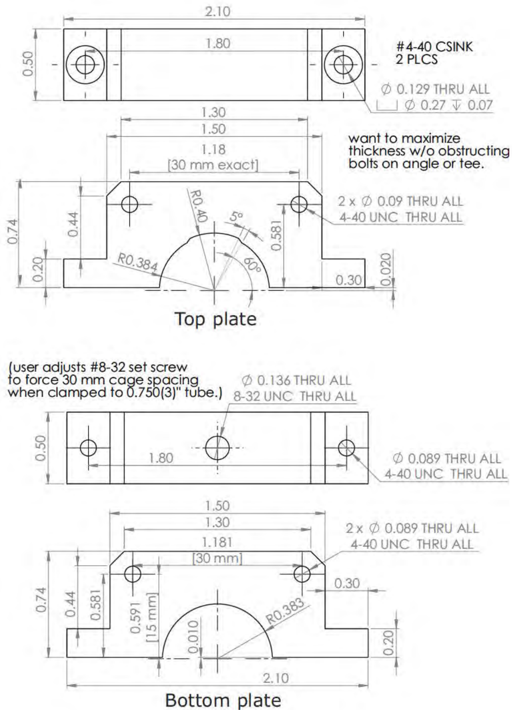
Figure A.5: Adapter for 0.75" tube (mini-CF) to 30 mm cage system. The separation between top and bottom clamp plates is intended to be defined by the set screw on the bottom plate. One should temporarily use a cage plate as close to the clamp to define the cage rod spacing when the clamp is installed. The clamp is shown attached to the chamber in the bottom left of Fig. 3.3.
