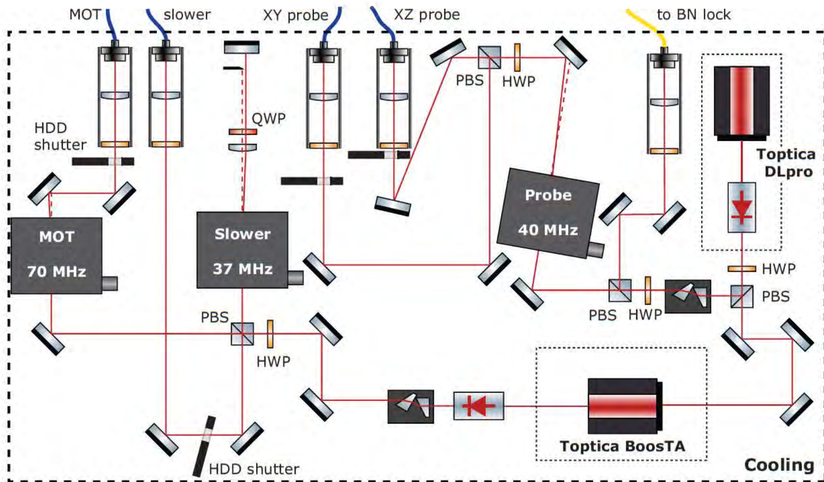
Figure 3.20: Rb Cooling light schematic.
