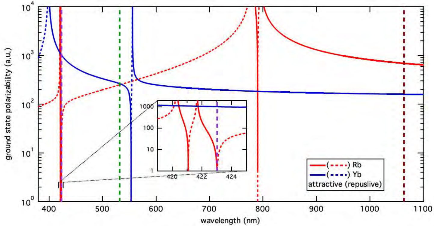
Figure 2.1: The ground state polarizability of Rb (red) and Yb (blue) in atomic units ( a_0^3 ). To display the variation of the polarizability over many decades, the magnitude is plotted with attractive (repulsive) polarizability as a solid (dashed) line. The Yb-only lattice laser at the zero in Rb polarizability (423.018(7) nm) is shown in the inset (purple vertical line); dipole trap colors are shown at 532 nm (green), where the polarizabilities are nearly equal but with opposite sign, and 1064 nm (dark red), which is roughly 4 times stronger for Rb than Yb.
