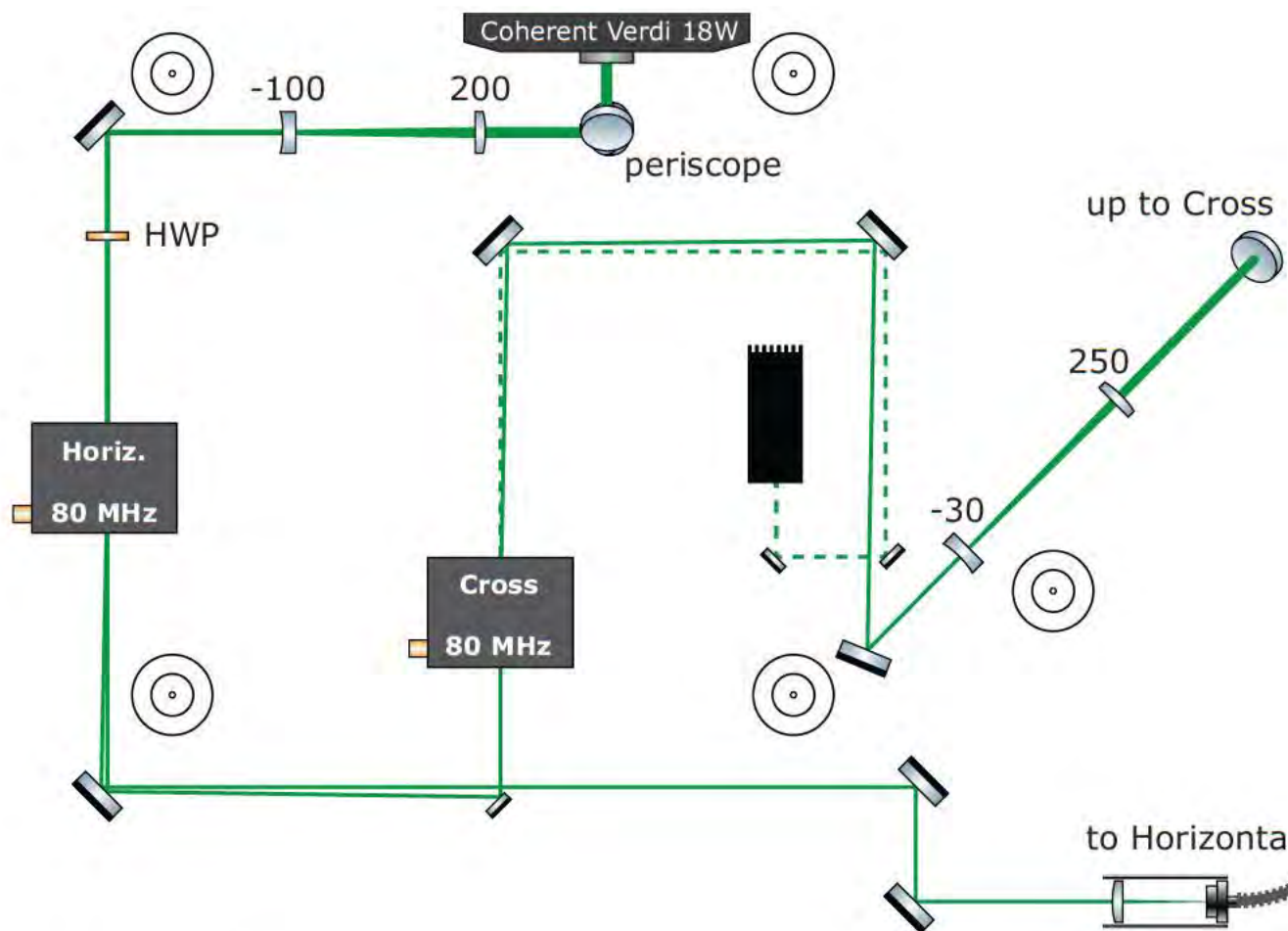
Figure 3.32: Division of the 532 nm laser into two dipole trapping beams. Lens focal length are given in mm.
