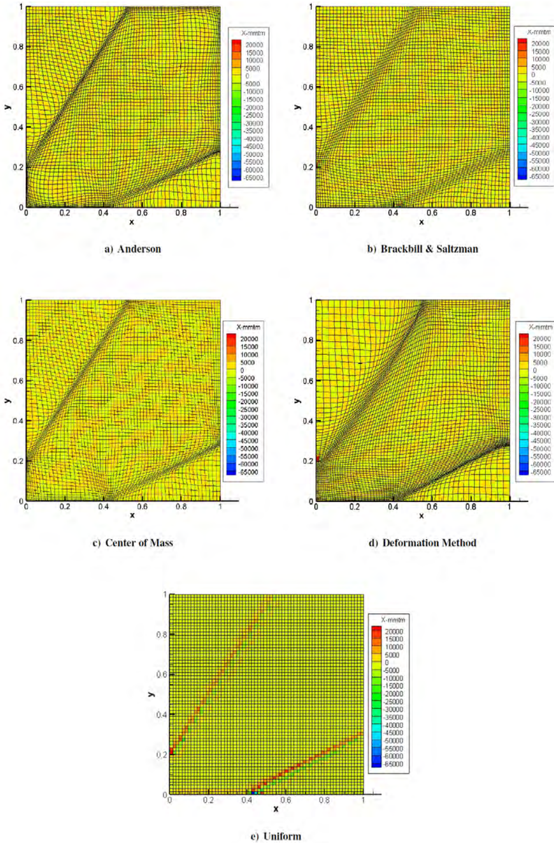
Figure 22. Truncation error for the x-momentum equation: edge case.
