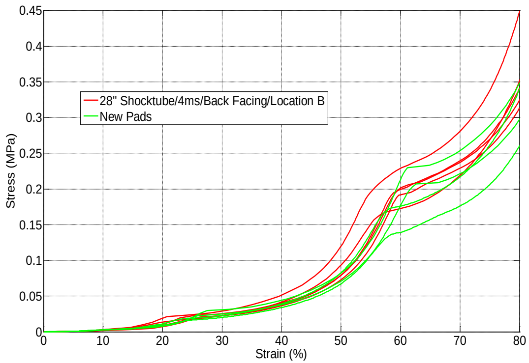
Figure A-10. Trapezoidal-28-inch shocktube/4-ms/back facing/location B vs. new pads.
