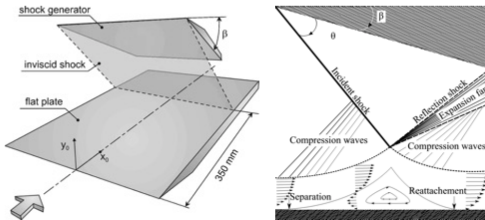
Figure 1: Experimental set-up of Schüle 8 (left) (adapted from Schüle 6 ) and schematics of the flow physics near the SWTBLI region (right)
