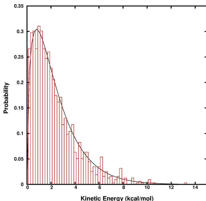
Figure 15 The histogrammed center-of-mass kinetic energy of \text{HO}_2 from the selection of the initial conditions at 800 K shown as red boxes. The analytic distribution for T = 800 K is shown as a solid black line for comparison.
