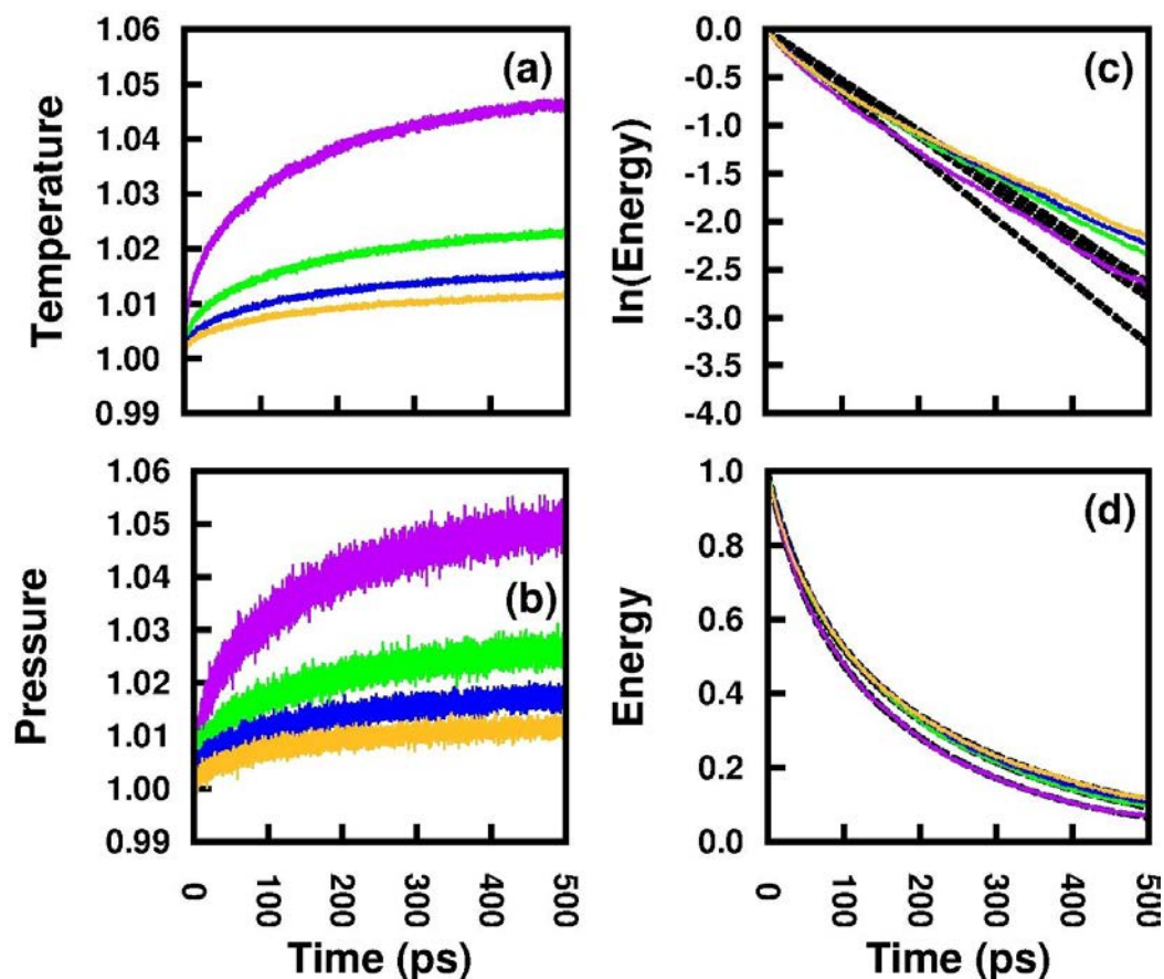
Figure 22. Relaxation results as a function of increasing numbers of Ar bath atoms. (a) Scaled bath gas temperature; 250 Ar, purple curve; 500 Ar, green curve; 750 Ar, blue curve; 1000 Ar, yellow curve. (b) Same as (a), except scaled bath pressure. (c) Vibrational energy decay on semi-log scale with the same coloration as in (a), dashed, black lines correspond to fits to a single exponential function. (d) Vibrational decay with corresponding fits to Eq. 46.
