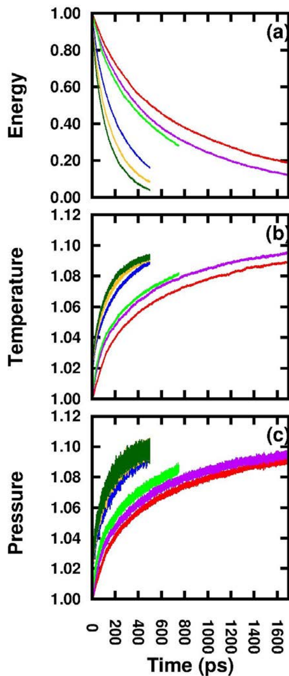
Figure 17 . The results of \text{HO}_2 with 40 kcal/mol of excess internal energy relaxing in a bath of 125 Ar atoms at various pressures. The scaled: (a) vibrational energy, (b) temperature, and (c) pressure. The line coloration: 35 atm, red; 70 atm, magenta; 100 atm, green; 500 atm, blue; 900 atm, yellow; 1300 atm, dark-green.
