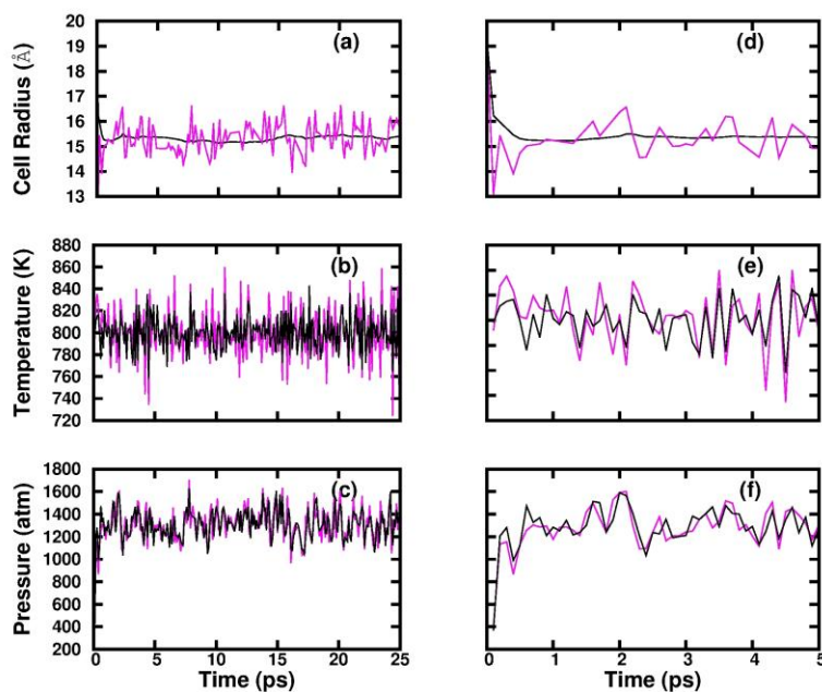
Figure 14 An illustration of the convergence of the cell properties during the pressure equilibration: (a) Cell radius; (b) Bath temperature; (c) Bath pressure. On a shorter timescale: (d) Cell radius (e) Bath temperature; (f) Bath pressure
