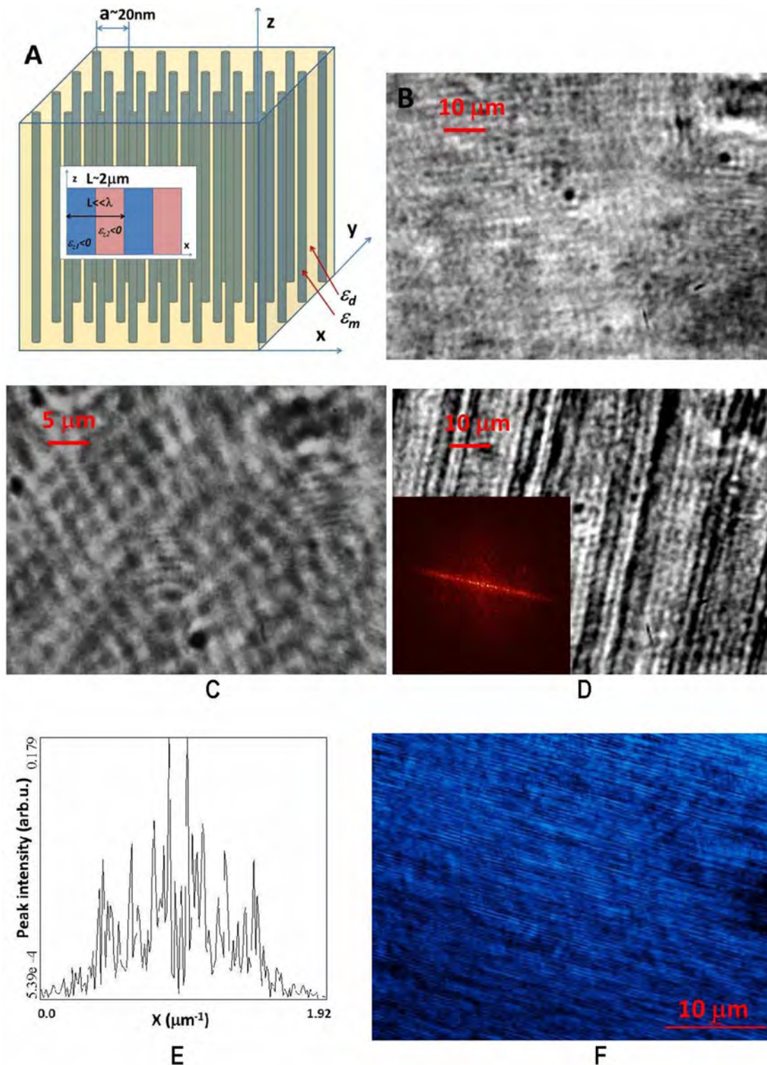
Figure 1 | (A) Experimental geometry of the ferrofluid based hyperbolic metamaterial. The array of self assembled cobalt nanocolumns has typical separation a \sim 20 nm between the nanocolumns. The inset shows a photonic hyper crystal structure formed by periodic arrangement of cobalt rich and cobalt sparse regions with typical periodicity L \sim 2 \mu\text{m} , so that periodic modulation of hyperbolic metamaterial properties on a scale L \ll \lambda is achieved in the LWIR spectral range where \lambda \sim 10 \mu\text{m} . Since photon wave vector in hyperbolic metamaterials is not diffraction limited, periodic modulation of hyperbolic metamaterial properties on a scale L \ll \lambda would lead to Bragg scattering and formation of band structure. (B–F) Microscopic images of cobalt nanoparticle based ferrofluid reveal subwavelength modulation of its spatial properties: frames (B) and (D) show microscopic images of the diluted cobalt nanoparticle based ferrofluid before and after application of external magnetic field. The pattern of self assembled stripes visible in image D is due to phase separation of the ferrofluid into cobalt rich and cobalt poor phases. The stripes are oriented along the direction of magnetic field. The inset shows Fourier transform image of frame D. Its cross section presented in panel E shows a histogram of different periods present in the image. A movie taken during this experiment when the external magnetic field was turned on and off is available in the supporting online material. A microscopic image of the sample taken along the axes of the nanowires is shown in frame C. Panel F demonstrates that the original undiluted ferrofluid exhibits similar phase separation in external magnetic field, even though on much smaller scale.
