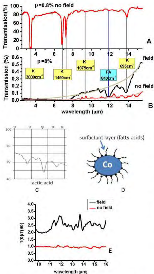
Figure 6 | (A) FTIR transmission spectrum of diluted ( \alpha(\infty) = 0.8\% ) ferrofluid exhibits clear set of kerosene absorption lines. (B) Transmission spectra of the \alpha(\infty) = 8.2\% ferrofluid measured with and without application of external magnetic field. Magnetic field induced transmission spectrum contains a very pronounced absorption line at \lambda \sim 12 \mu\text{m} ( \sim 840 \text{ cm}^{-1} ), which can be attributed to lactic acid. Kerosene absorption lines are marked with yellow boxes, while the fatty acid line at 840 \text{ cm}^{-1} is marked with a green box. (C) The 10 - 14 \mu\text{m} portion of lactic acid FTIR absorption spectrum. (D) Schematic view of cobalt nanoparticle coated with a monolayer of fatty acids, such as lactic and oleic acid. (E) Extinction coefficient (the ratio T(0)/T(90) ) of ferrofluid transmissions at 0 and 90 degrees of ferrofluid subjected to external magnetic field exhibits pronounced resonances around the fatty acid absorption line at \lambda \sim 12 \mu\text{m} and the kerosene absorption line at \lambda \sim 14 \mu\text{m} . These resonances provide clear evidence of field enhancement by cobalt nanoparticle chains.
