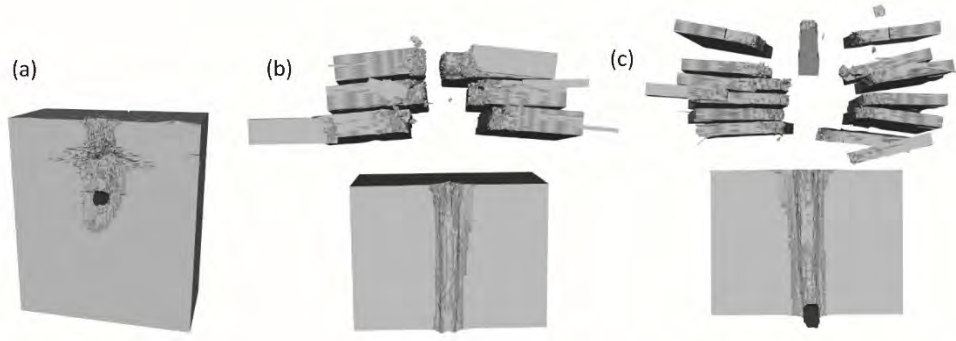
Fig. 3 Penetration simulations into ceramic-metal targets: a) one tile, tied bonding, impact velocity 1,030 m/s, b) 3 tiles, free bonding, with polymer, impact velocity 1,100 m/s, and c) 6 tiles, free bonding, without polymer, impact velocity 1,160 m/s
