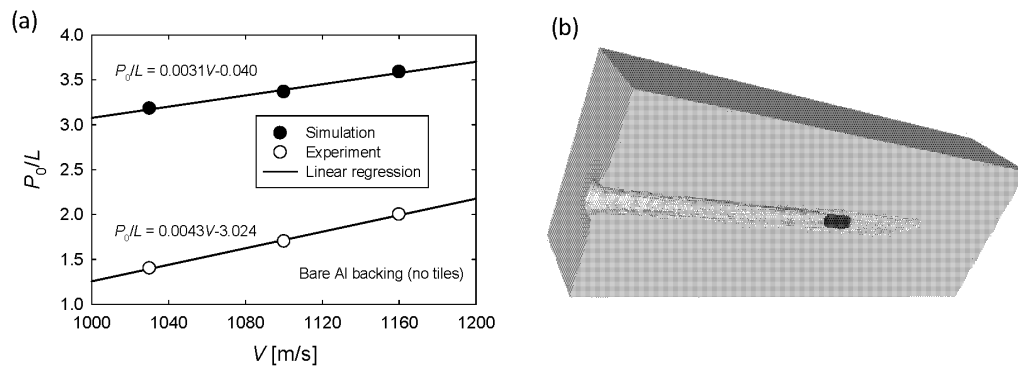
Fig. 2 Penetration into bare aluminum backing material: a) depth vs. impact velocity for simulation and experiment 1 and b) simulation result at impact velocity of 1,030 m/s
