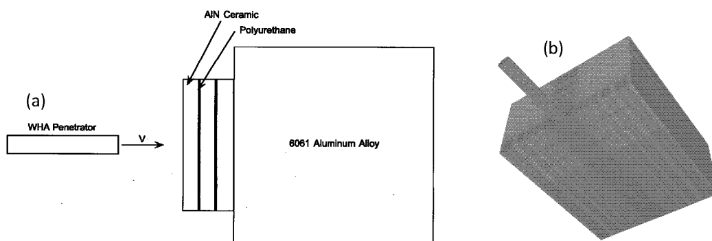
Fig. 1 Ballistic impact problem: a) projectile and target (3 tiles) and b) finite element mesh
