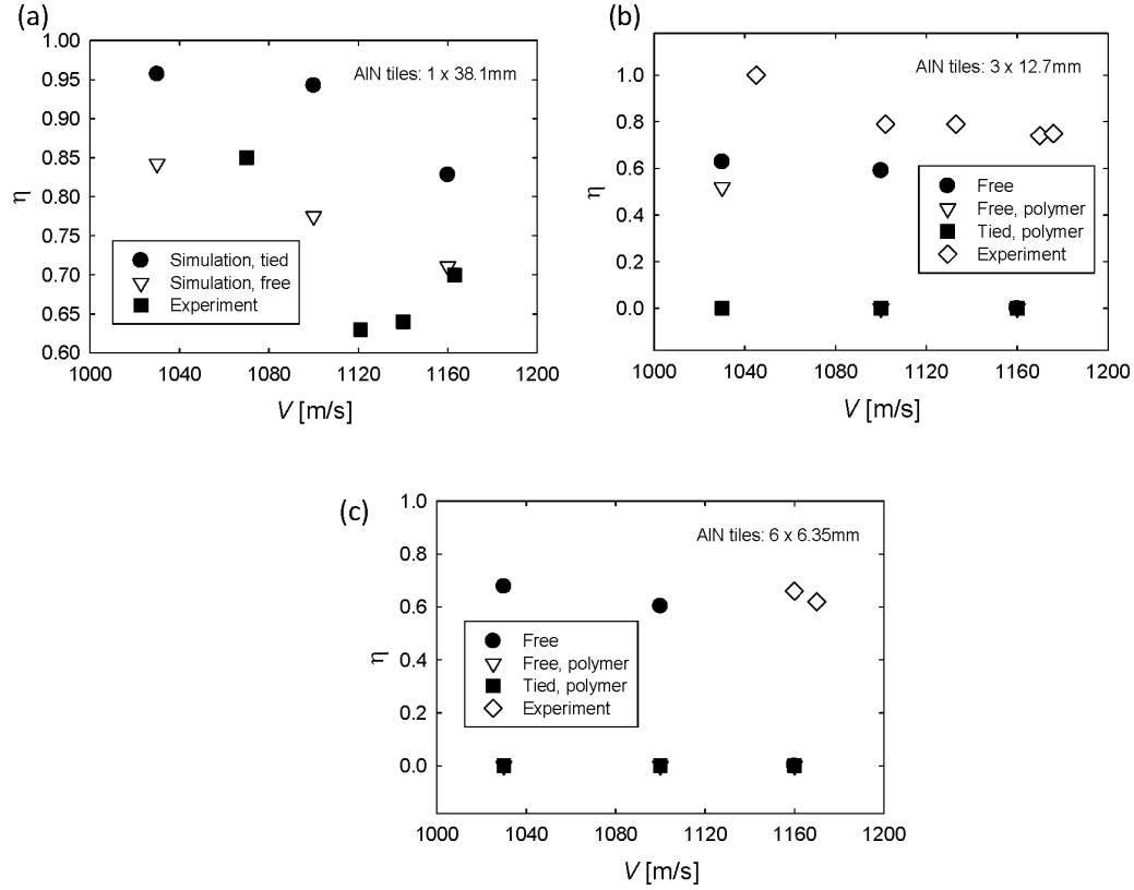
Fig. 4 Ballistic efficiency vs. impact velocity for ceramic-metal targets from simulations and experiments 1 : a) 1 tile, b) 3 tiles, and c) 6 tiles
