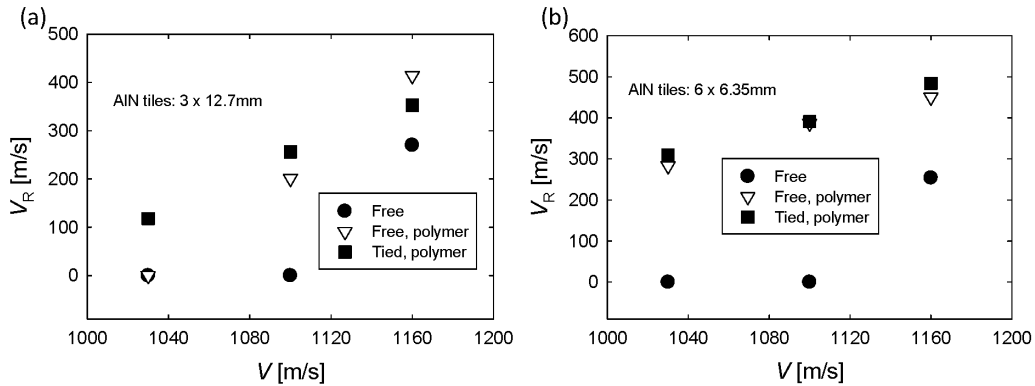
Fig. 5 Residual penetrator velocity vs. impact velocity from simulations: a) 3 tiles and b) 6 tiles
