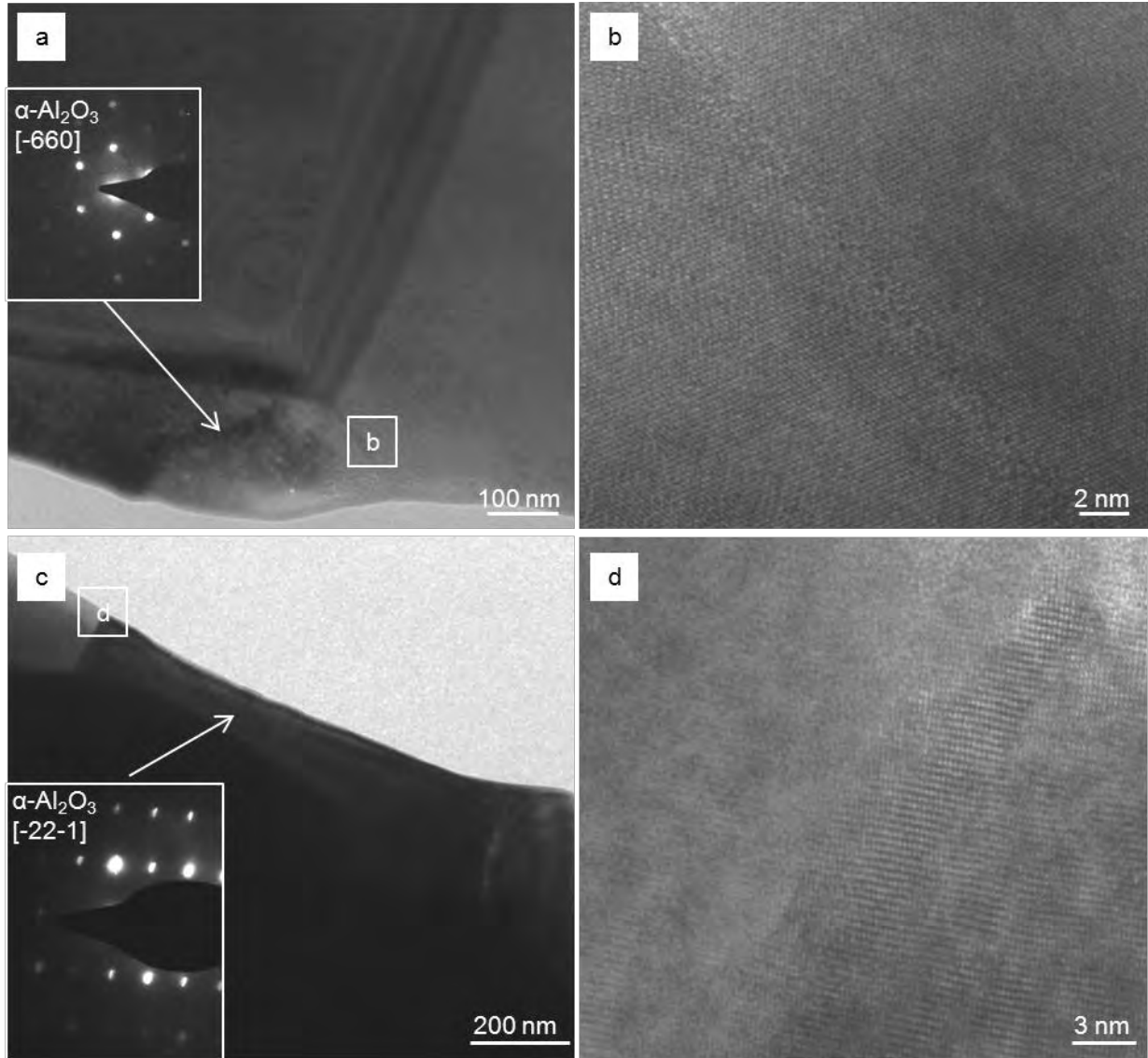
Figure 53: TEM images of the AO-H sample showing clean grain boundaries in the \text{Al}_2\text{O}_3 matrix.
