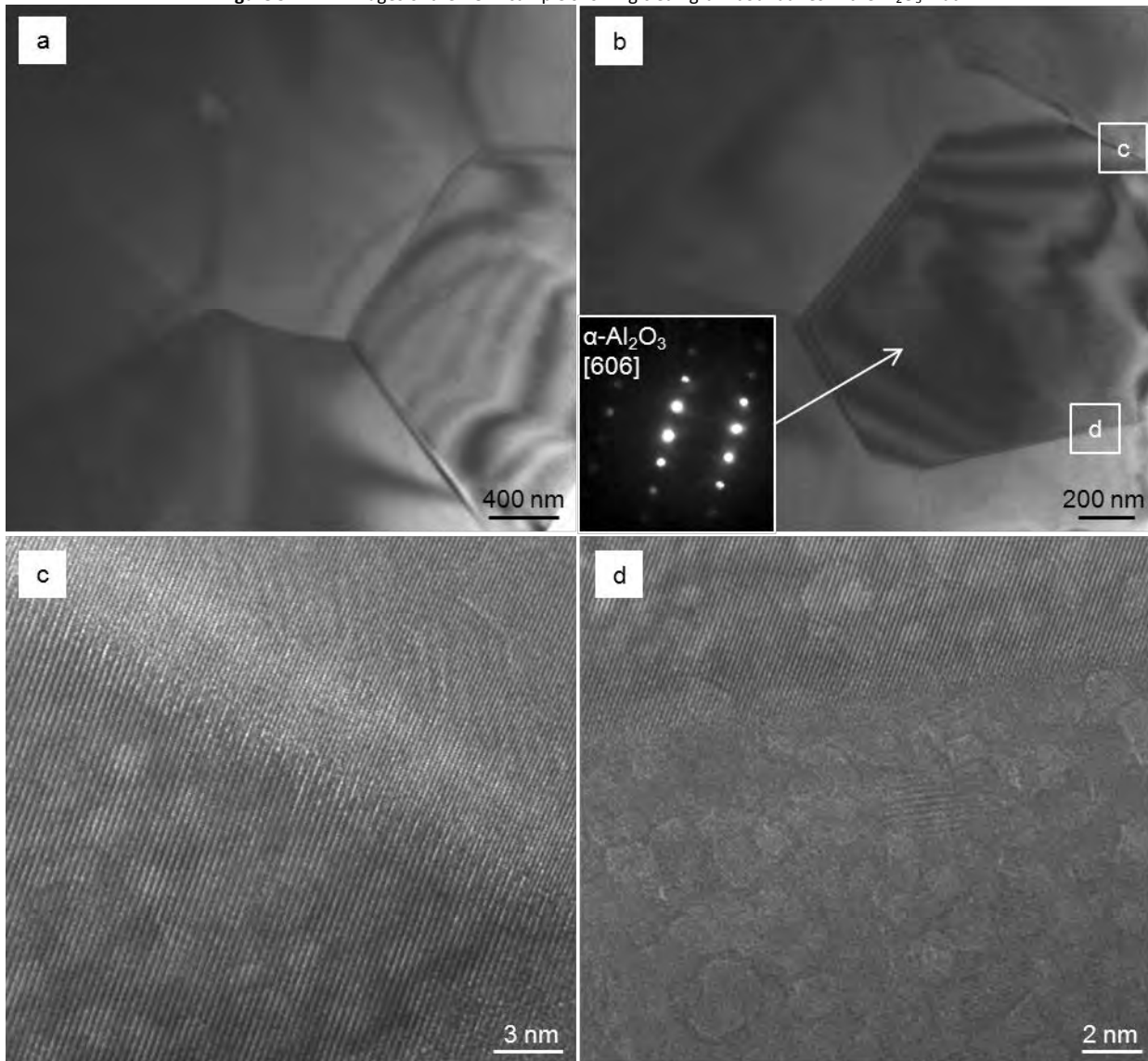
Figure 52: TEM images of the AO-H sample showing clean grain boundaries in the Al 2 O 3 matrix.
