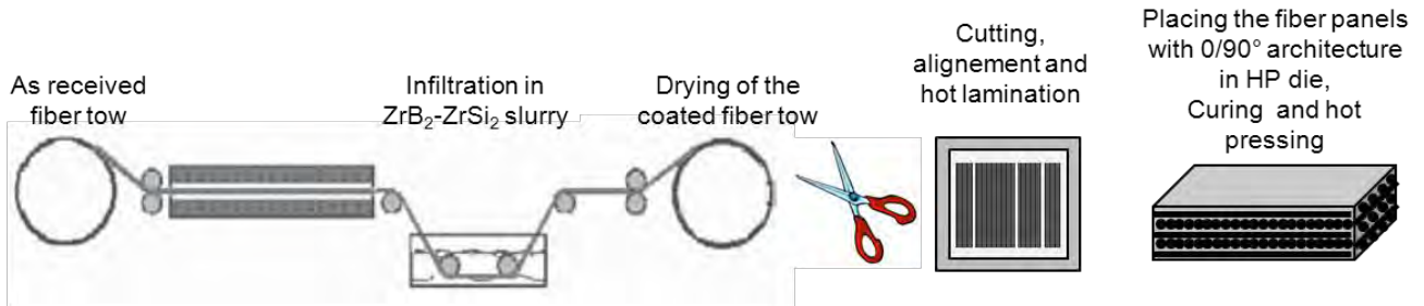
Figure 17: Sketch of the experimental procedure for the fabrication of 0/90° long-fiber ZrB 2 composite.
