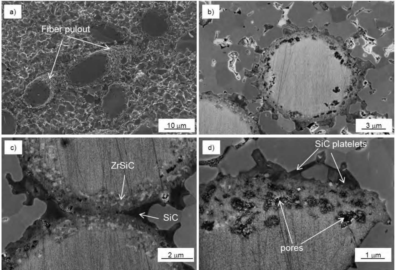
Figure 10: a) Fracture surface and b)-d) polished surfaces of ZrB_2 composite containing Hi-Nicalon S fiber and Si_3N_4 as sintering additive. b) Overview of a fiber section, c) magnification of fiber-matrix interface and d) reaction products trapped inside the fiber
