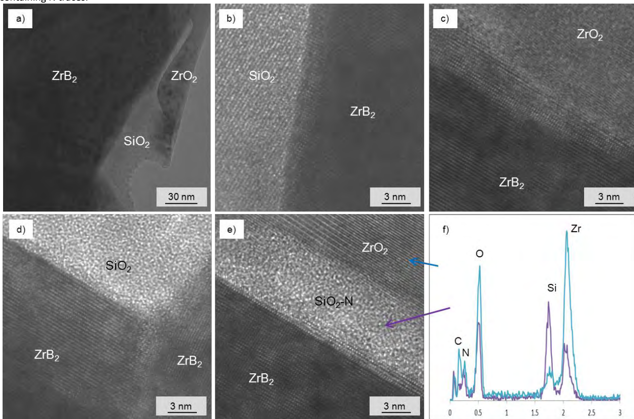
Figure 19: Examples of HR-TEM images of the matrix in ZBZ-iH* showing the interfaces between ZrB_2 - SiO_2 - ZrO_2 with EDS spectra of SiO_2 and ZrO_2 containing N traces.
