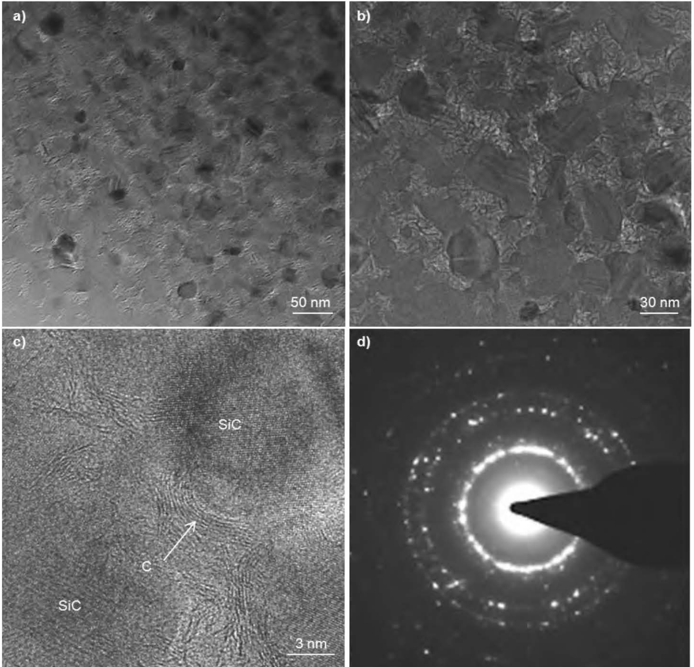
Figure 35: TEM images of fiber core with diffraction pattern showing the presence of amorphous phase and turbostratic carbon.
