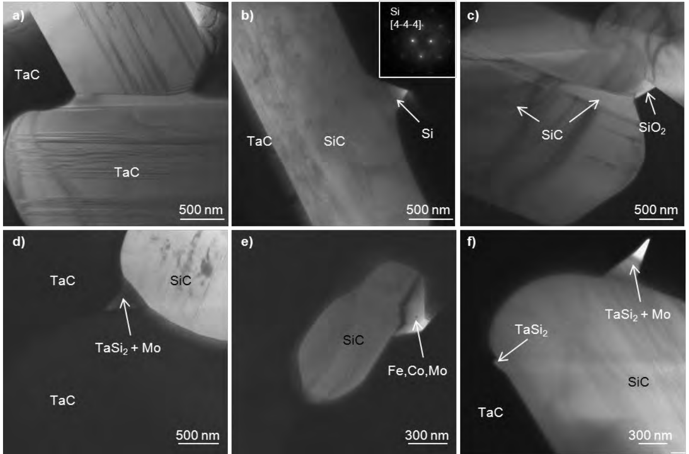
Figure 29: TEM images of TM-S showing adjacent SiC platelets and secondary phases at the triple junctions.
