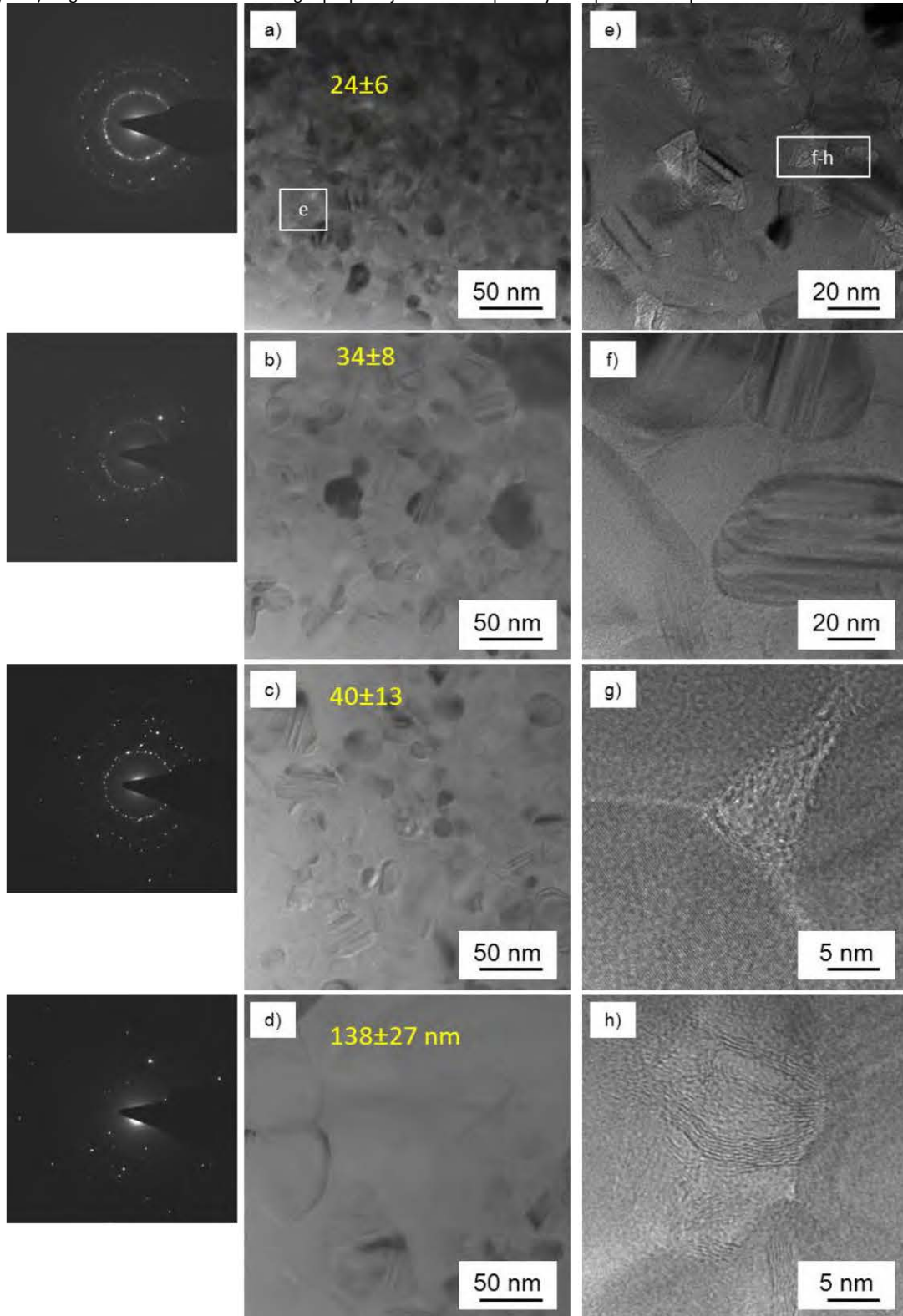
Figure 14: a)-d) Microstructure of a SiC fiber in ZBS-HS moving from the core outwards with corresponding diffraction patterns showing improved crystallinity. e-h) magnification of fiber core showing triple point junctions and partially amorphous C-rich phase.
