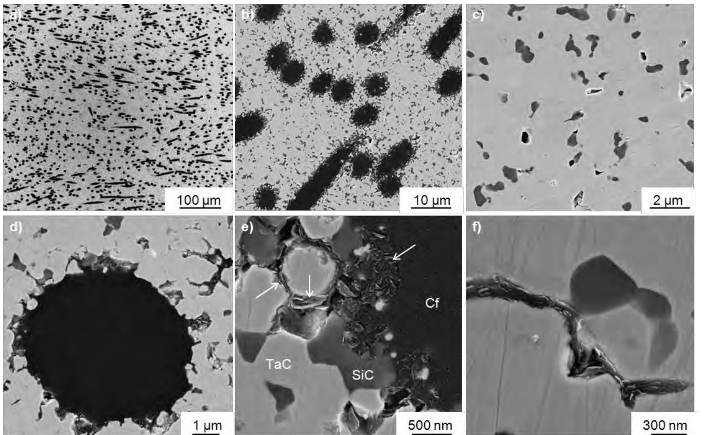
Figure 41: SEM images of polished section of TS-C showing a) the fiber distribution, b) the overall microstructure, c) scattered SiC in the matrix, d) a fiber section, e) a magnification of the fiber/matrix interface with arrows indicating graphite flakes and f) graphite sheets throughout TaC grains.
