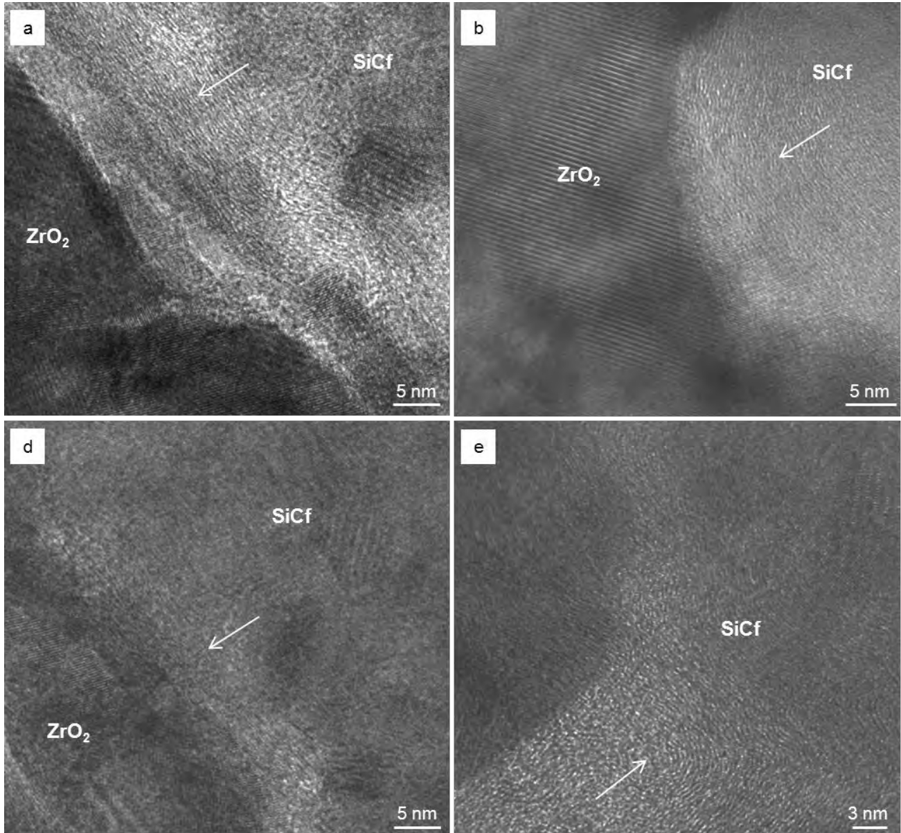
Figure 60: HR-TEM images of the fiber/matrix interface in ZO-H sample showing the presence of turbostratic carbon indicated by arrows.
