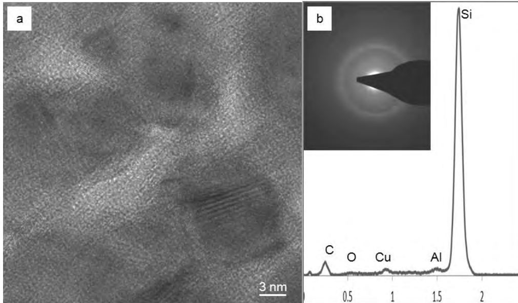
Figure 55: a) HR-TEM image of a SiC fiber in the AO-H sample with EDS spectrum and diffraction pattern in b).
