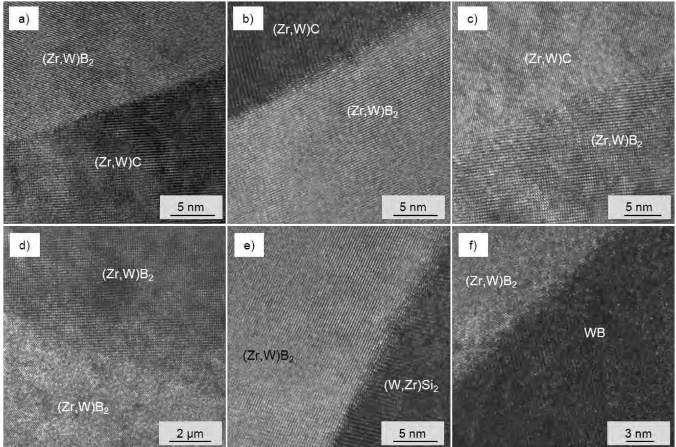
Figure 7: HR-TEM images showing clean grain boundaries between (\text{Zr,W})\text{B}_2 , (\text{Zr,W})\text{C} , (\text{W,Zr})\text{Si}_2 and WB.
