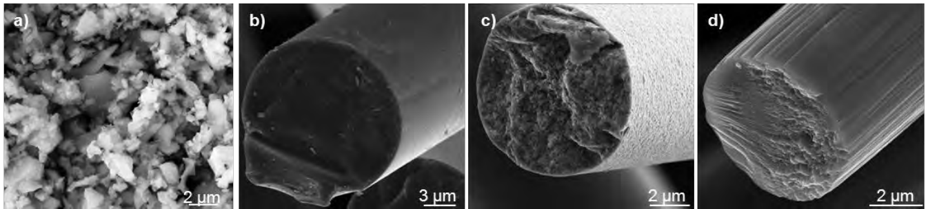
Figure 26: SEM image of reinforcing phases: a) SiC particles, b) Hi-Nicalon, c) Tyranno SA3, d) C fiber.
