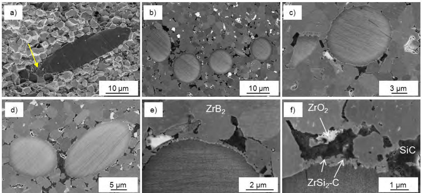
Figure 16: a) Fracture surface and b)-f) polished surfaces of ZrB_2 composite containing Hi-Nicalon S fiber and ZrSi_2 as sintering additive. b) Overview of the material microstructure, c) magnification of a fiber section, d) formation of SiC between two fibers, e) fiber-matrix interface and f) reaction products at the fiber edge.
