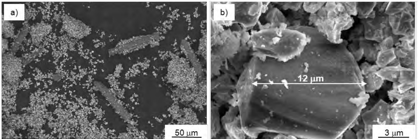
Figure 9: a) Low and b) high magnification of Hi-Nicalon S fiber after in house chopping and mixing with ZrB_2 powder.
