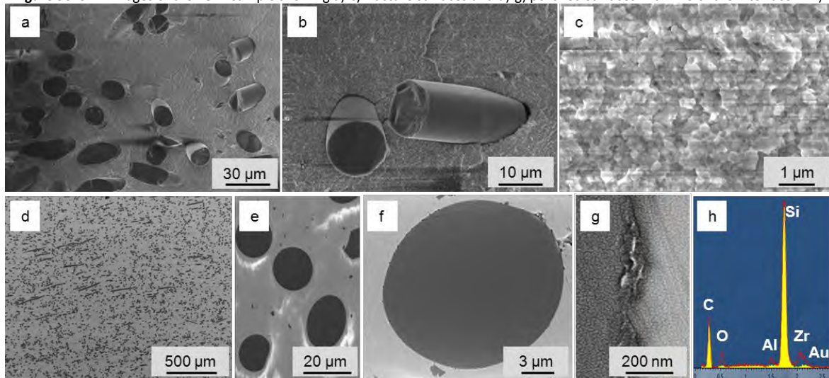
Figure 56: SEM images of the ZO-H sample showing a)-c) fracture surfaces and d)-g) polished surfaces with EDS of the interface in h).
