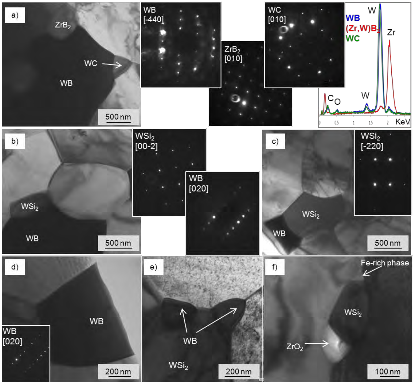
Figure 5: TEM images of the secondary phases with EDX spectra and diffraction patterns showing the presence of WB, WC, \text{WSi}_2 and residual \text{ZrO}_2 .
