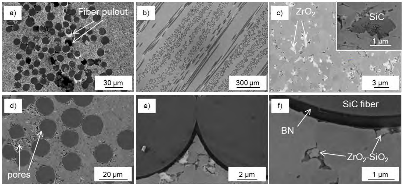
Figure 18: a) Fracture surface and b)-f) polished surfaces of ZrB 2 composite containing long BN-coated Hi-Nicalon fiber and ZrSi 2 as sintering additive. b) Overview of the material architecture, c) magnification of the matrix showing ZrO 2 and SiC aggregates, d) fiber distribution with trapped porosity, e) homogeneous BN coating around the fibers and f) efficient blockage of secondary phases at the coating interface.
