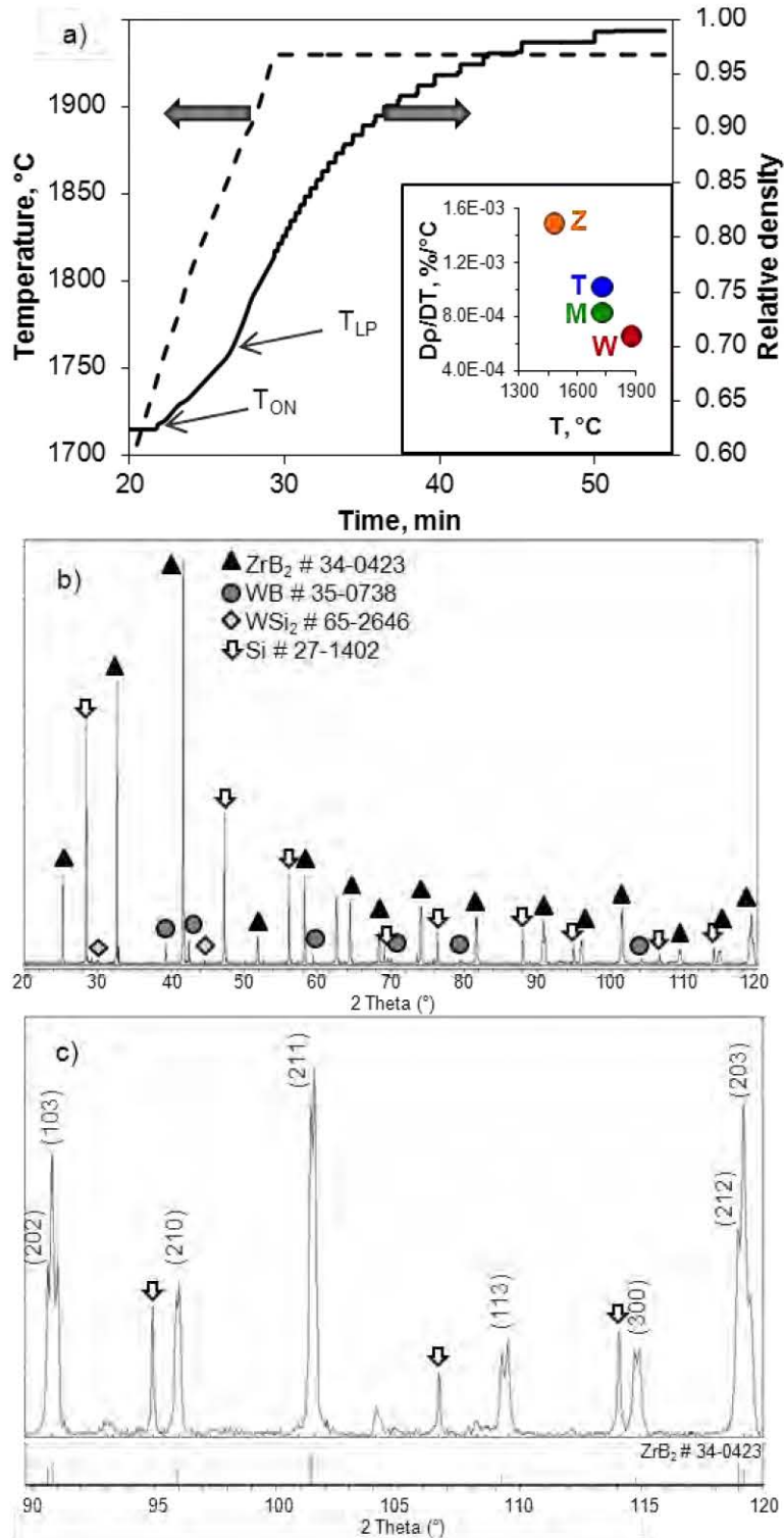
Figure 2: a) Densification curve recorded during hot pressing. T_{ON} : temperature at which shrinkage begins, T_{LP} : temperature at which liquid phase forms. In the inset: plot of the maximum densification rate as a function of the temperature for different silicides; Z: ZrSi_2 , T: TaSi_2 , M: MoSi_2 , W: WSi_2 . b) X-ray diffraction pattern of the sintered composite showing the crystalline phases and c) ZrB_2 peaks splitting at high 2-Theta angles.
