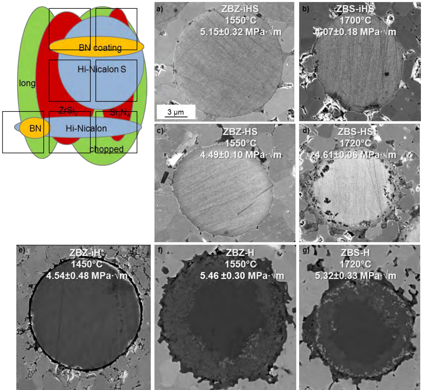
Figure 24: Examples of fiber section in various ZrB 2 -based composites sintered with ZrSi 2 or Si 3 N 4 as additive and containing Hi-Nicalon or Hi-Nicalon S, naked or BN-coated, long or short fiber, like indicated in the sketch on the left. For each composite, the sintering temperature and the fracture toughness are reported.
