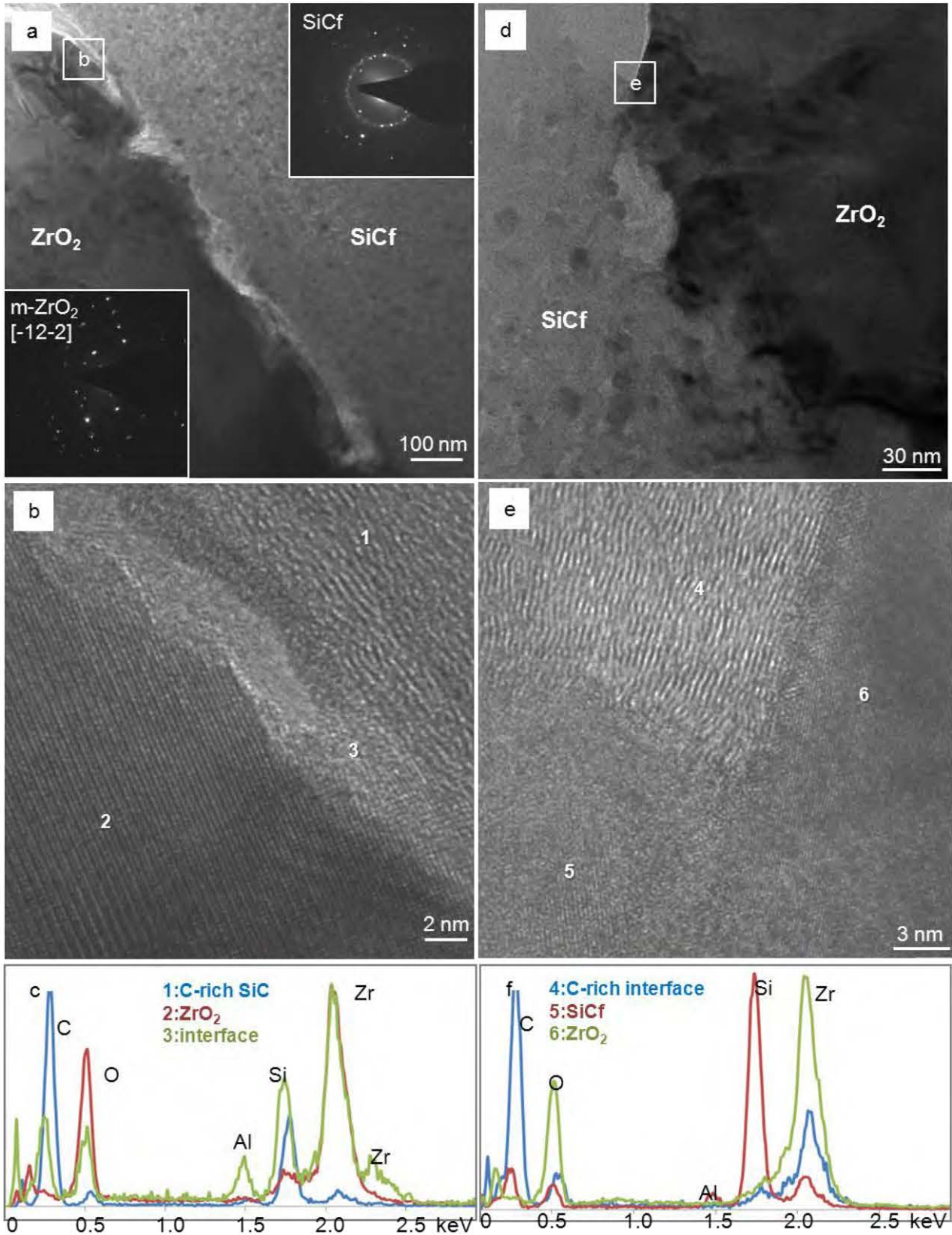
Figure 59: TEM images of the fiber/Matrix interface in ZO-H sample with HR-images and EDS spectra as indicated.
