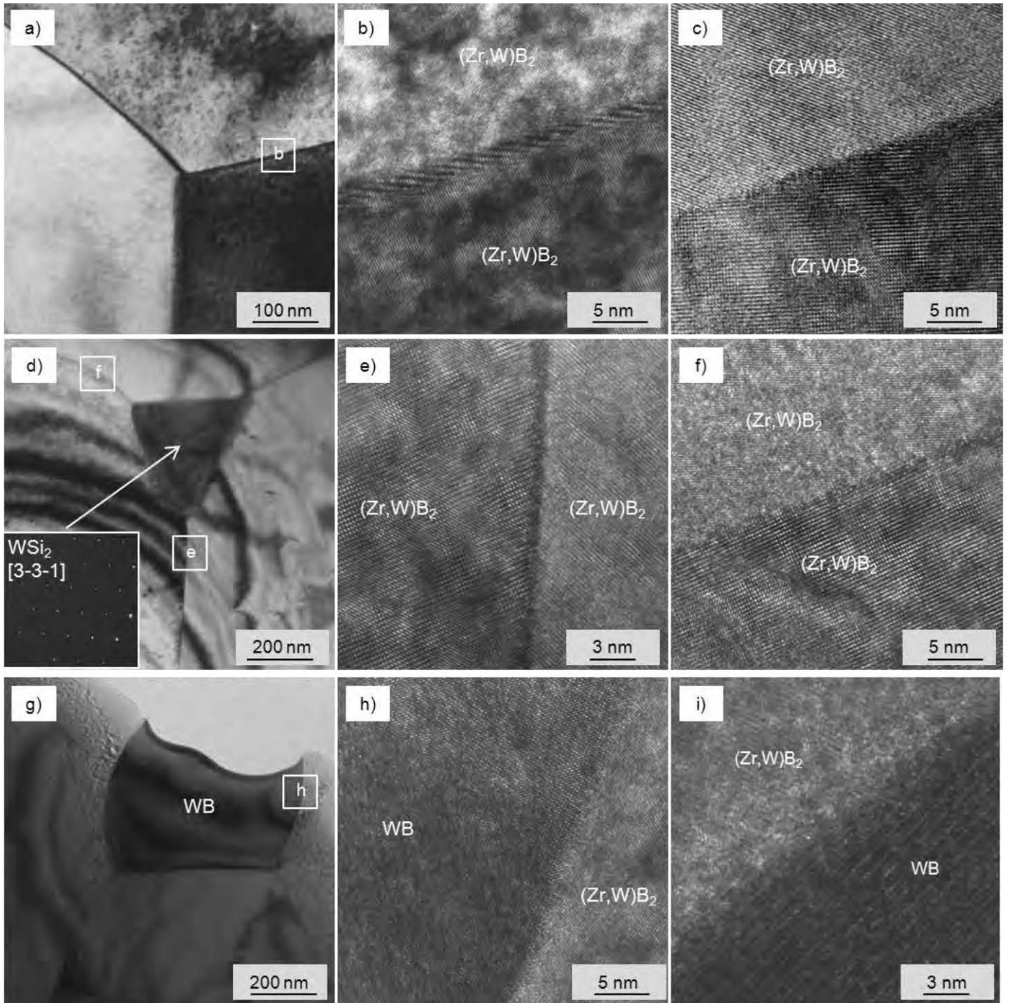
Figure 6: TEM and HRTEM images of the triple point junctions showing clean grain boundaries between a-f) adjacent (\text{Zr,W})\text{B}_2 grains and g-i) between WB and (\text{Zr,W})\text{B}_2 .
