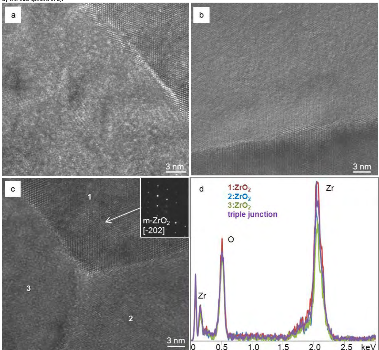
Figure 57: HR-TEM images of the ZO-H sample showing a)-b) clean grain boundaries and c) a triple point junction free of other phases, as confirmed by the EDS spectra in d).
