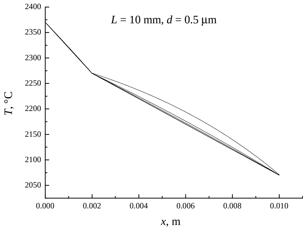
Fig. 8. Temperature distribution at d = 0.5 \mu\text{m} , L = 10 \text{ mm} . Pulling velocities 1 \mu\text{m/s} , 0.01 \text{ mm/s} , 0.1 \text{ mm/s} , 0.25 \text{ mm/s} , 1 \text{ mm/s} .
