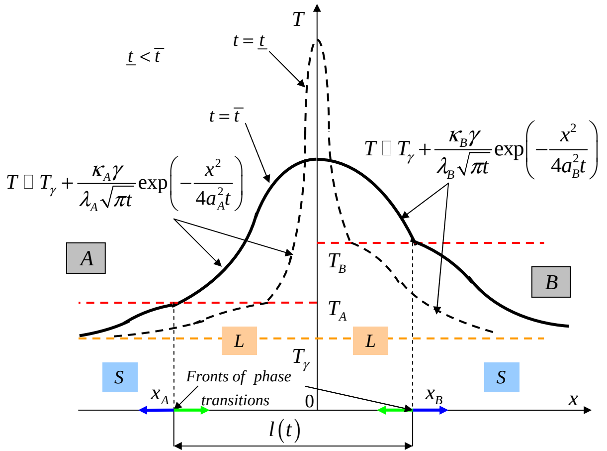
Fig. 16. Schematic graph of themperature distribution in the neighbourhood of flat boundary x=0 of initial separation of phases A and B , x_A(0) = x_B(0) = 0 ;
