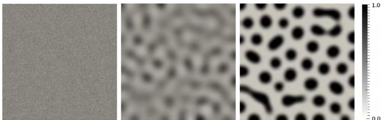
Fig.25. The results of 2D-simulations (composition distribution) of the formation of eutectic structure in \text{LaB}_6 - \text{ZrB}_2 from glass at the temperature T = 2000^\circ\text{K} for the time points t=0 ; 60; 180 sec (from the left to the right).
