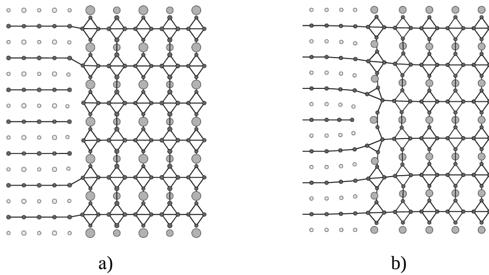
Fig. 59. Semicohherent interface: a) before relaxation of atomic positions; b) after relaxation. Atoms La – large gray circles, Zr – small gray circles, B – black circles.
