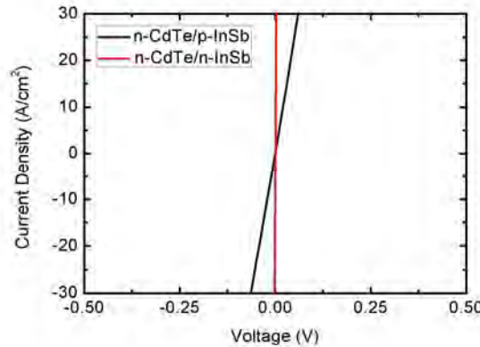
Figure 8 Current-voltage characteristics of n-CdTe/n-InSb and n-CdTe/p-InSb vertical transport samples show linear behaviors with small resistivity below 0.1 \Omega \cdot \text{cm}^2 indicating negligible voltage drop across interfaces.
