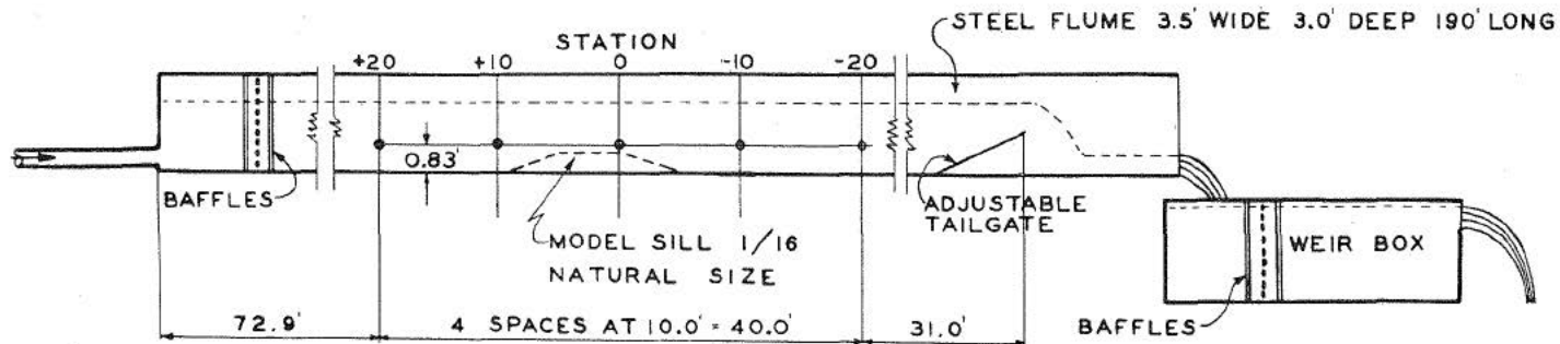
LAYOUT OF APPARATUS FOR FLUME TESTS
