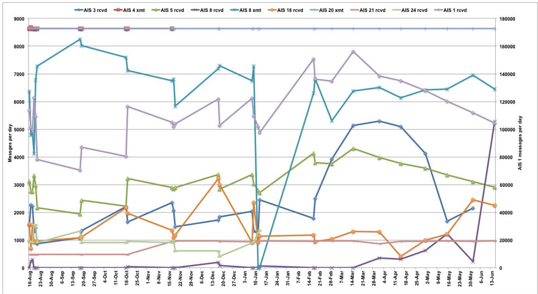
Figure 8. Sample statistics.
