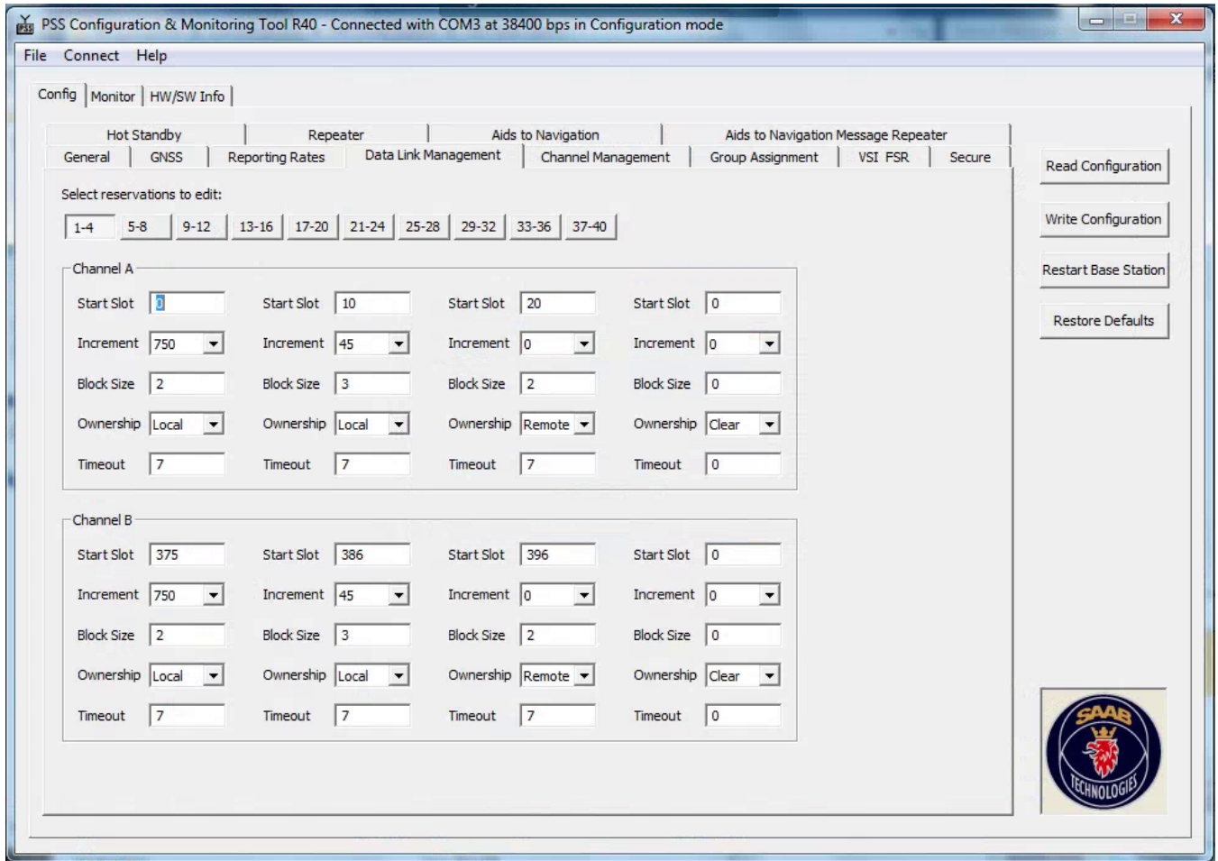
Figure 2. Louisville base station slot reservations.
