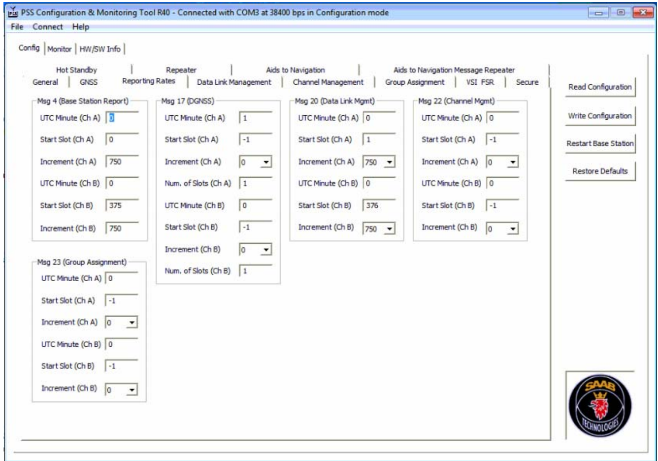
Figure 3. Louisville base station scheduled messages.
