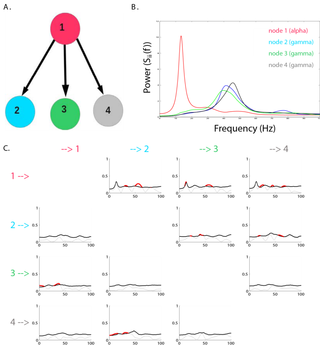
Fig. 5 Alpha node 1 driving 3 gamma nodes. A: connectivity structure of a simulated network. B: The power spectrum (0–100 Hz) computed from the MVAR model. C: computed DTF values plotted against frequency (0–100 Hz), where the rows correspond to the sending nodes and the columns correspond to the receiving nodes. In each DTF plot, the red curves above the black lines correspond to frequency values with DTF values statistically significant.
