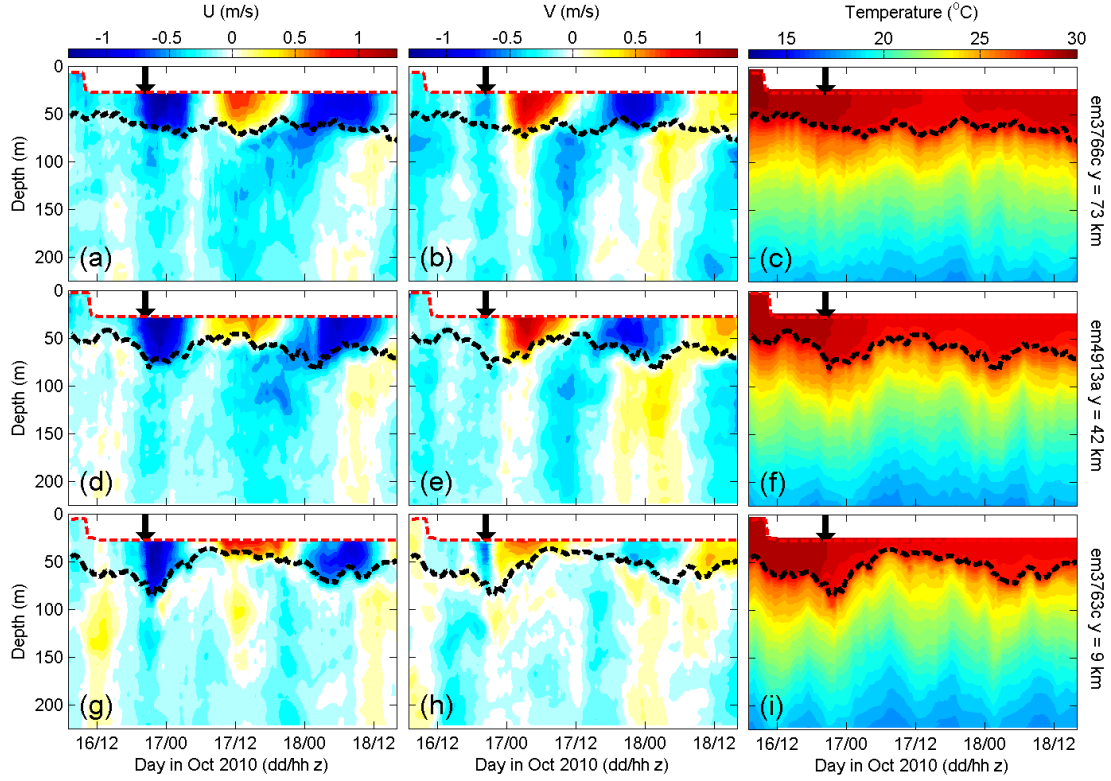
Fig. 2. Contour plots of current velocity and temperature measured by three EM-APEX floats in October 2010. (a), (d), (g) Zonal current velocity ( \text{m s}^{-1} ). (b), (e), (h) Meridional current velocity ( \text{m s}^{-1} ). (c), (f), (i) Ocean temperature ( ^{\circ}\text{C} ). The x axis is the day (dd/hh) in UTC. Label to the right of each row is the cross-track distance (km) for each float, positive to the right hand side of the storm track (mostly to the north because Typhoon Megi's motion is westward). The dashed red lines mark the shallowest depth of float measurements. The black arrows indicate the arrival time of Typhoon Megi at the float array, about 2030 UTC on 16 October. The black dash lines are the mixed layer depth.
