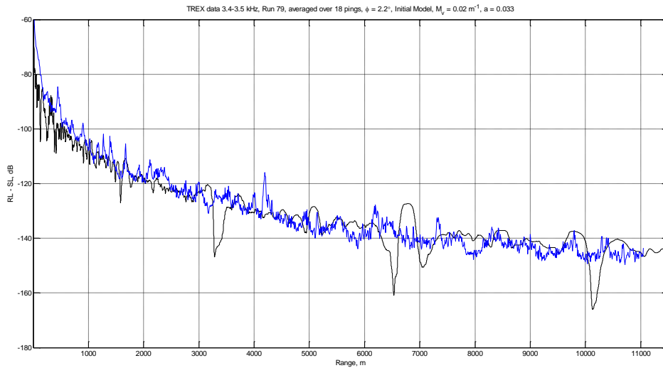
Figure 17: TREX13 normalized reverberation intensity, RL-SL , at 3.4-3.5 kHz, measured after storm (blue), compared to that calculated for volume scattering from sand bottom (range-independent, ) with M_V = 0.02 \text{ m}^{-1} .
