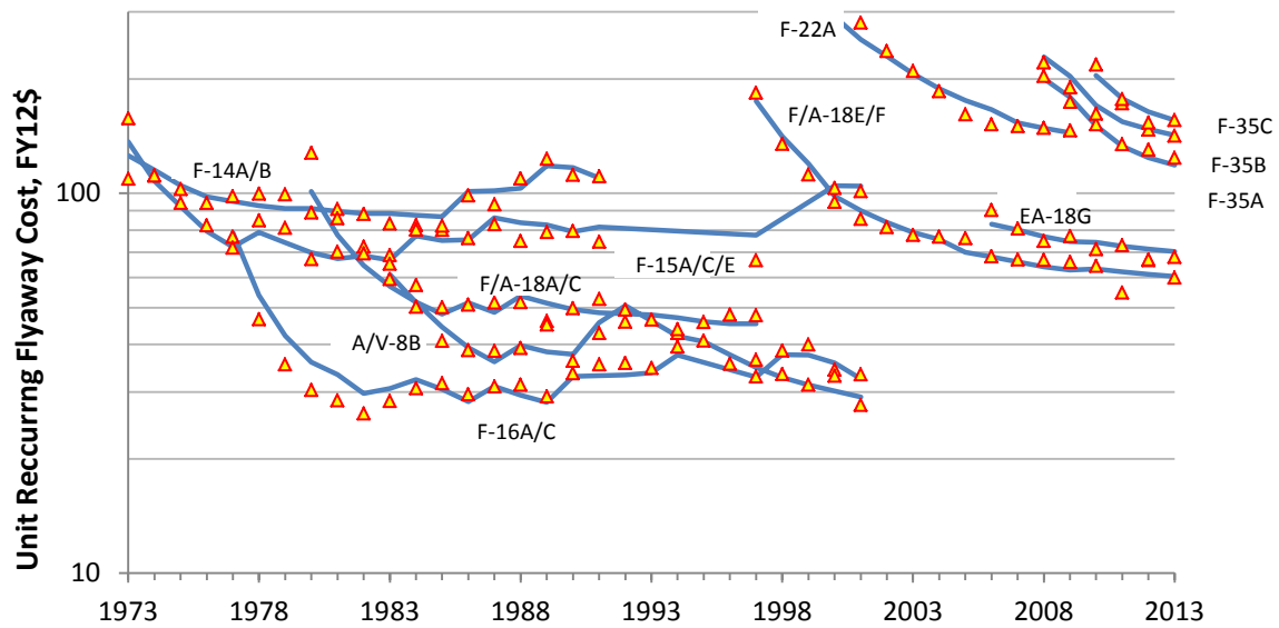
Figure 3. Fit of the Full CER Model to the Data
