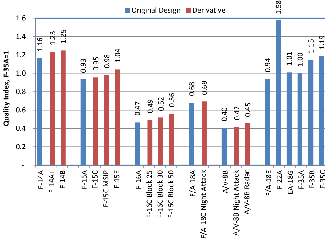
Figure 4. Estimated Quality Index for Tactical Aircraft (F-35A=1): Full CER Model Estimates
