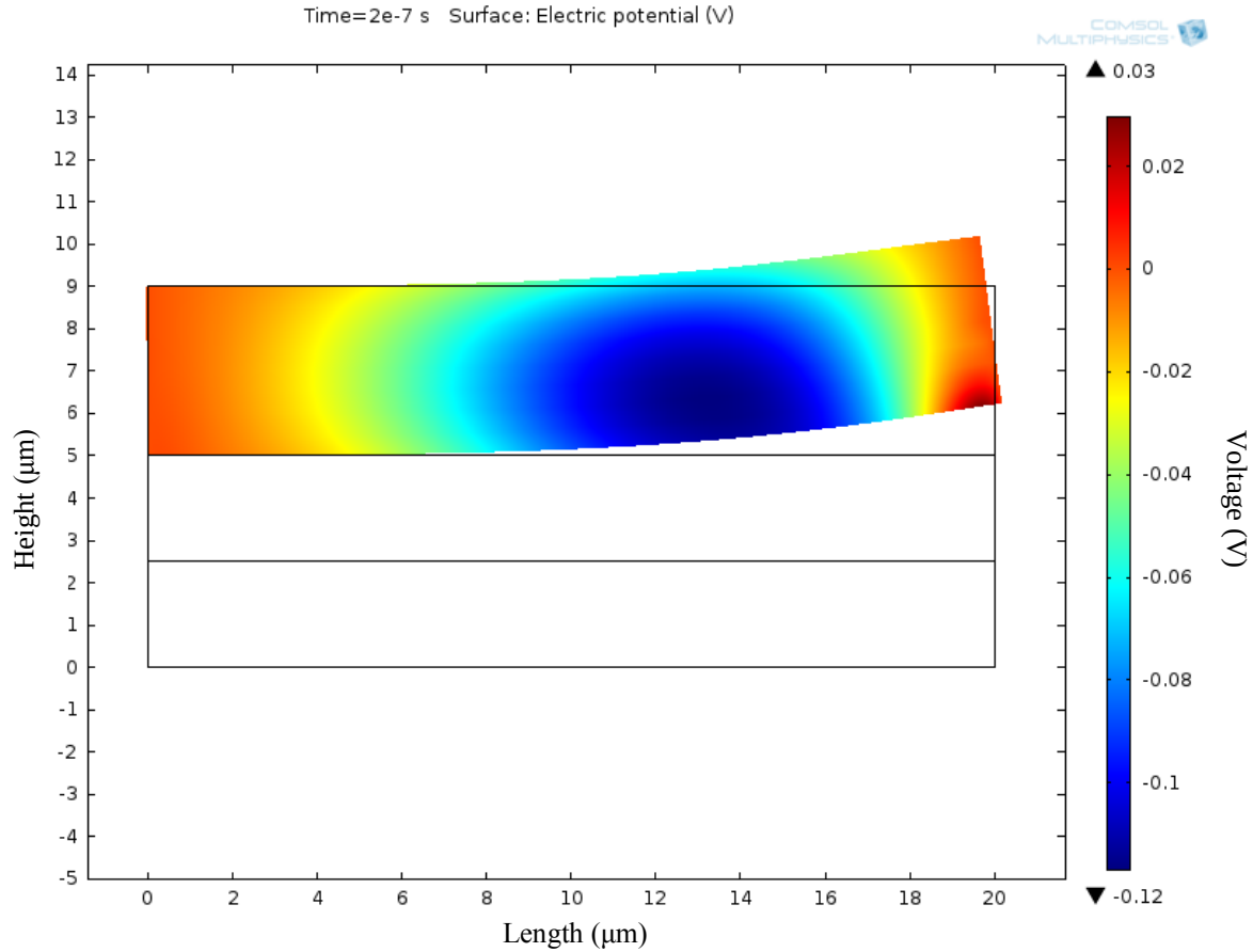
Figure 15. Stressed piezoelectric material (deformation scale 500; bimetal layer not shown)
