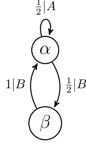
Figure 16: Representation of even process
