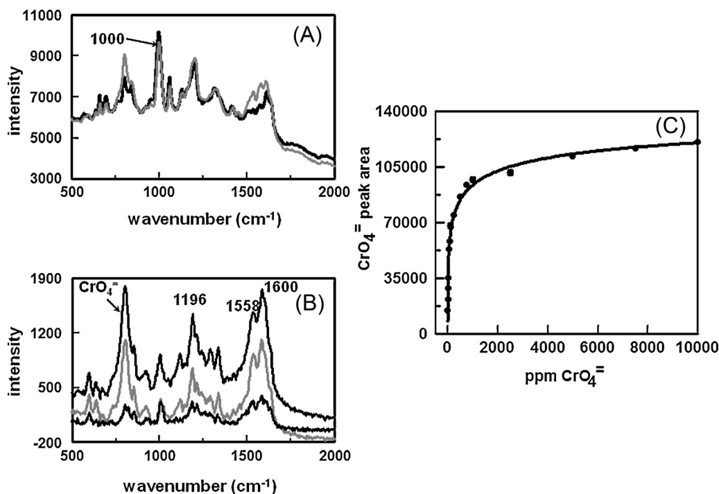
Fig. 3. (a) SERS spectra of a conventional Au/MEP SERS substrate obtained at chromate concentrations of 0 (black) and 2500 (gray) ppm. Spectra were obtained using 785 nm excitation at 30 mW and averaging ten 2 s spectra. (b) Difference spectra obtained by subtracting the 0 ppm spectrum from the 1 (bottom), 100 (middle), and 500 (top) ppm chromate Au/MEP spectra. The chromate peak is indicated. (c) Plot of chromate peak area as a function of chromate concentration. Equation describing the curve is summarized in Table 1.
