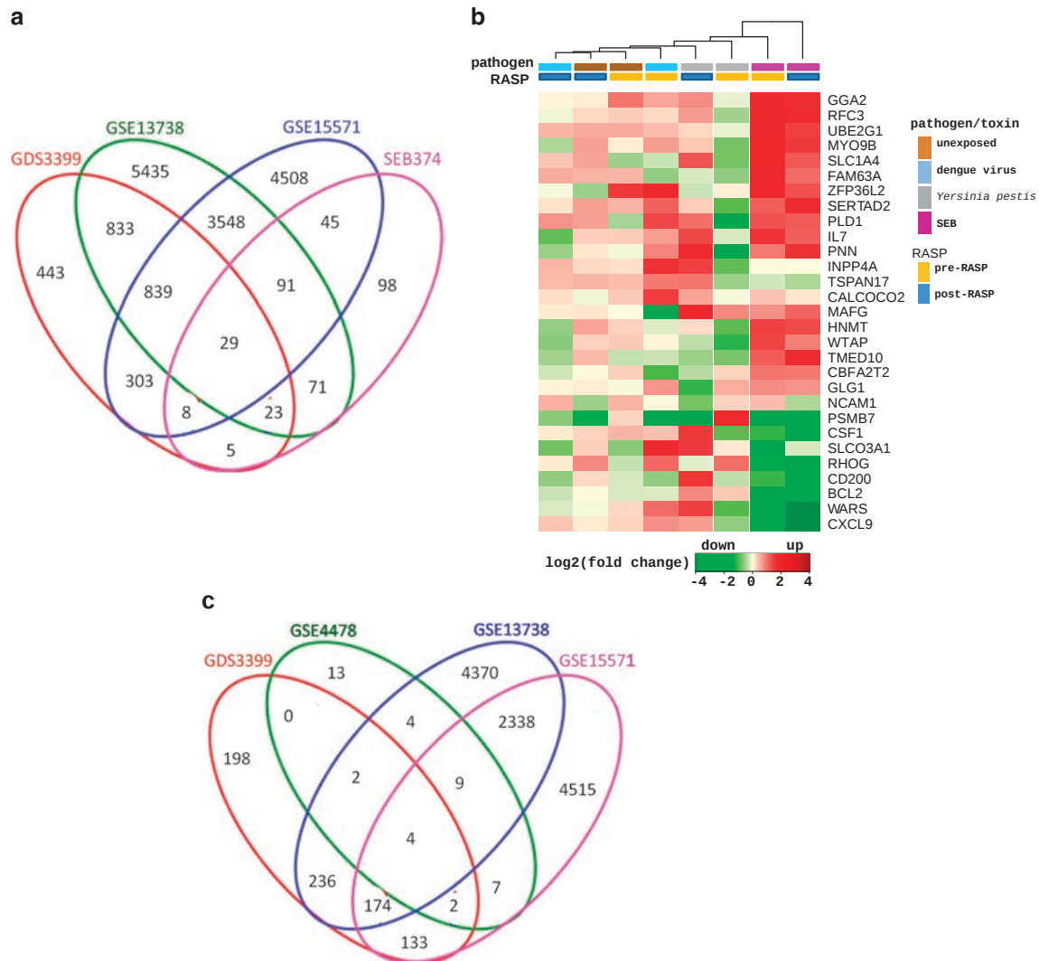
Figure 9. (a) The 29 common probes among three GEO data sets ('GDS3399', 'GSE13738', and 'GSE15571') and 374 SEB-specific probes. (b) The 29 probes that are specific to SEB (both in the pre- and post-RASP SEB exposures). (c) The four common probes of the four GEO data sets using stringently filtered lists of differentially expressed transcripts. CXCL9 is common to both groups of the common probes.
