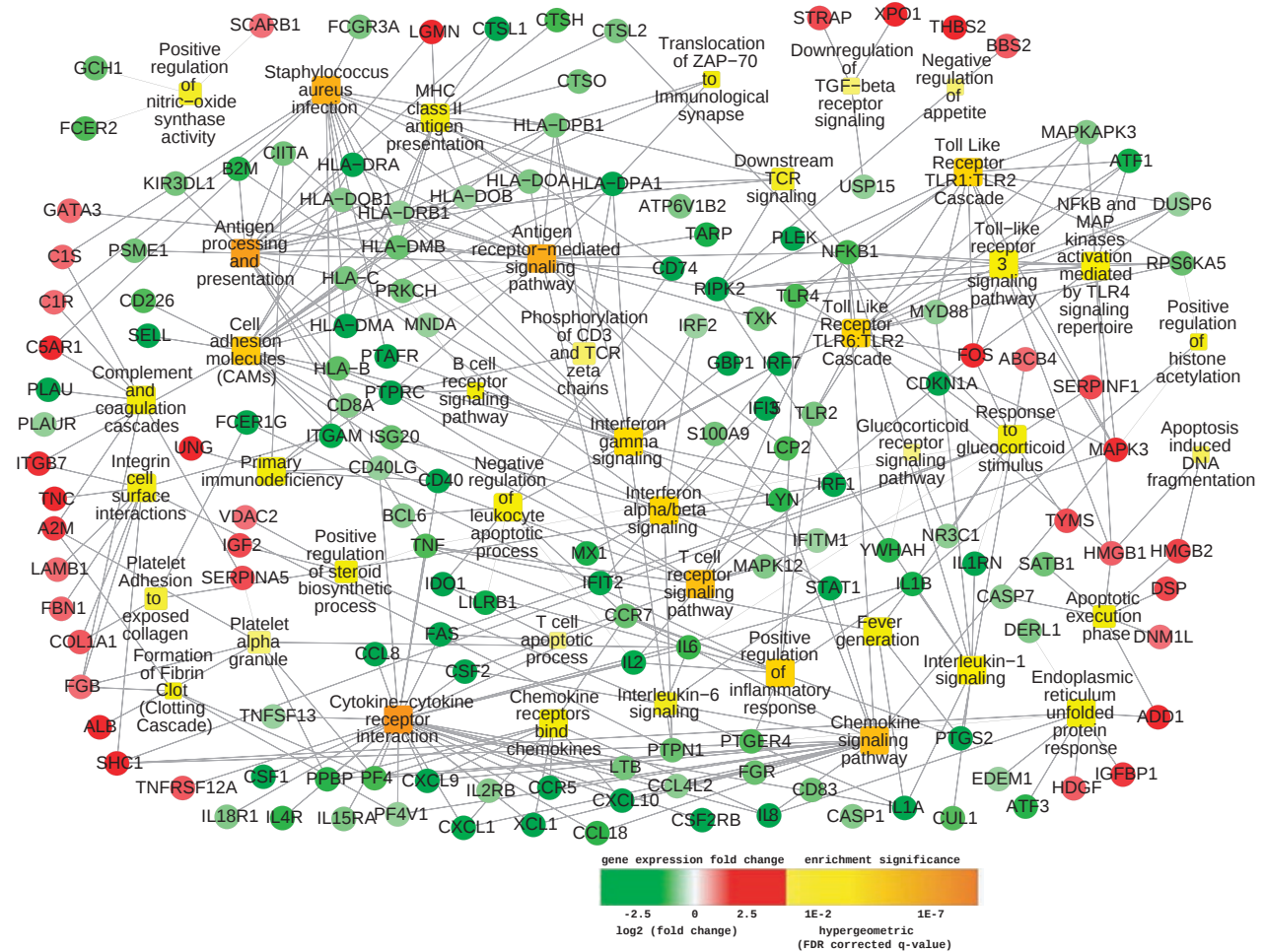
Figure 2. Functional interaction networks of pathways and biological processes significantly associated with the 460 post-RASP SEB response transcripts. Striking changes in downregulated transcripts related to inflammation, chemotaxis, antigen presentation and T-cell receptor signaling. Growth factors such as insulin like growth factors were upregulated among SEB-regulated transcripts. IGFs and their receptors are shown to suppress inflammatory responses. 17 Note: yellow square nodes represent pathways and processes; red and green round nodes represent transcripts.
