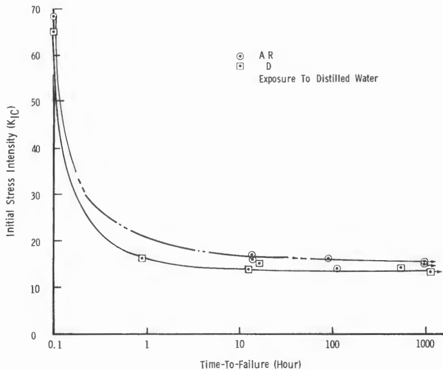
Figure 6. K_{IC} - time-to-break curves.
