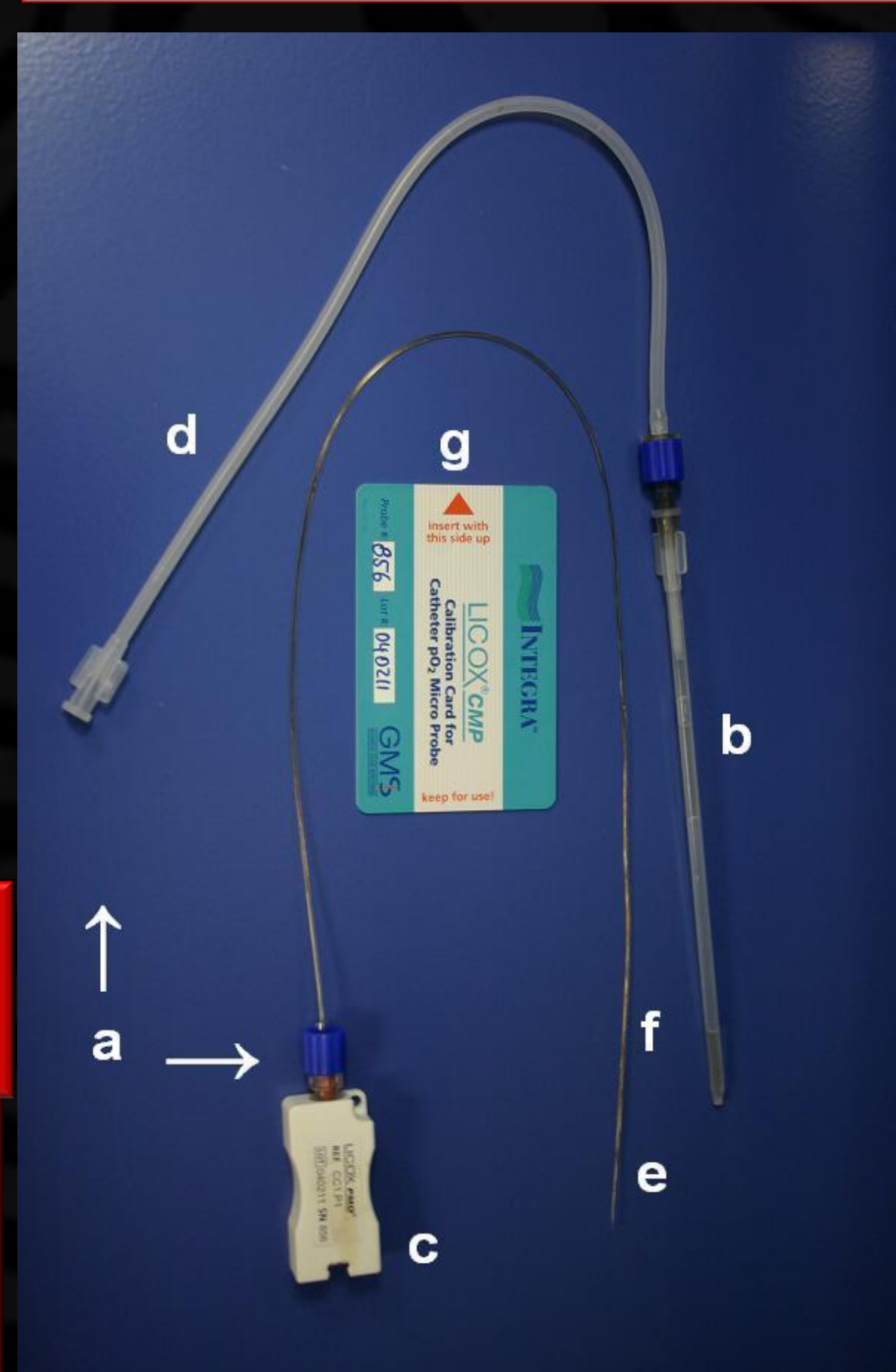
Fig. 1. The probe (Licox Combined Oxygen and Temperature Probe CC1.P1, Integra, Plainsboro, NJ) is a Clark type polarographic oxygen probe (e) and temperature measurement (f) device and comes packaged as shown: (a) probe enters the extension tube (d) and plastic closed humid chamber over the tip (b). The plastic cover (b) is removed for insertion. The probe is connected to the monitor via a cable at (c). A smart card with calibration data specific to each probe is inserted into the monitor. Letter (e) shows the oxygen sensitive area and (f) shows the temperature sensitive area of the probe.
