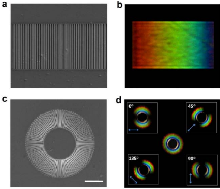
FIG. 5. (a) SEM image of the 1D plasmonic spectroscop with gradually changing periods from 400 to 200 nm (from left to right); scale bar is 2 \mu\text{m} . (b) Optical microscopy image of the plasmonic spectroscop illuminated with white light. (c) SEM image of the fabricated 2D spoke structure. Scale bar is 3 \mu\text{m} . (d) Optical microscopy images of the spoken structure illuminated with unpolarized (center) and polarized light (4 boxes).
