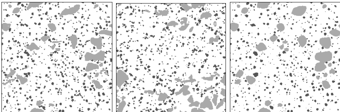
Figure 36 (a). Realistic simulated microstructure of (94\ \mu\text{m})^2 area having 10% Ti (light gray), 10% B (dark grey), 80% Al (white); (b) Hypothetical clustered microstructure like (a), different only in that mean Ti-to-B and B-to-Ti distances are 3.2\ \mu\text{m} and 8.3\ \mu\text{m} by design; (c) Hypothetical microstructure identical to (a) except that all particles are now circularized half of the way.
