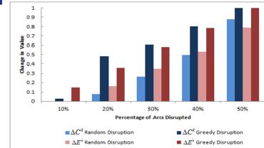
Figure 8. A bar graph displaying the average change in value at each degree of disruption while comparing random disruption approach to a greedy disruption approach for both \Delta E^k and \Delta C^k .
