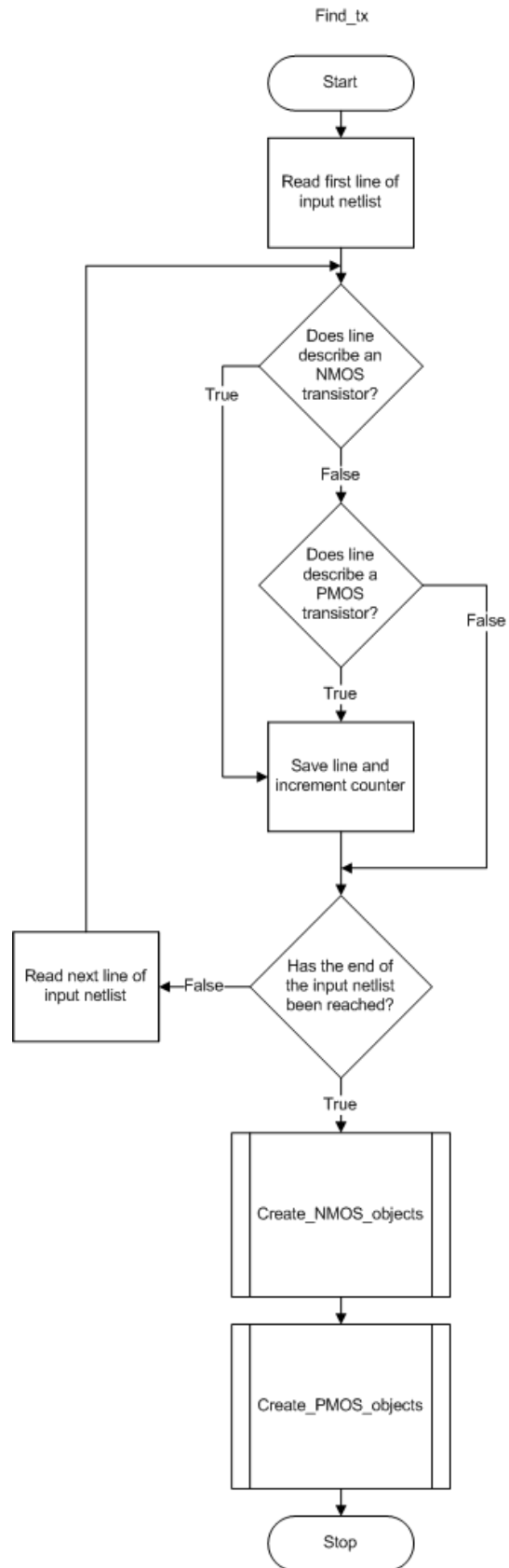
Figure 63: Flowchart of the Find_tx function in the second level of hierarchy
