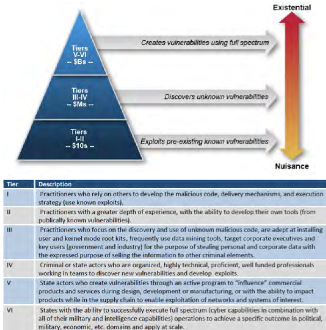
Figure 2. The Defense Science Board's 2013 cyber threat taxonomy [16].
