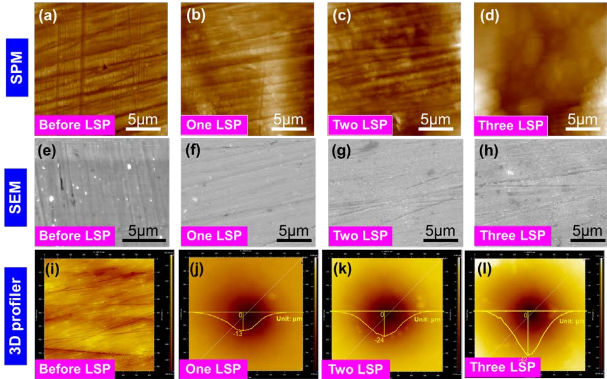
Figure 5. (a-d) SPM images of 5052 Al alloy surfaces treated by a single pulse LSP for (a) zero, (b) one, (c) two, and (d) three impacts. Corresponding (e-h) enlarged SEM images and (i-h) 3D surface topographies of the 5052 Al alloy are shown in (a-d). Insets in (j, k, l) show the cross-sectional height profiles along the lines in the same images.
