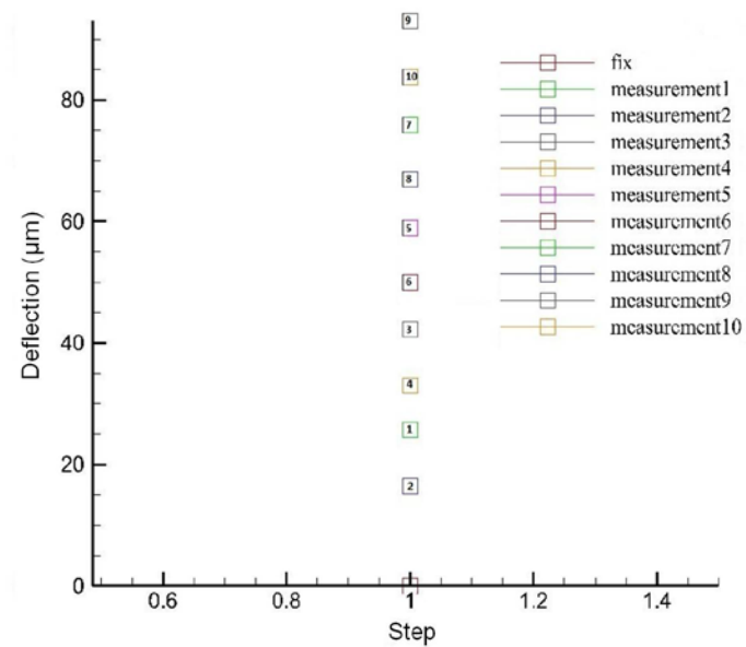
Figure 43: CoventorWare® simulation of a 10-beam “zipper” actuator with 250- \mu\text{m} -long aluminum bimorph segments located at the bottom of the cantilever beams, graph of deflections at each secondary anchor and end of the last partial-bimorph cantilever beam
