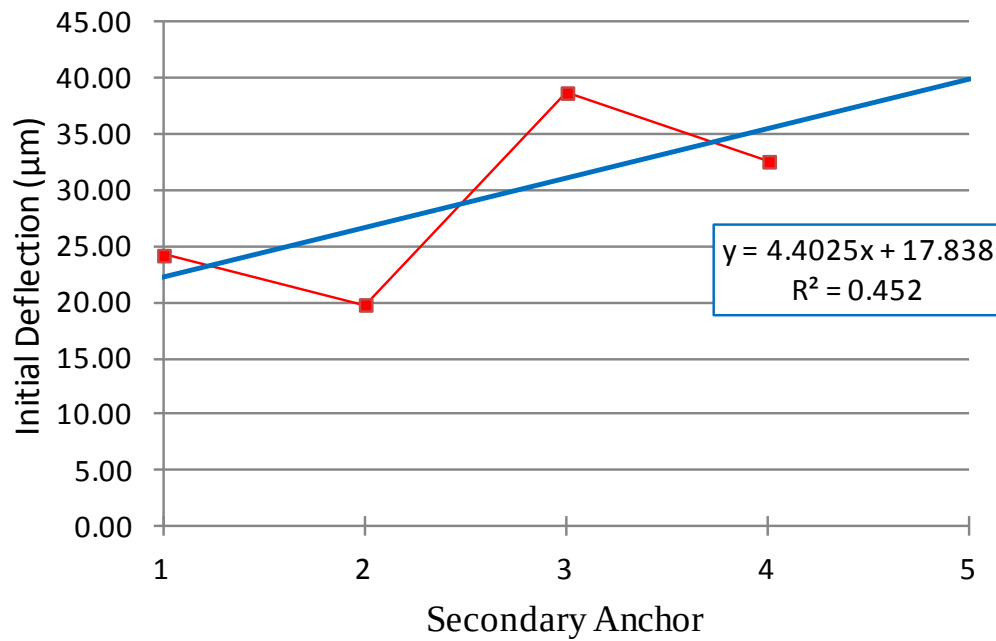
Figure 101: Graph of measured initial deflection results for PolyMUMPs® fabricated, 4-beam “zipper” actuators; 500 \mu\text{m} partial-bimorph cantilever beams with 250 \mu\text{m} bimorph segments
