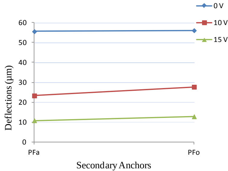
Figure 118: Graph of measured micro-mirror platform deflection results for pull-in test of PolyMUMPs® fabricated 9-beam micro-mirror platform assembly 1; measured on platform assembly 1; measured on actuation side (PF a ) and side opposite actuation (PF o )
