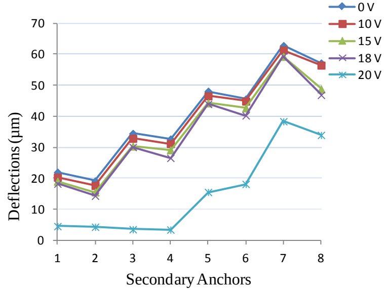
Figure 121: Graph of measured 8-beam “zipper” actuator deflection results for pull-in test of PolyMUMPs® fabricated micro-mirror platform assembly 1; measured at each secondary anchor
