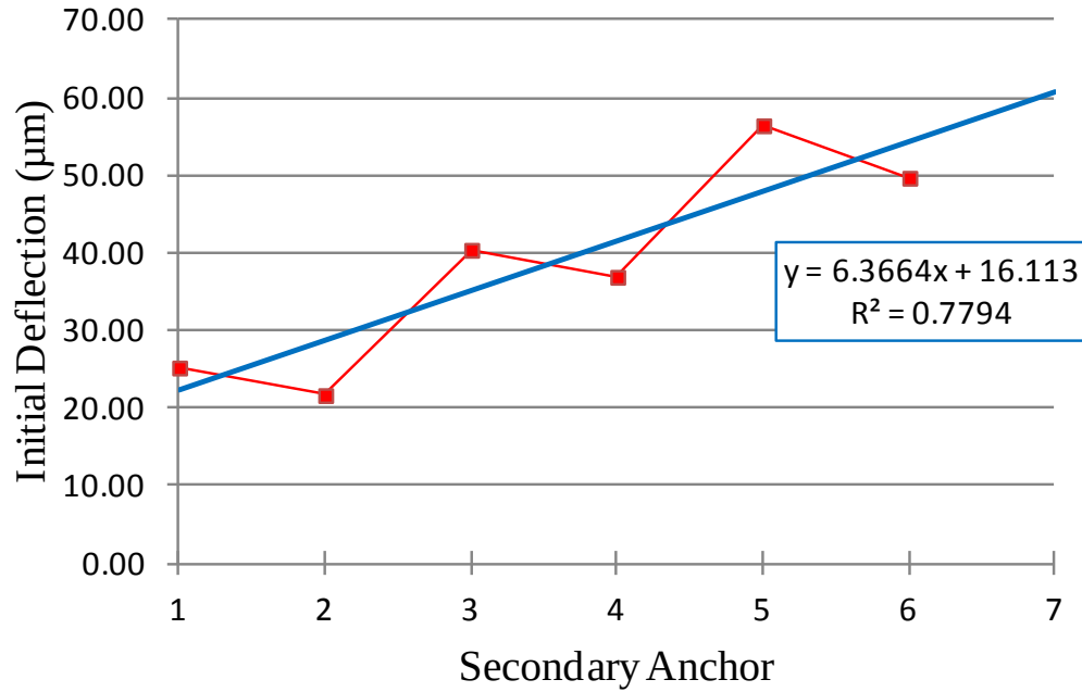
Figure 99: Graph of measured initial deflection results for PolyMUMPs® fabricated, 6-beam “zipper” actuators; 500 \mu\text{m} partial-bimorph cantilever beams with 250 \mu\text{m} bimorph segments
