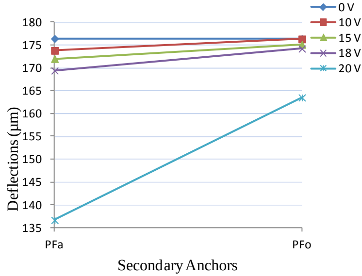
Figure 110: Graph of measured micro-mirror platform deflection results for pull-in test of PolyMUMPs® fabricated 22-beam micro-mirror platform assembly 2; measured on actuation side ( PF_a ) and side opposite actuation ( PF_o )
