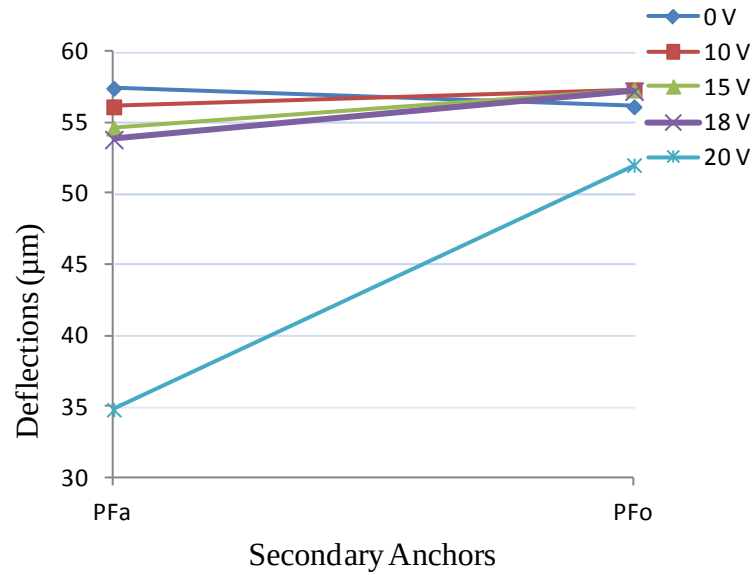
Figure 122: Graph of measured micro-mirror platform deflection results for pull-in test of PolyMUMPs® fabricated 8-beam micro-mirror platform assembly 1; measured on actuation side (PF a ) and side opposite actuation (PF o )
