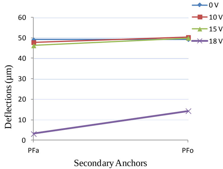
Figure 130: Graph of measured micro-mirror platform deflection results for pull-in test of PolyMUMPs® fabricated 7-beam micro-mirror platform assembly 3; measured on actuation side ( PF_a ) and side opposite actuation ( PF_o )
