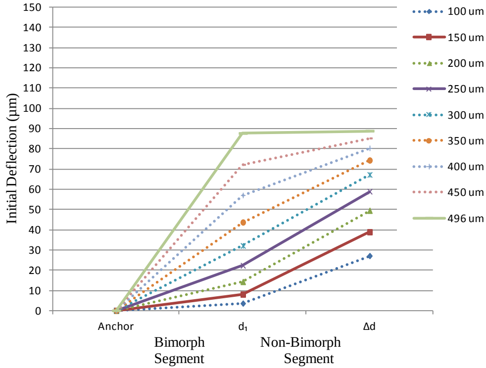
Figure 83: Graph of calculated initial deflection results for a 500 \mu\text{m} partial-bimorph cantilever beam with varied bimorph segments and a temperature change of 150° C
