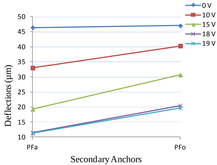
Figure 160: Graph of measured micro-mirror platform deflection results for pull-in test of PolyMUMPs® fabricated 7-beam (corrugated) micro-mirror platform assembly 1; measured on actuation side (PF a ) and side opposite actuation (PF o )
