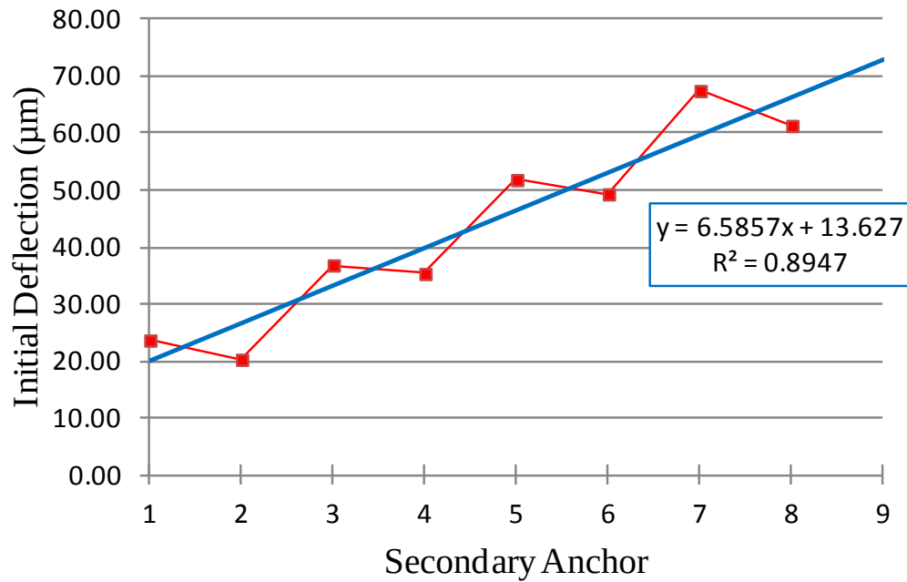
Figure 97: Graph of measured initial deflection results for PolyMUMPs® fabricated, 8-beam “zipper” actuators; 500 \mu\text{m} partial-bimorph cantilever beams with 250 \mu\text{m} bimorph segments
