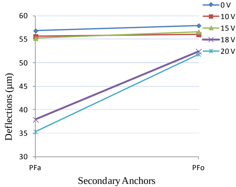
Figure 124: Graph of measured micro-mirror platform deflection results for pull-in test of PolyMUMPs® fabricated 8-beam micro-mirror platform assembly 2; measured on actuation side (PF a ) and side opposite actuation (PF o )
