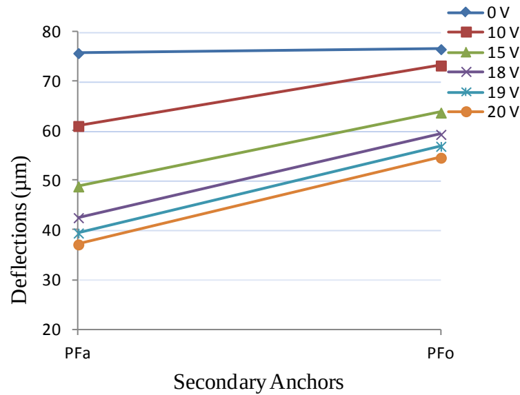
Figure 150: Graph of measured micro-mirror platform deflection results for pull-in test of PolyMUMPs® fabricated 11-beam (corrugated) micro-mirror platform assembly 1; measured on actuation side (PF a ) and side opposite actuation (PF o )
