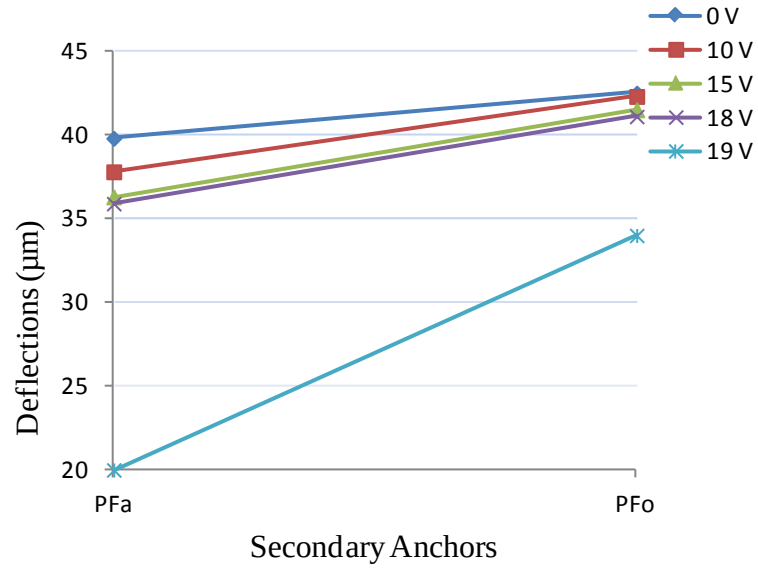
Figure 134: Graph of measured micro-mirror platform deflection results for pull-in test of PolyMUMPs® fabricated 6-beam micro-mirror platform assembly 2; measured on actuation side (PF a ) and side opposite actuation (PF o )
