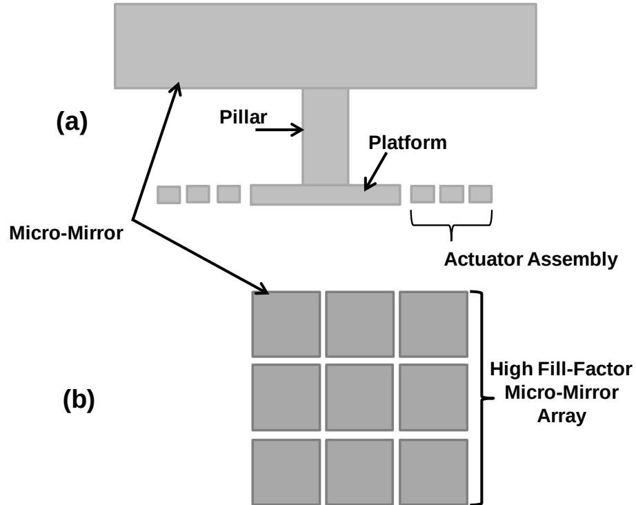
Figure 19: Illustration showing how platform actuation assembly is to be incorporated into a micro-mirror array: (a) a cross-section of a single micro-mirror element with mirror and pillar assembly bonded to micro-mirror actuation assembly, (b) a representative top view showing the high fill-factor mirror array
