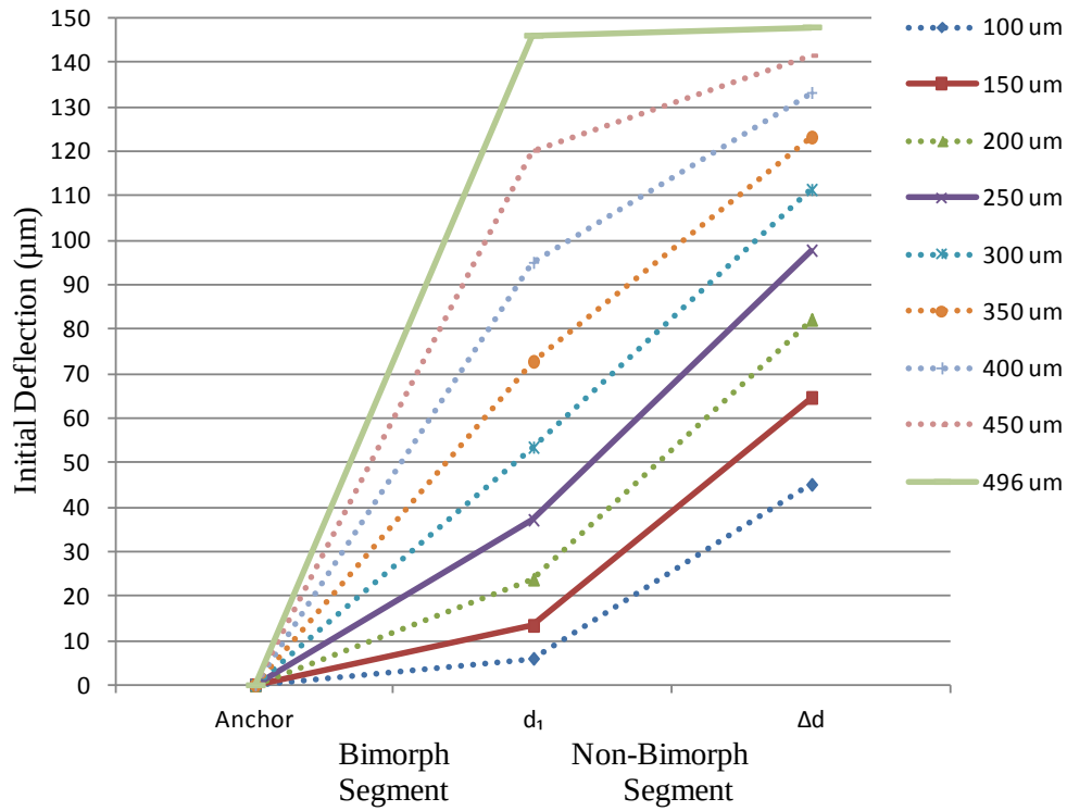
Figure 85: Graph of calculated initial deflection results for a 500 \mu\text{m} partial-bimorph cantilever beam with varied bimorph segments and a temperature change of 250° C
