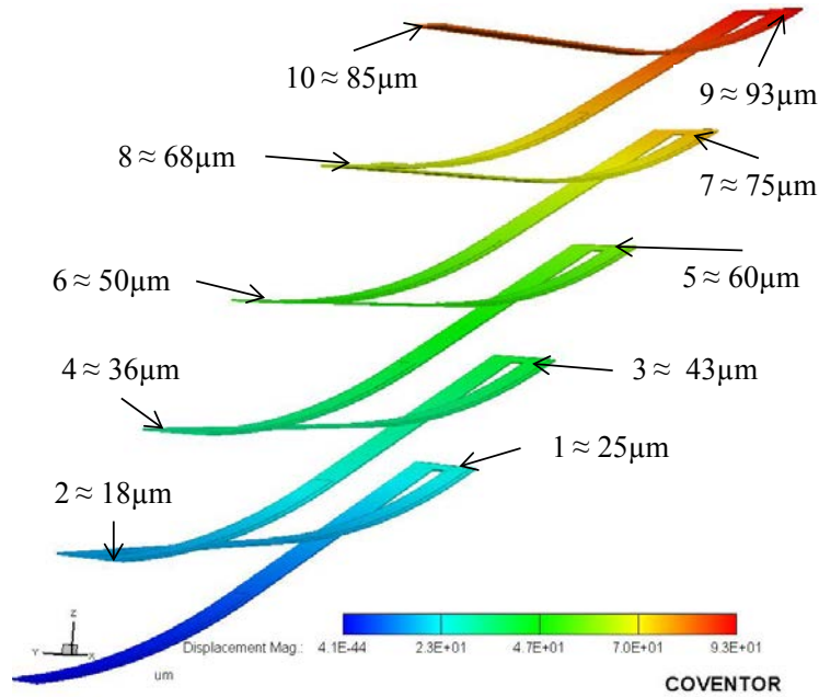
Figure 42: CoventorWare® simulation of a 10-beam “zipper” actuator with 250- \mu\text{m} -long aluminum bimorph segments located at the bottom of the cantilever beams, 3D deformation model
