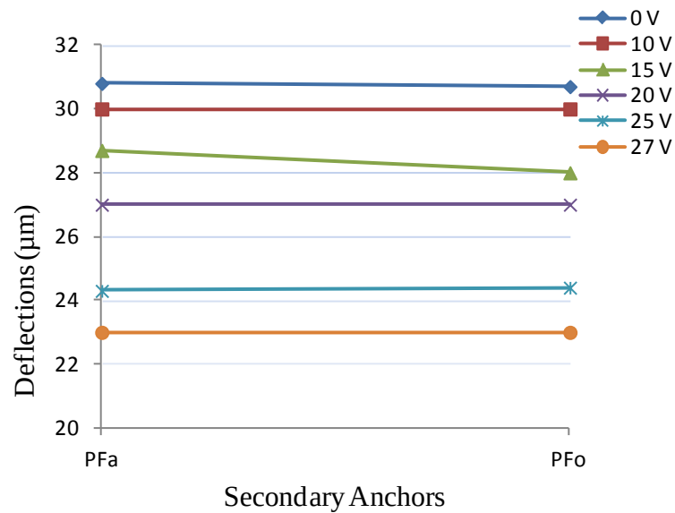
Figure 140: Graph of measured micro-mirror platform deflection results for pull-in test of PolyMUMPs® fabricated 4-beam micro-mirror platform assembly 1; measured on actuation side (PF a ) and side opposite actuation (PF o )
