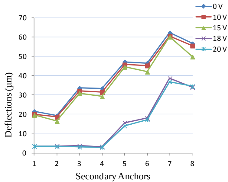
Figure 122: Graph of measured micro-mirror platform deflection results for pull-in test of PolyMUMPs® fabricated 8-beam micro-mirror platform assembly 1; measured on actuation side (PF a ) and side opposite actuation (PF o )
