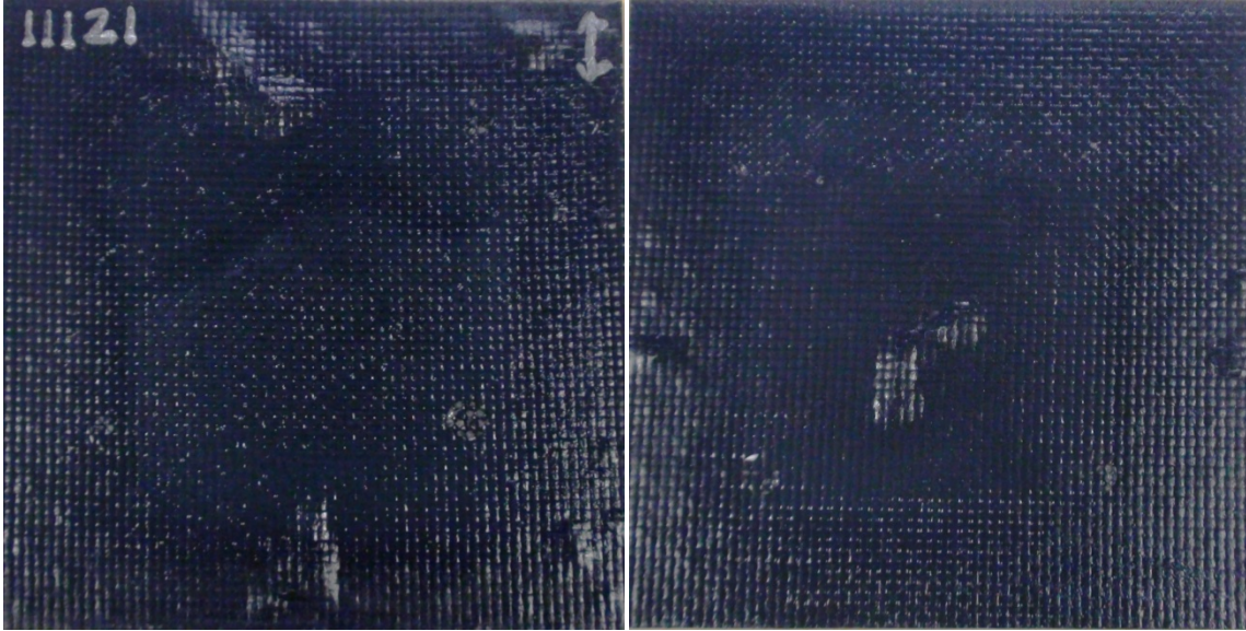
Figure B.11: T300/HYPR-SiC™ – 100h 1300°C exposure plate 11121 top face (left) and bottom face (right) Plate exhibits mild blistering and a glossy appearance.
