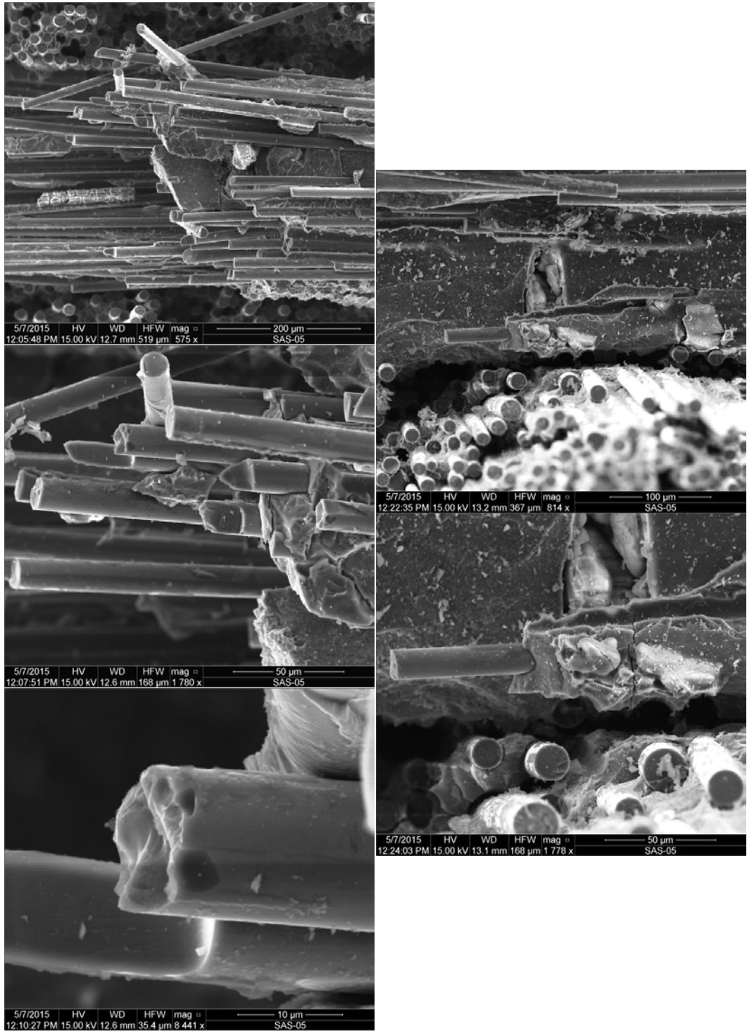
Figure J. 15: SEM micrographs of a fracture surface obtained in tensile test of a Hi-Nicalon™/SiNC specimen subjected to prior heat treatment for 100 h at 1300°C (Plate 11105, Specimen 6)
