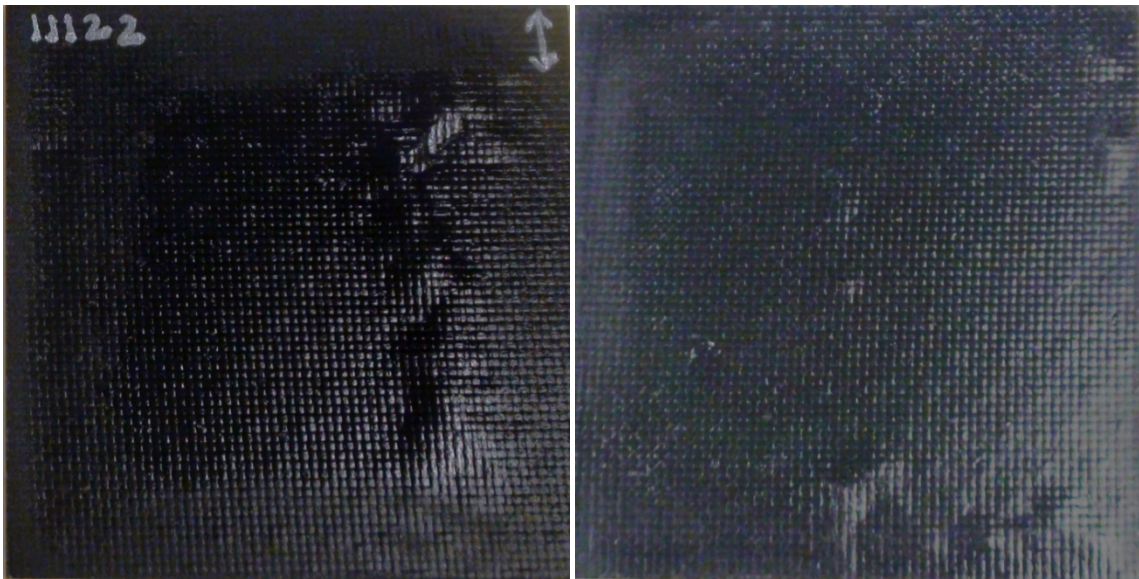
Figure B.12: T300/HYPR-SiC™ – 100h 1200°C exposure plate 11122 top face (left) and bottom face (right) Plate exhibits mild blistering and a glossy appearance.
