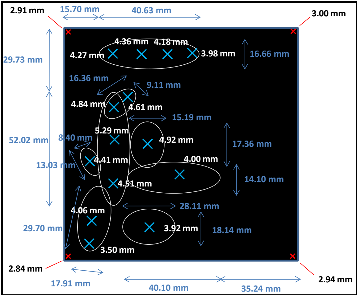
Figure C.4: Diagram of blistered C/HYPR-SiC™ plate after 20 h 1300°C exposure – plate 11124, face down
