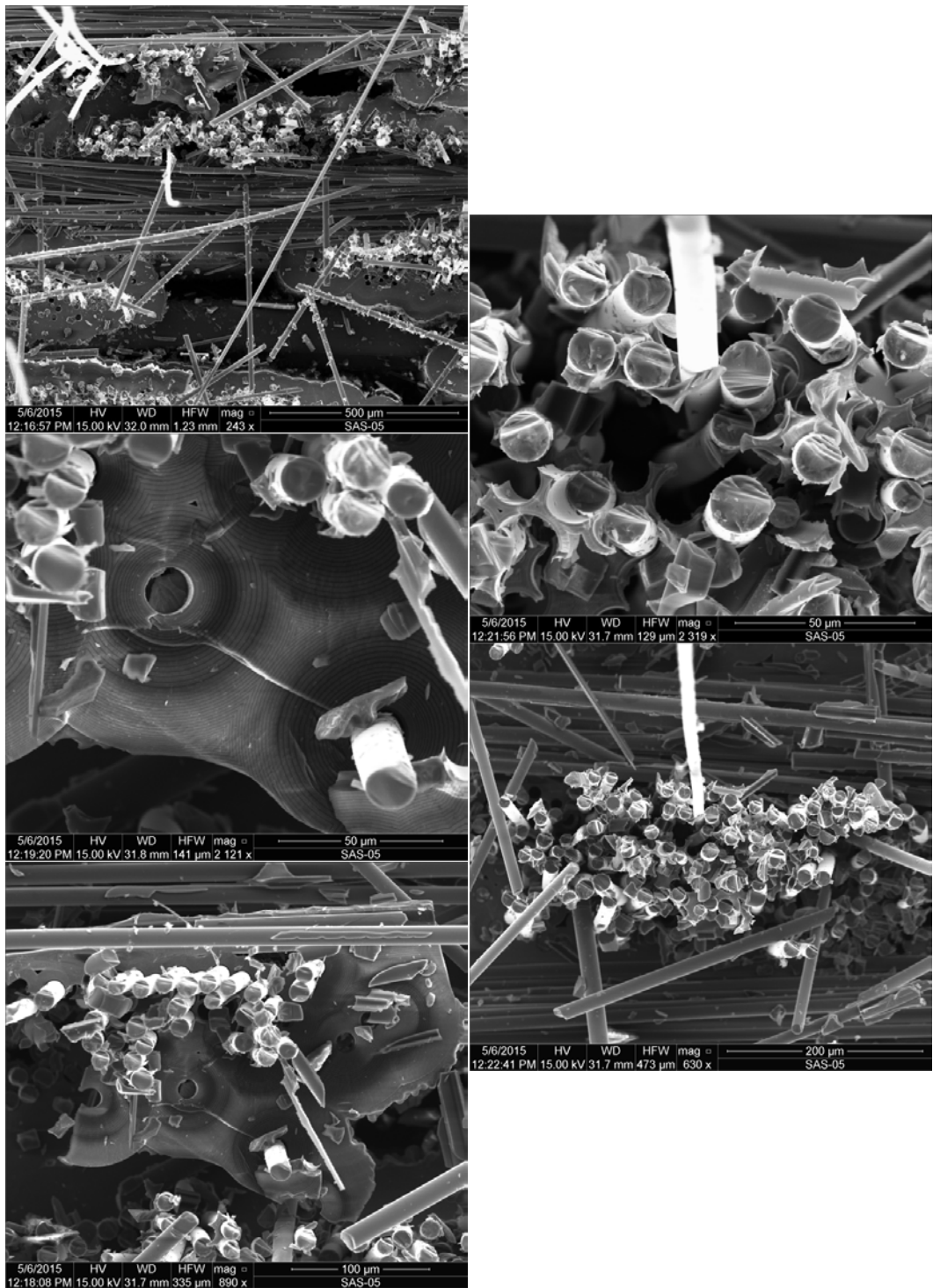
Figure M. 7: SEM micrographs of a fracture surface obtained in tensile test of a Hi-Nicalon™/HYPR-SiC™ specimen subjected to prior heat treatment for 10 h at 1400°C (Plate 11133, Specimen 2)
