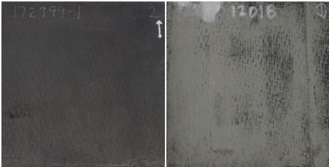
Figure 12: Example of HexTow® IM7/SiC plate discoloration due to heat treatment – virgin plate (left); exposed plate (right).
