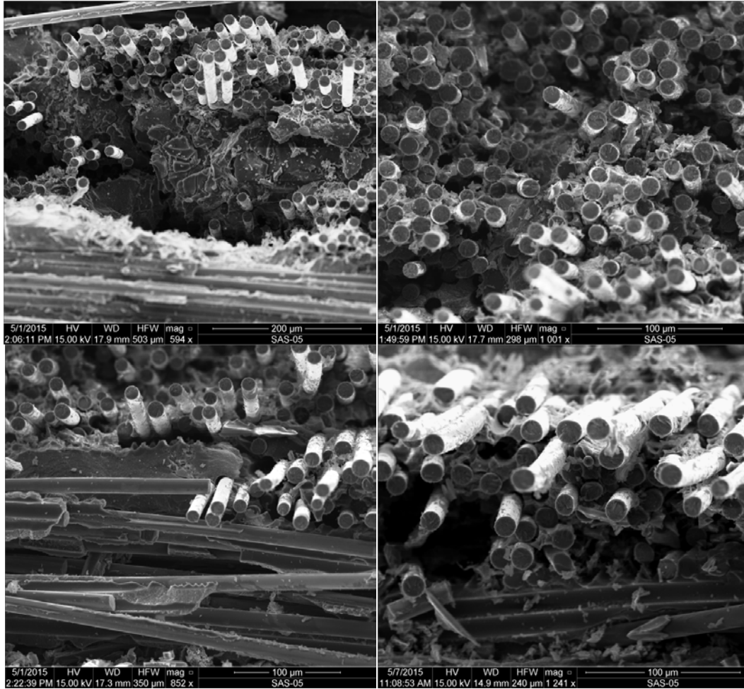
Figure J. 10: SEM micrographs of a fracture surface obtained in tensile test of a Hi-Nicalon™/SiNC specimen subjected to prior heat treatment for 10 h at 1300°C (Plate 11101, Specimen 6)
