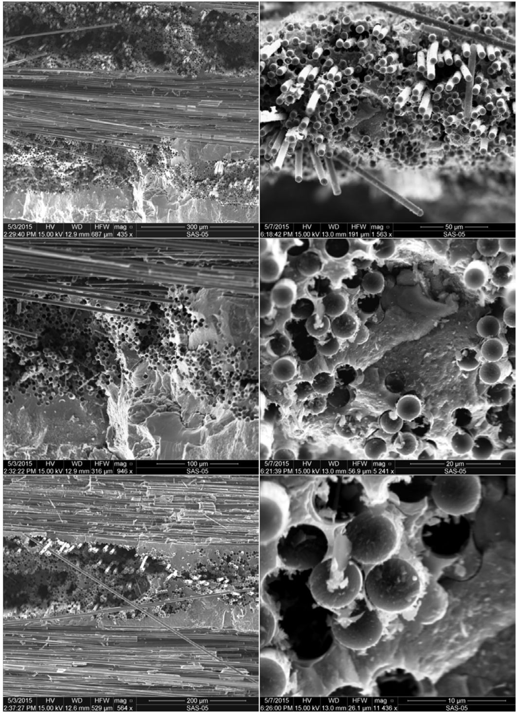
Figure K. 3: SEM micrographs of a fracture surface obtained in tensile test of a virgin C/SiC specimen (Plate 12012, Specimen 6)
