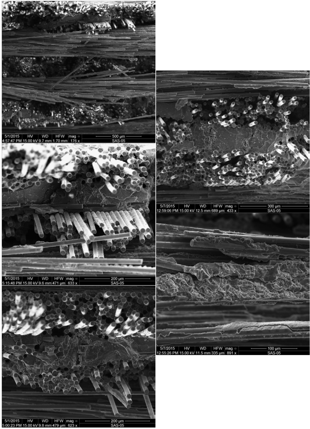
Figure J. 17: SEM micrographs of a fracture surface obtained in tensile test of a Hi-Nicalon™/SiNC specimen subjected to prior heat treatment for 100 h at 1200°C (Plate 11106, Specimen 4)
