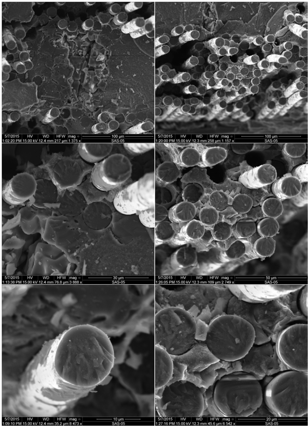
Figure J. 19: SEM micrographs of a fracture surface obtained in tensile test of a Hi-Nicalon™/SiNC specimen subjected to prior heat treatment for 100 h at 1200°C (Plate 11106, Specimen 4)
