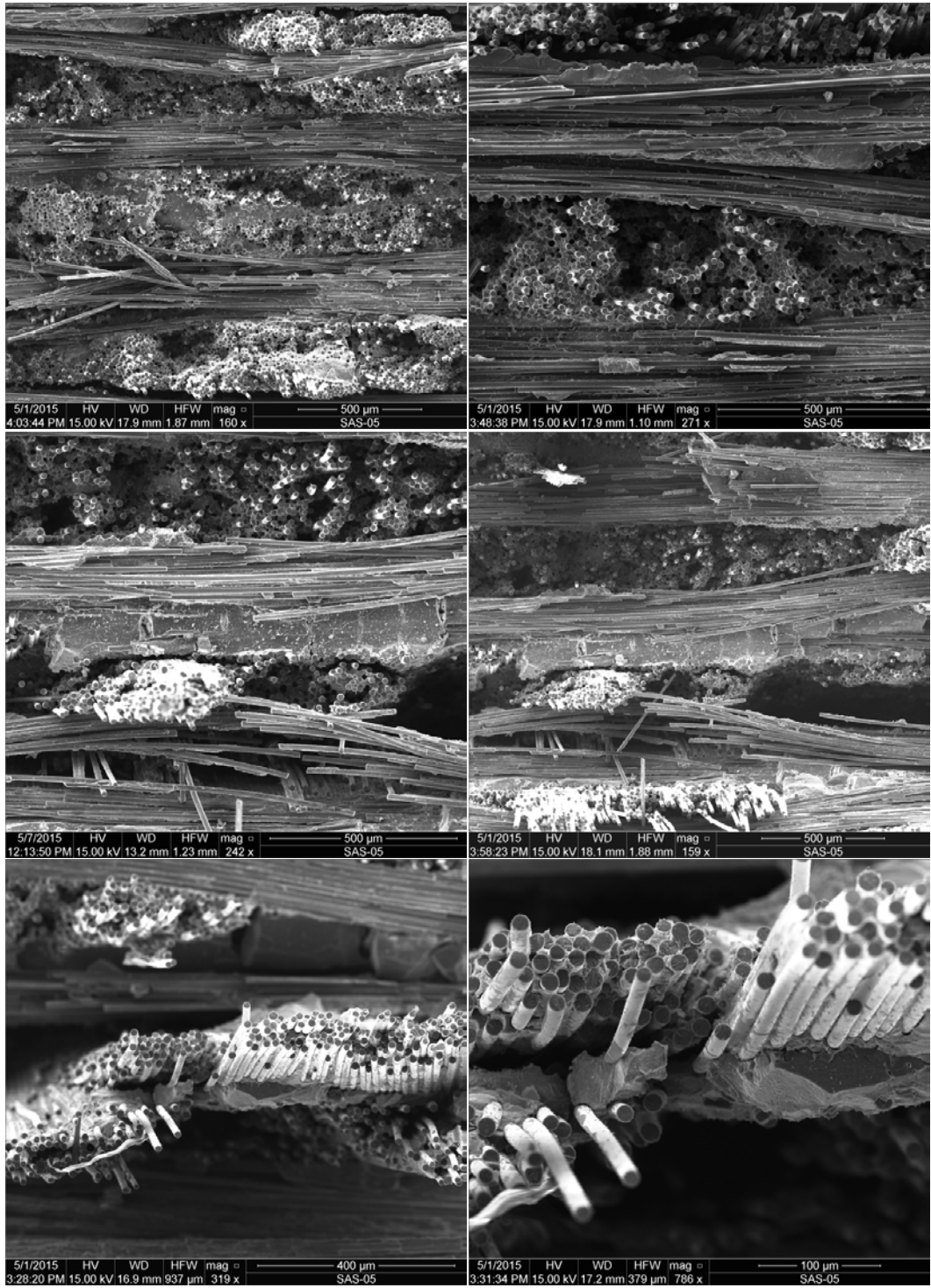
Figure J. 13: SEM micrographs of a fracture surface obtained in tensile test of a Hi-Nicalon™/SiNC specimen subjected to prior heat treatment for 100 h at 1300°C (Plate 11105, Specimen 6)
