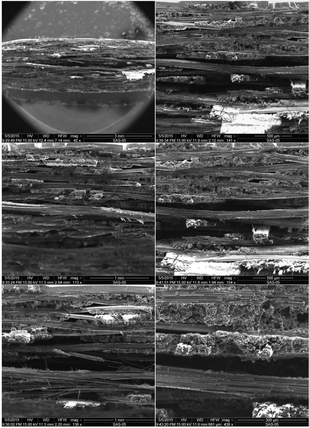
Figure L. 14: SEM micrographs of a fracture surface obtained in tensile test of a C/HYPR-SiC™ specimen subjected to prior heat treatment for 100 h at 1200°C (Plate 11122, Specimen 5)
