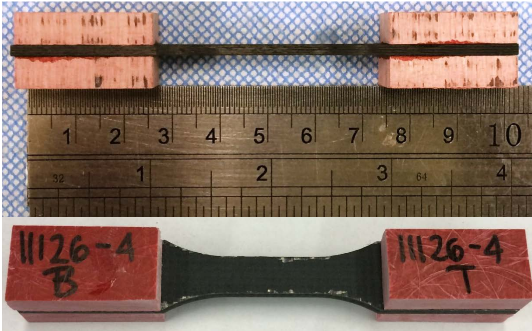
Figure 19: Test-ready specimen – edge view (top) and face-up (bottom)
