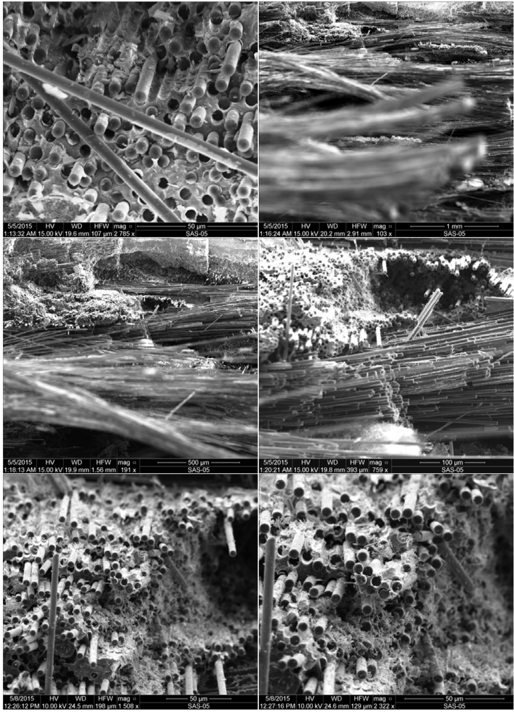
Figure K. 18: SEM micrographs of a fracture surface obtained in tensile test of a C/SiC specimen subjected to prior heat treatment for 100 h at 1300°C (Plate 12015, Specimen 3)
