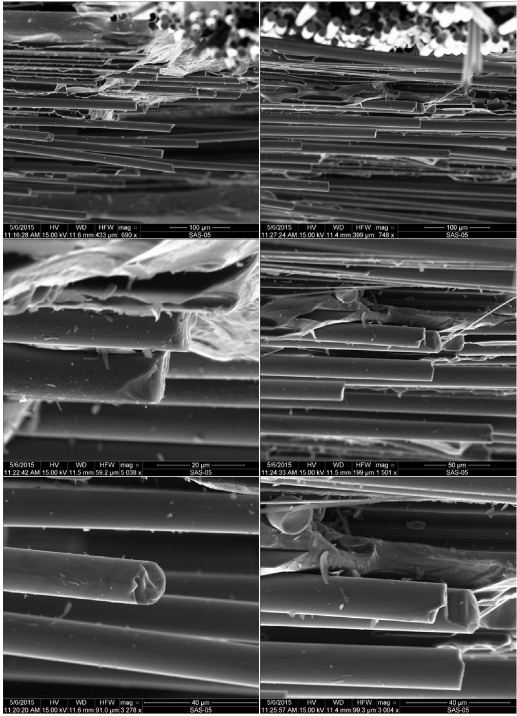
Figure M. 15: SEM micrographs of a fracture surface obtained in tensile test of a Hi-Nicalon™/HYPR-SiC™ specimen subjected to prior heat treatment for 100 h at 1300°C (Plate 11139, Specimen 1)
