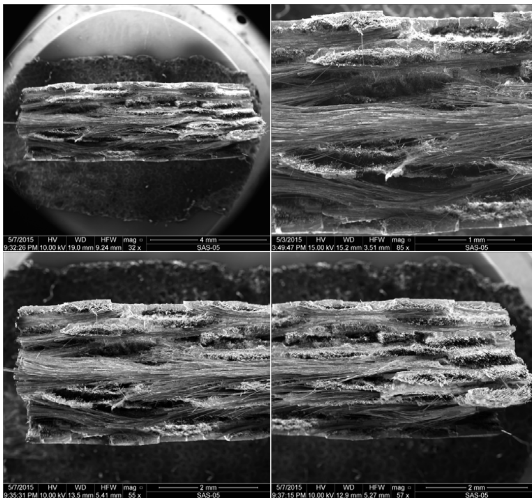
Figure K. 7: SEM micrographs of a fracture surface obtained in tensile test of a C/SiC specimen subjected to prior heat treatment for 40 h at 1300°C (Plate 12018, Specimen 2)
