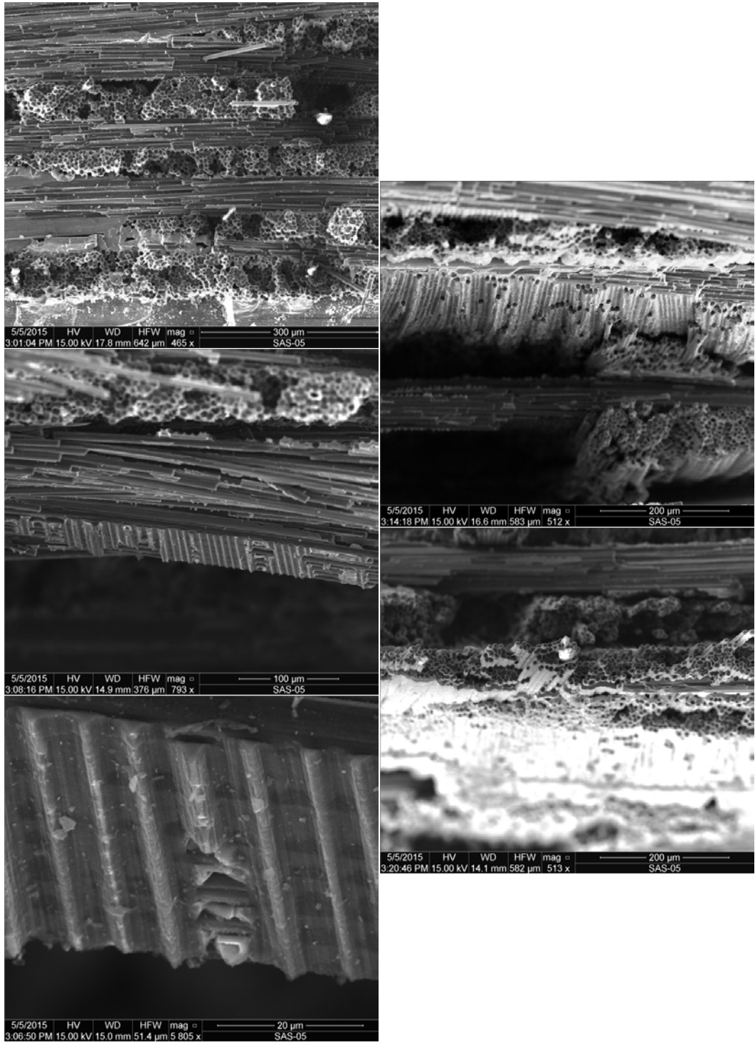
Figure L. 4: SEM micrographs of a fracture surface obtained in tensile test of a virgin C/HYPR-SiC™ specimen (Plate 11126, Specimen 4)
