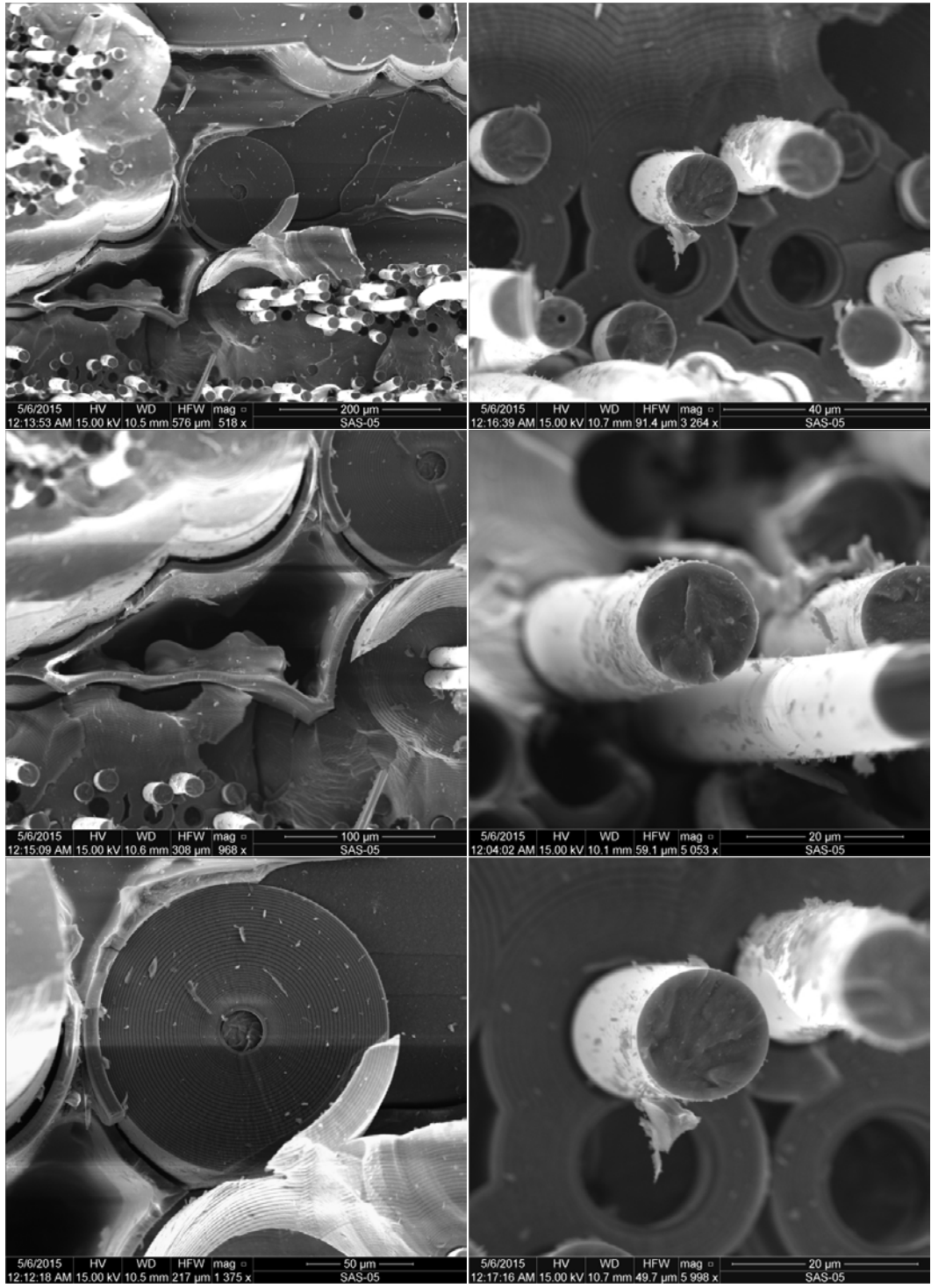
Figure M. 9: SEM micrographs of a fracture surface obtained in tensile test of a Hi-Nicalon™/HYPR-SiC™ specimen subjected to prior heat treatment for 100 h at 1400°C (Plate 11137, Specimen 6)
