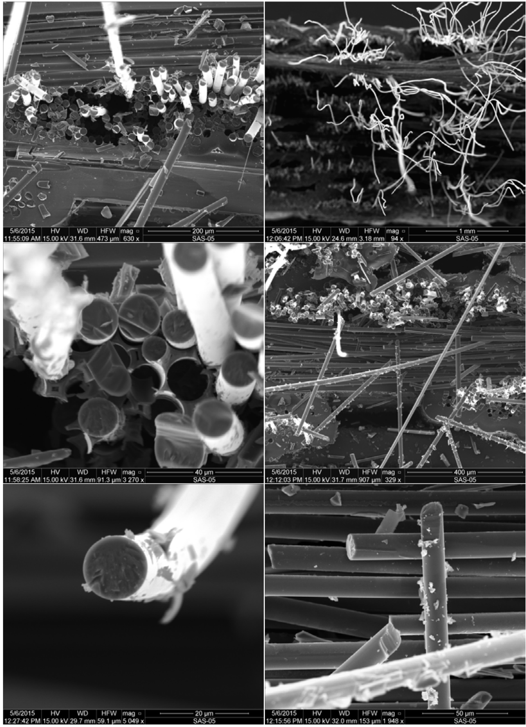
Figure M. 6: SEM micrographs of a fracture surface obtained in tensile test of a Hi-Nicalon™/HYPR-SiC™ specimen subjected to prior heat treatment for 10 h at 1400°C (Plate 11133, Specimen 2)
