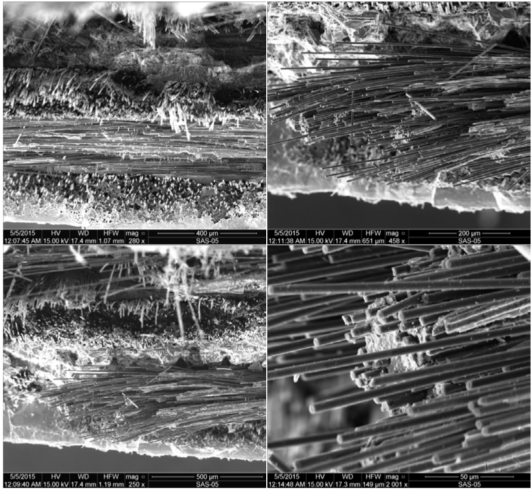
Figure K. 27: SEM micrographs of a fracture surface obtained in tensile test of a C/SiC specimen subjected to prior heat treatment for 100 h at 1200°C (Plate 12016, Specimen 3)
