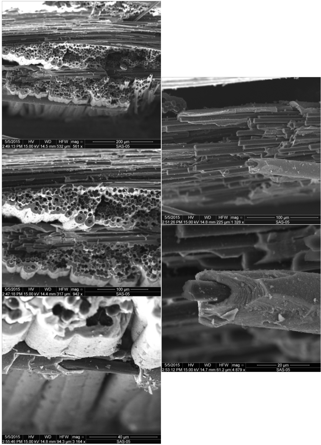
Figure L. 3: SEM micrographs of a fracture surface obtained in tensile test of a virgin C/HYPR-SiC™ specimen (Plate 11126, Specimen 4)
