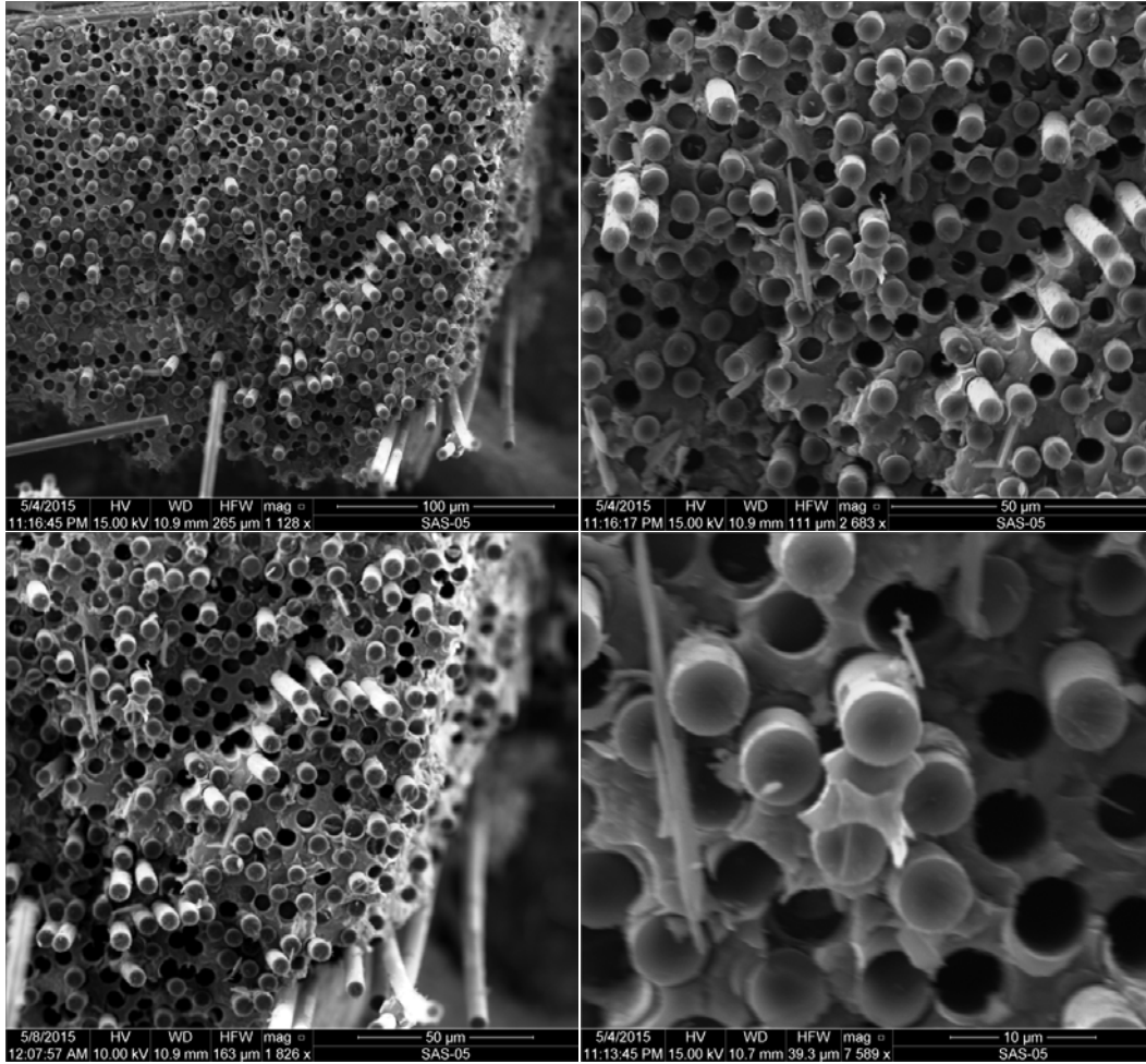
Figure K. 22: SEM micrographs of a fracture surface obtained in tensile test of a C/SiC specimen subjected to prior heat treatment for 100 h at 1200°C (Plate 12016, Specimen 3)
