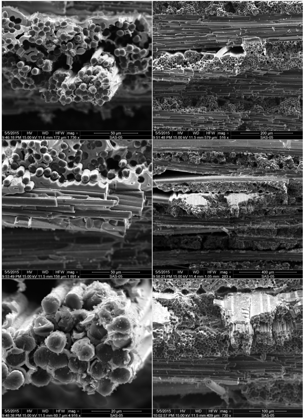
Figure L. 15: SEM micrographs of a fracture surface obtained in tensile test of a C/HYPR-SiC™ specimen subjected to prior heat treatment for 100 h at 1200°C (Plate 11122, Specimen 5)
