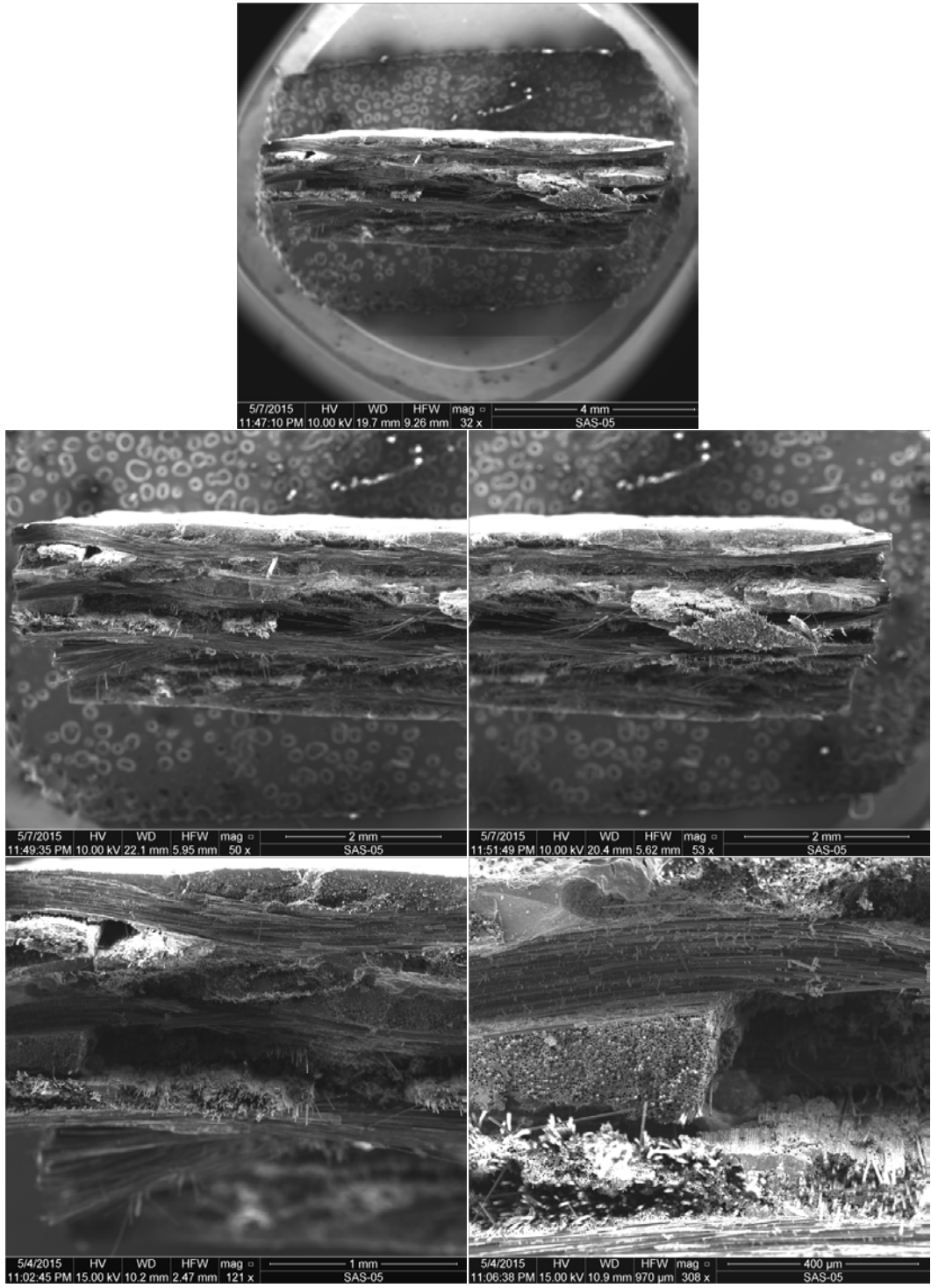
Figure K. 21: SEM micrographs of a fracture surface obtained in tensile test of a C/SiC specimen subjected to prior heat treatment for 100 h at 1200°C (Plate 12016, Specimen 3)
