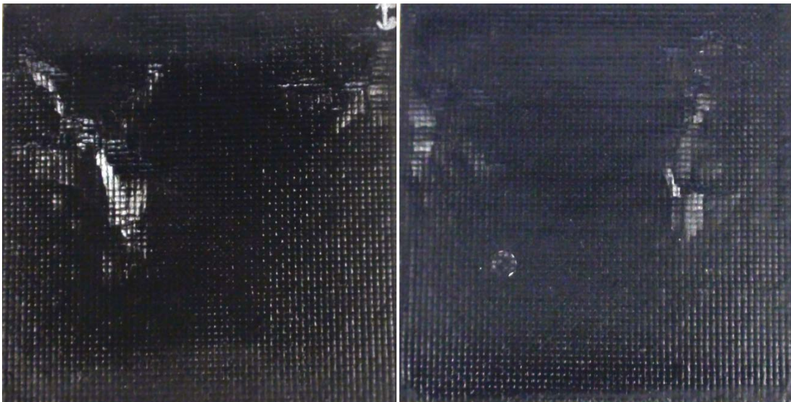
Figure B.10: T300/HYPR-SiC™ – 40h 1300°C exposure plate 11125 top face (left) and bottom face (right) Plate exhibits moderate blistering and a glossy appearance.
