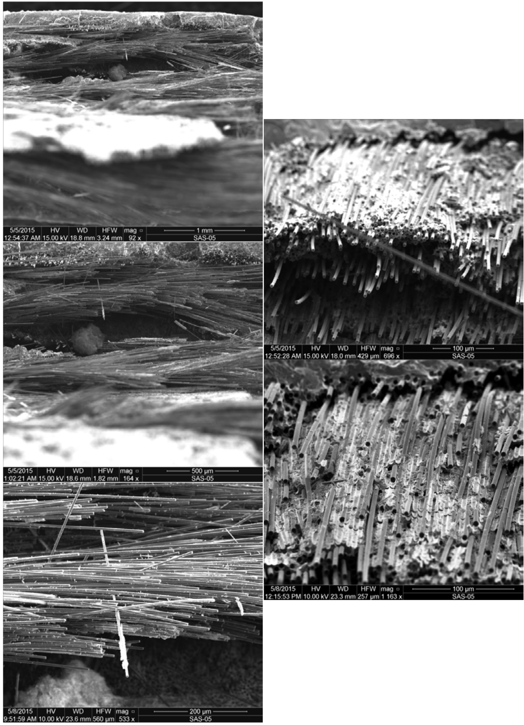
Figure K. 16: SEM micrographs of a fracture surface obtained in tensile test of a C/SiC specimen subjected to prior heat treatment for 100 h at 1300°C (Plate 12015, Specimen 3)
