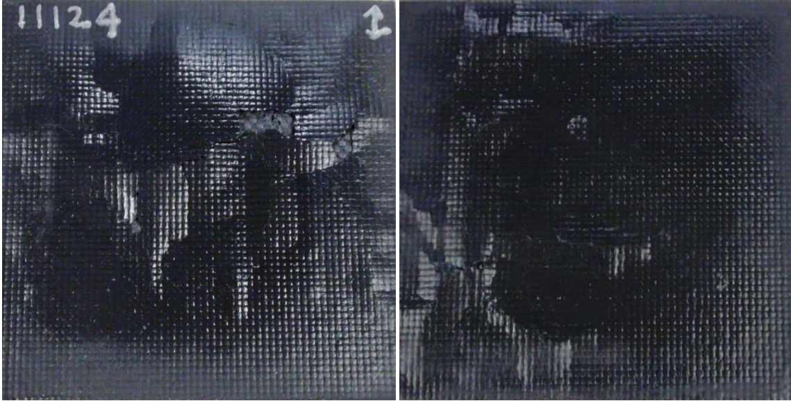
Figure B.9: T300/HYPR-SiC™ – 20h 1300°C exposure plate 11124 top face (left) and bottom face (right) Plate exhibits severe blistering and a glossy appearance.
