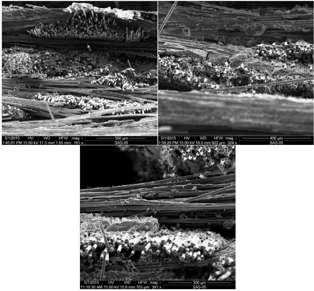
Figure J. 9: SEM micrographs of a fracture surface obtained in tensile test of a Hi-Nicalon™/SiNC specimen subjected to prior heat treatment for 10 h at 1300°C (Plate 11101, Specimen 6)
