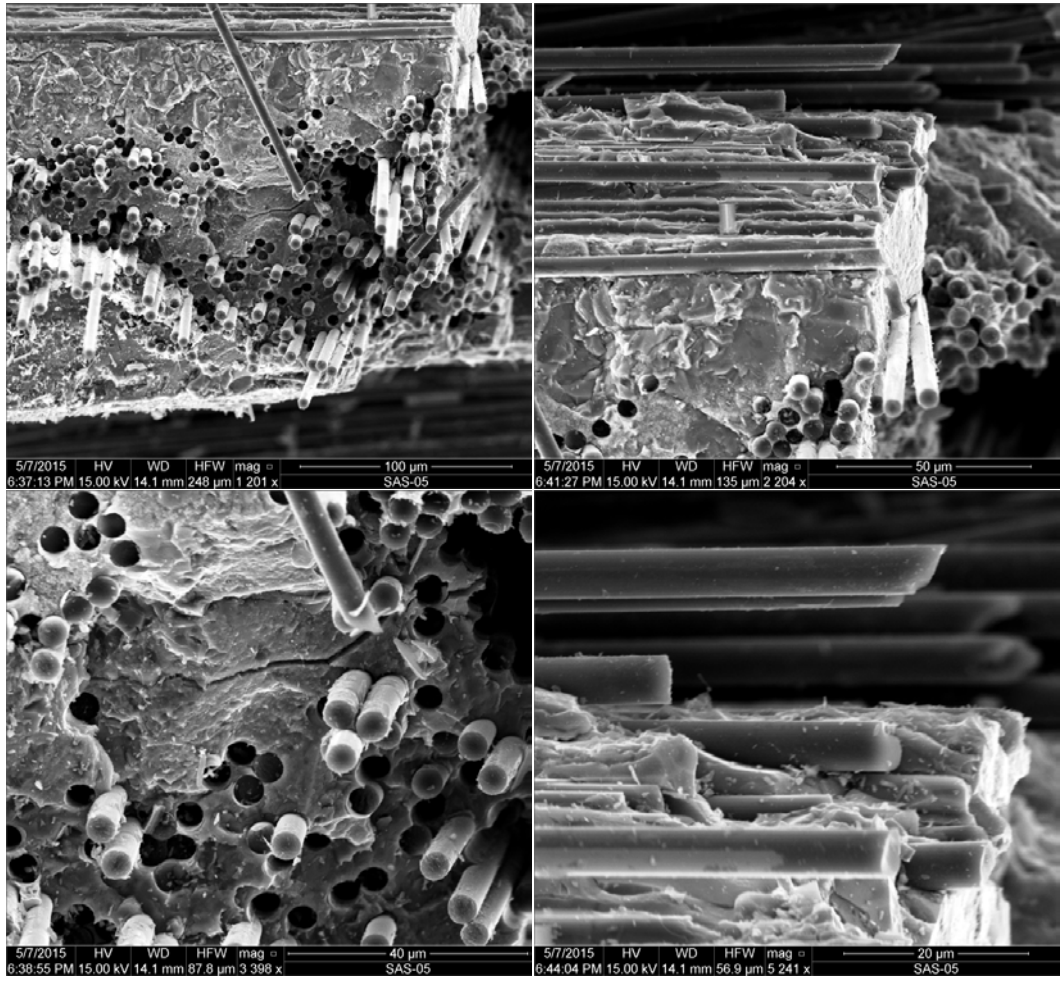
Figure K. 2: SEM micrographs of a fracture surface obtained in tensile test of a virgin C/SiC specimen (Plate 12012, Specimen 6)
