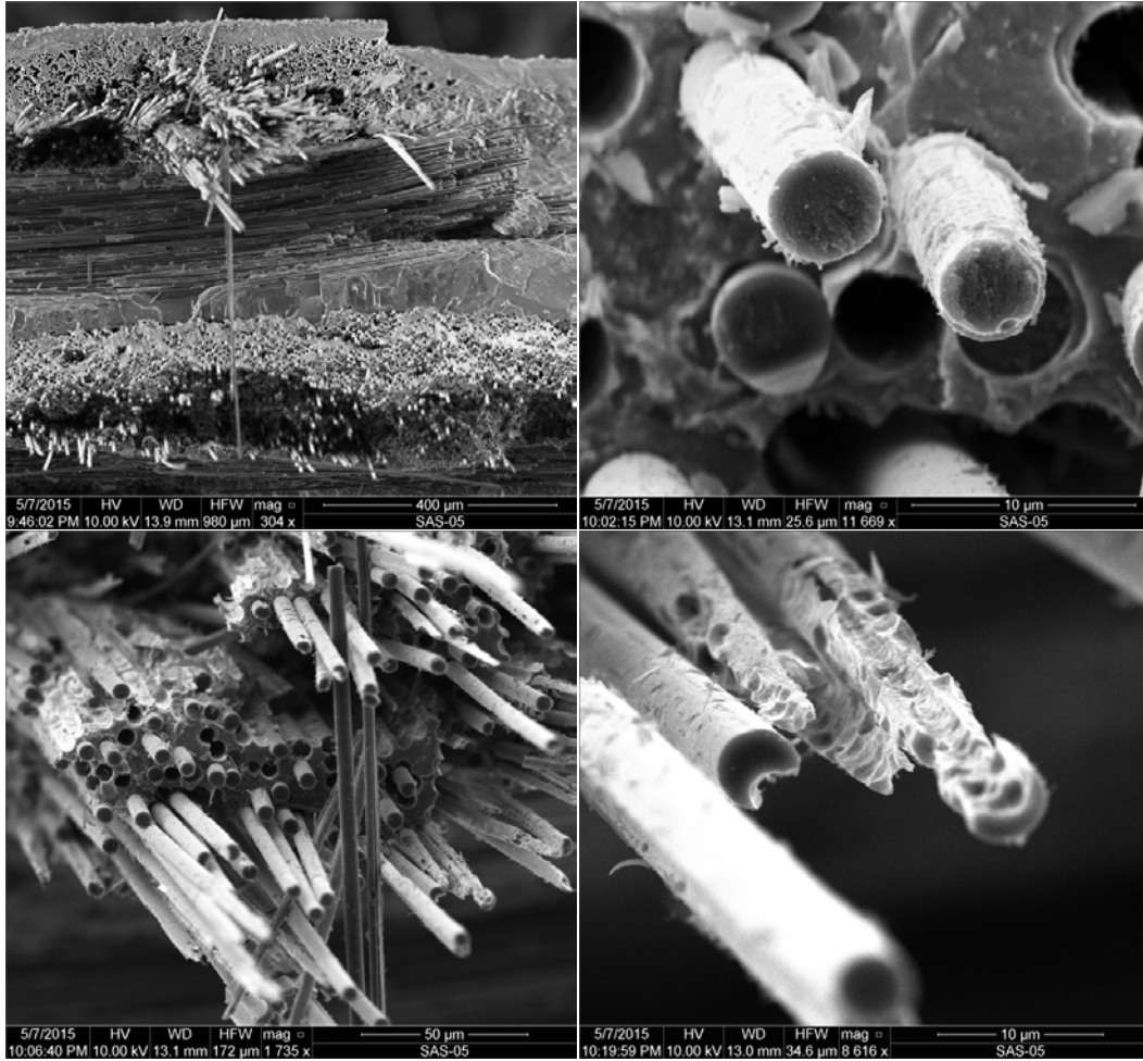
Figure K. 8: SEM micrographs of a fracture surface obtained in tensile test of a C/SiC specimen subjected to prior heat treatment for 40 h at 1300°C (Plate 12018, Specimen 2)
