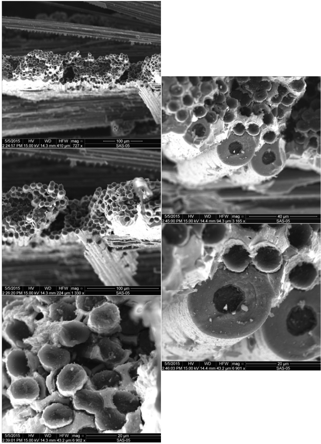
Figure L. 2: SEM micrographs of a fracture surface obtained in tensile test of a virgin C/HYPR-SiC™ specimen (Plate 11126, Specimen 4)
