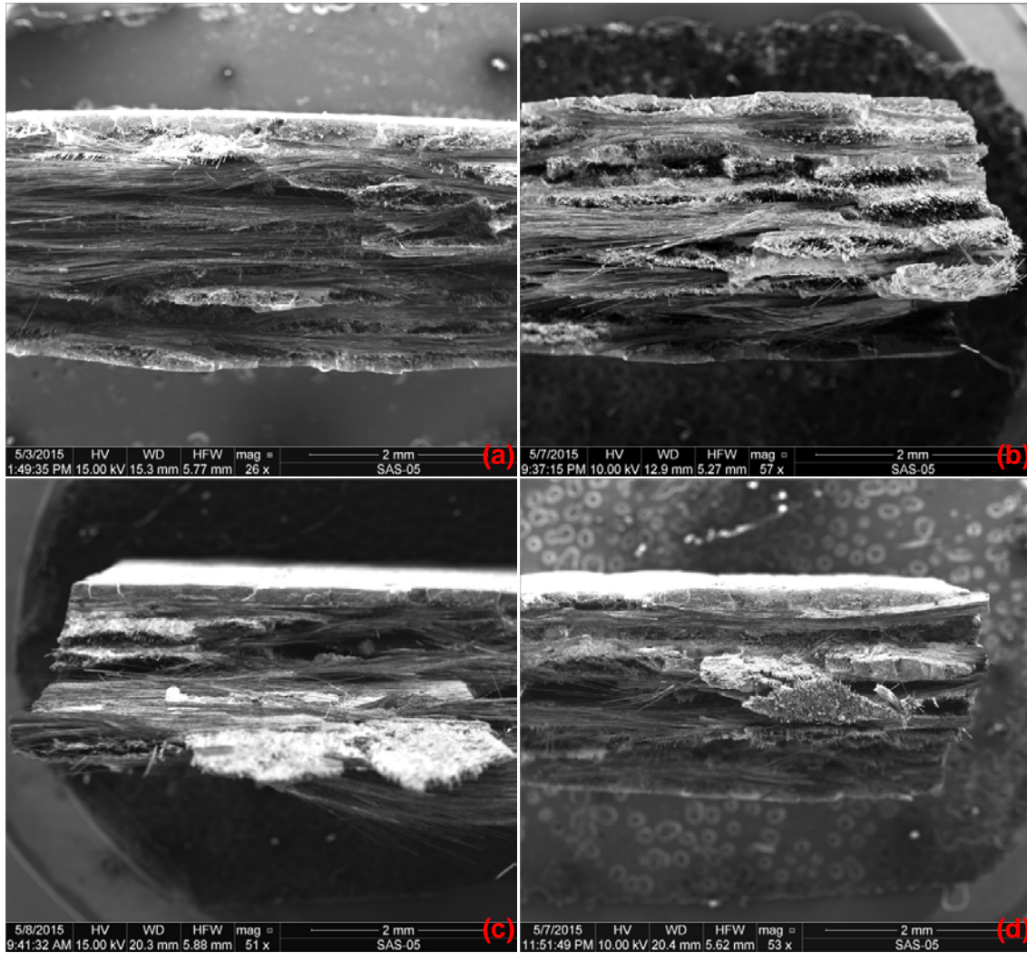
Figure 45: SEM micrographs of fracture surfaces obtained in tensile tests of C/SiC – (a) virgin specimen; and specimens exposed for (b) 40 h at 1300°C; (c) 100 h at 1300°C; and (d) 100 h at 1200°C
