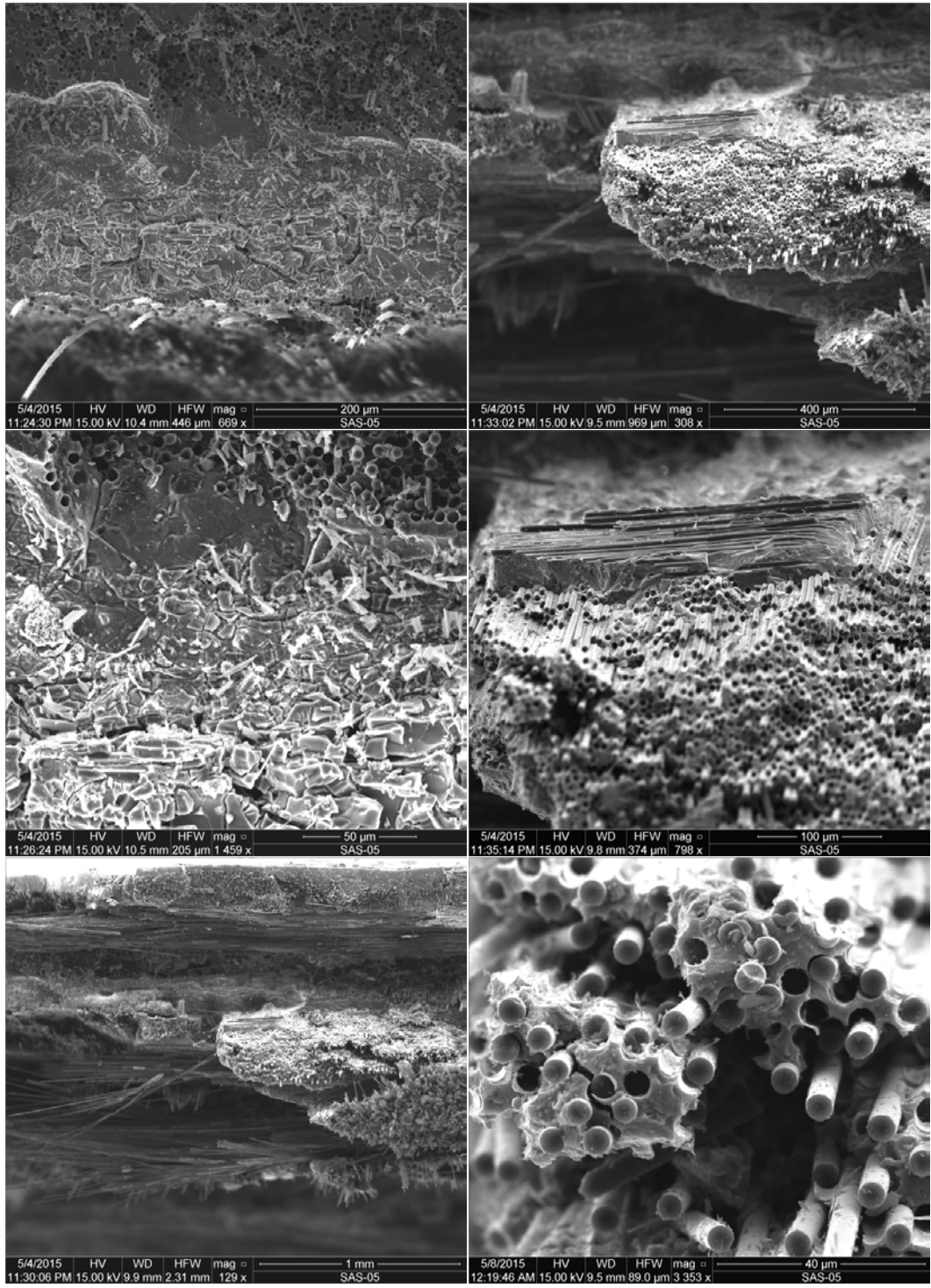
Figure K. 23: SEM micrographs of a fracture surface obtained in tensile test of a C/SiC specimen subjected to prior heat treatment for 100 h at 1200°C (Plate 12016, Specimen 3)
