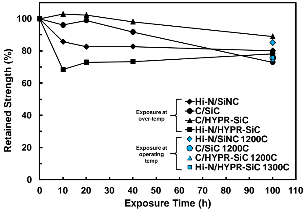
Figure 31: Comparison of retained strength with time-temperature history for all CMCs
