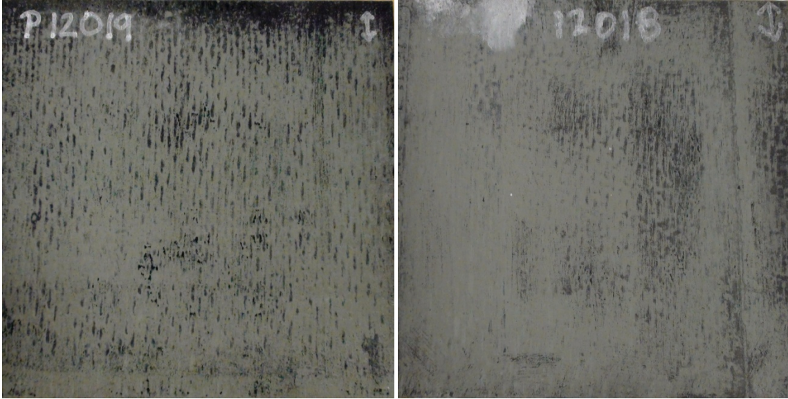
Figure B. 5: HexTow ® IM7/SiC – 20h 1300°C exposure plate 12019 (left); 40h 1300°C exposure plate 12018 (right). Exposed plates exhibit discoloration.
