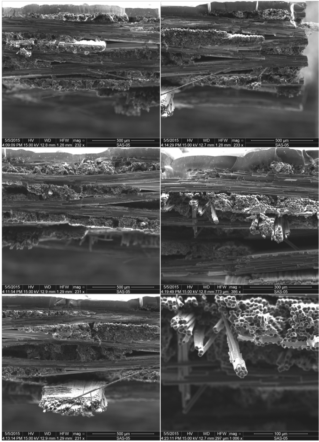
Figure L. 6: SEM micrographs of a fracture surface obtained in tensile test of a C/HYPR-SiC™ specimen subjected to prior heat treatment for 40 h at 1300°C (Plate 11125, Specimen 4)
