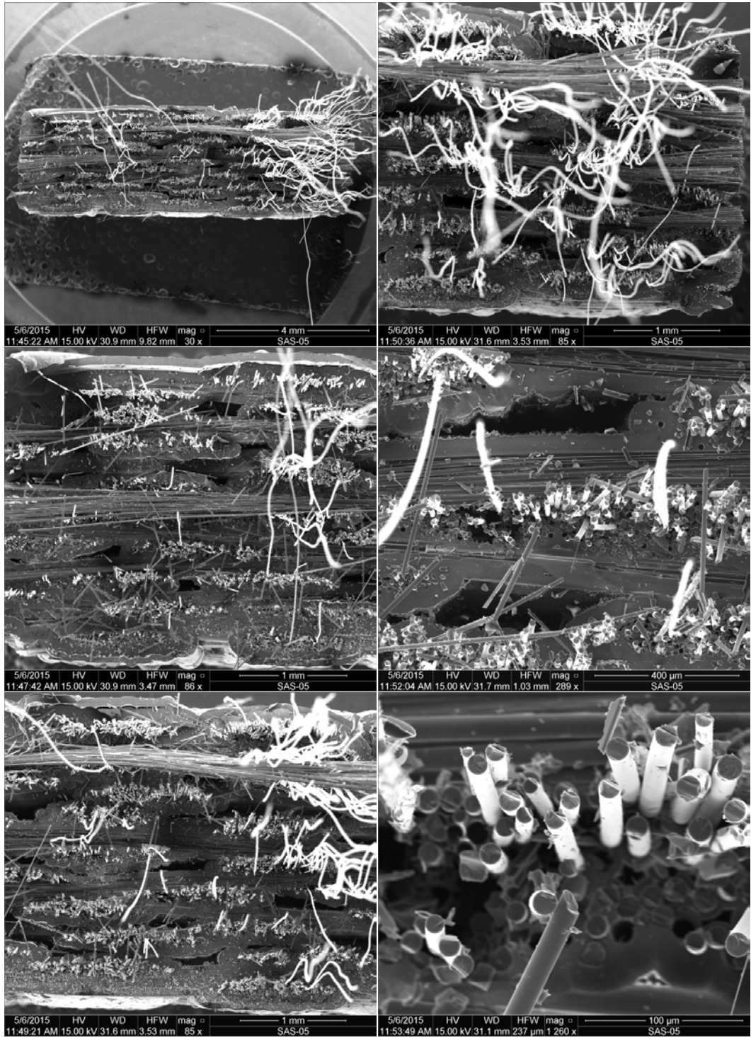
Figure M. 5: SEM micrographs of a fracture surface obtained in tensile test of a Hi-Nicalon™/HYPR-SiC™ specimen subjected to prior heat treatment for 10 h at 1400°C (Plate 11133, Specimen 2)
