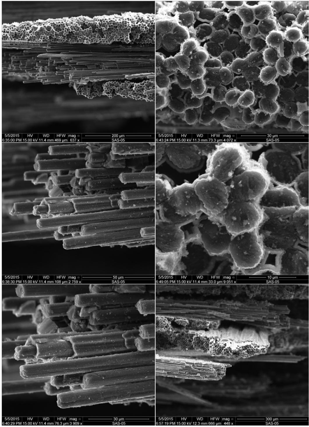
Figure L. 11: SEM micrographs of a fracture surface obtained in tensile test of a C/HYPR-SiC™ specimen subjected to prior heat treatment for 100 h at 1300°C (Plate 11121, Specimen 5)
