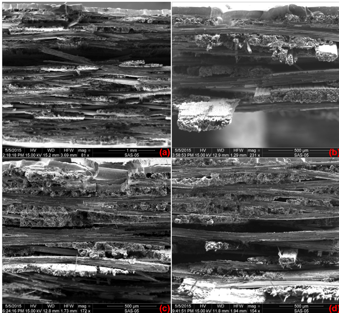
Figure 48: SEM micrographs of fracture surfaces obtained in tensile tests of C/HYPR-SiC™ – (a) virgin specimen; and specimens exposed for (b) 40 h at 1300°C; (c) 100 h at 1300°C; and (d) 100 h at 1200°C
