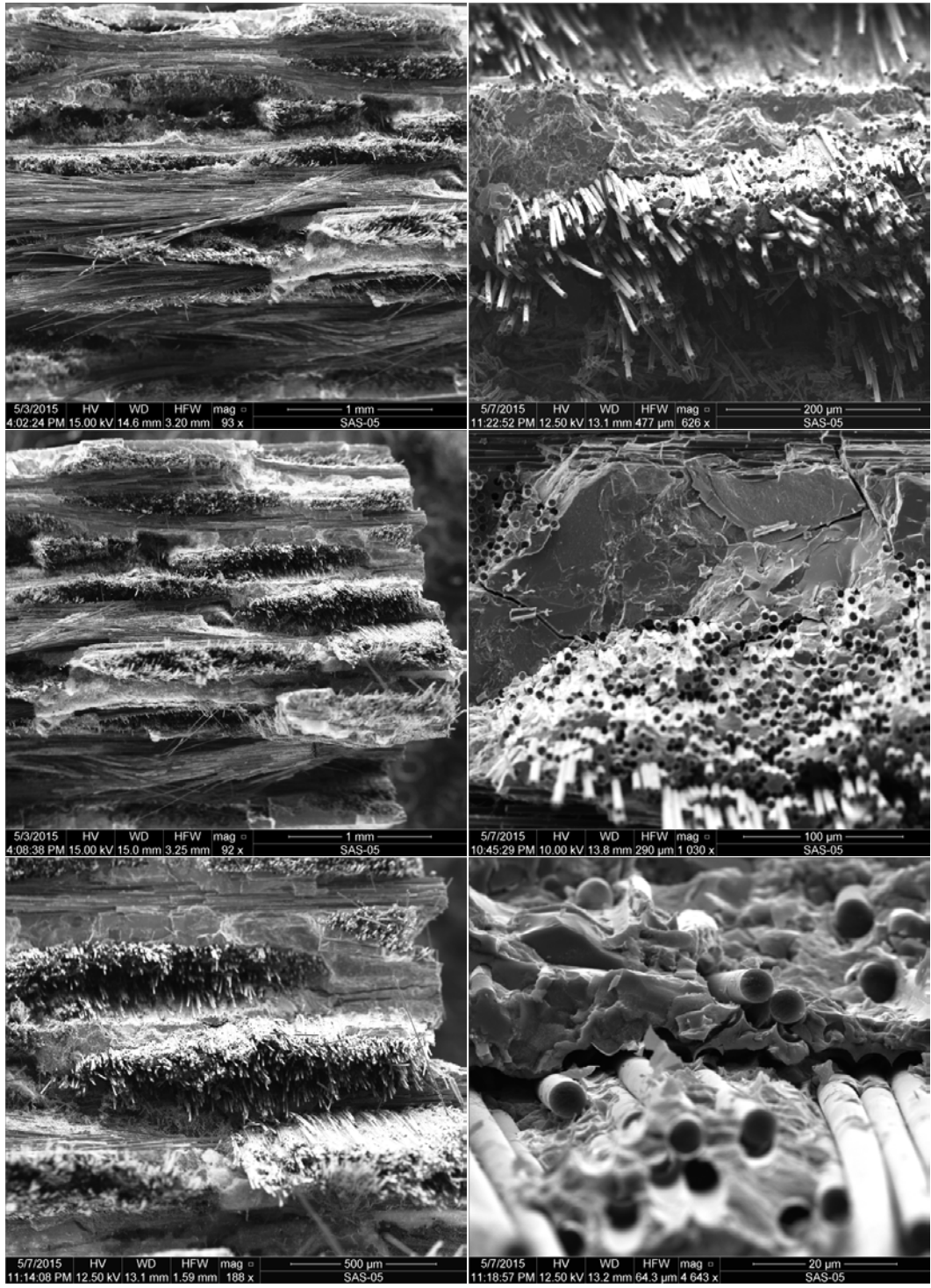
Figure K. 10: SEM micrographs of a fracture surface obtained in tensile test of a C/SiC specimen subjected to prior heat treatment for 40 h at 1300°C (Plate 12018, Specimen 2)
