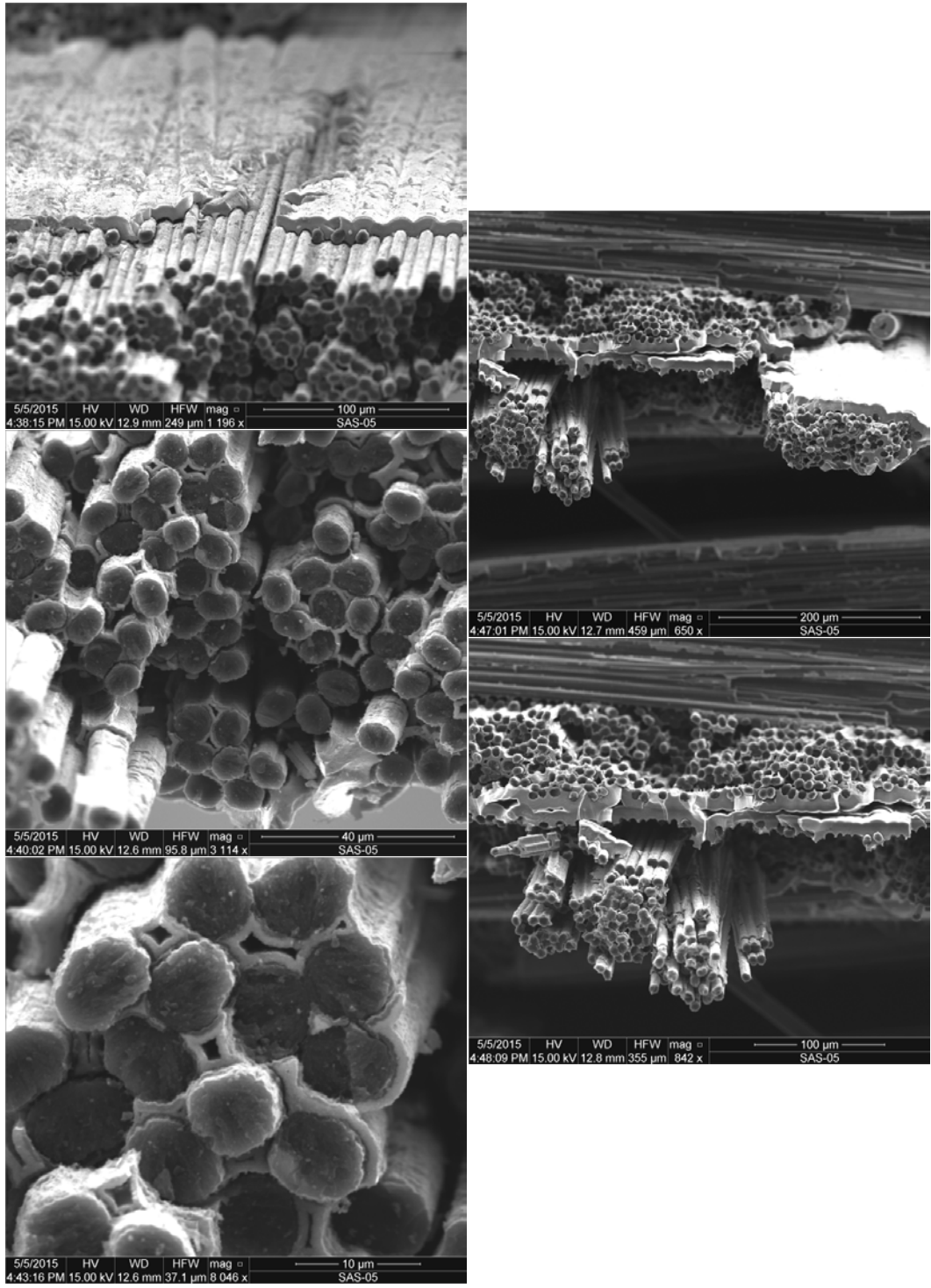
Figure L. 8: SEM micrographs of a fracture surface obtained in tensile test of a C/HYPR-SiC™ specimen subjected to prior heat treatment for 40 h at 1300°C (Plate 11125, Specimen 4)
