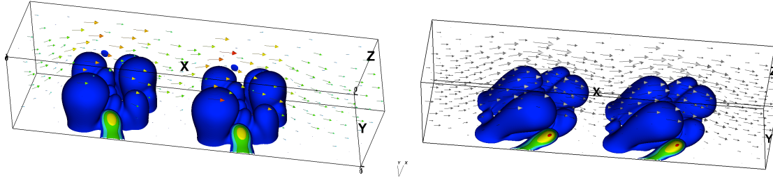
(a) \phi_n at t = 0
