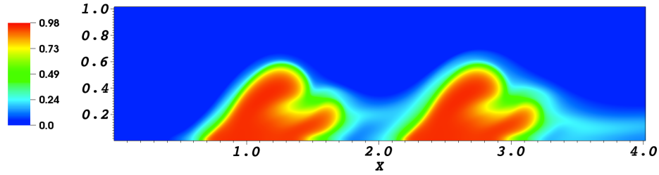
(e) 2D slice of AHL at z = 0.35
