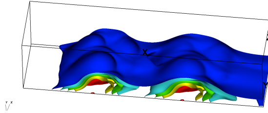
(c) AHL at t = 31
