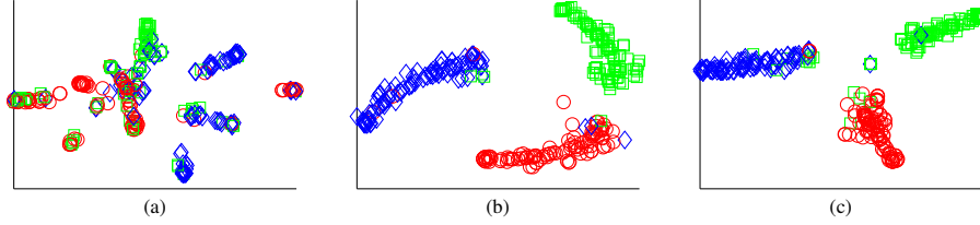
Figure 10: Projection of three classes of 20newsgroups onto the topical space by (a) FSTM, (b) FSTM c , and (c) MedLDA. FSTM did not provide a good projection in the sense of class separation, since label information was ignored. FSTM c and MedLDA actually found good discriminative topical spaces, and provided a good separation of classes.
