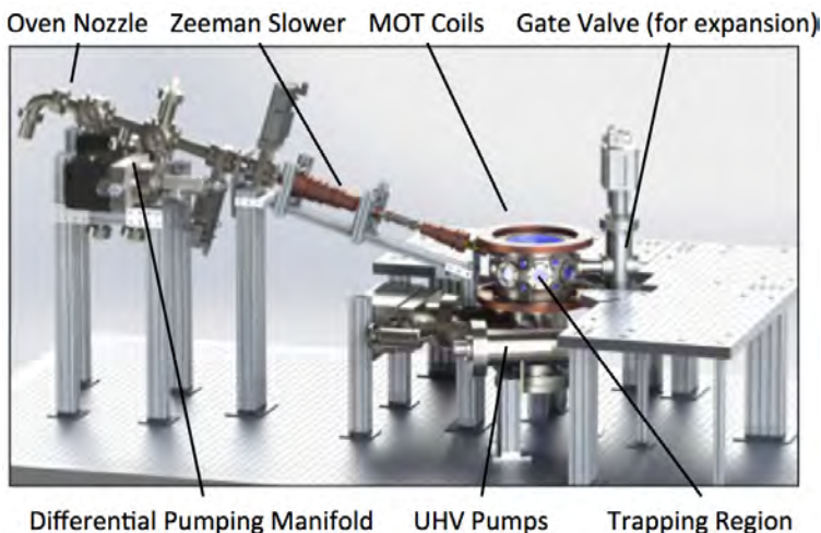
Figure 2: UCSB strontium apparatus. Left: Diagram of the strontium machine design. Right: The assembled machine in the PI's lab, with optical breadboards removed.
