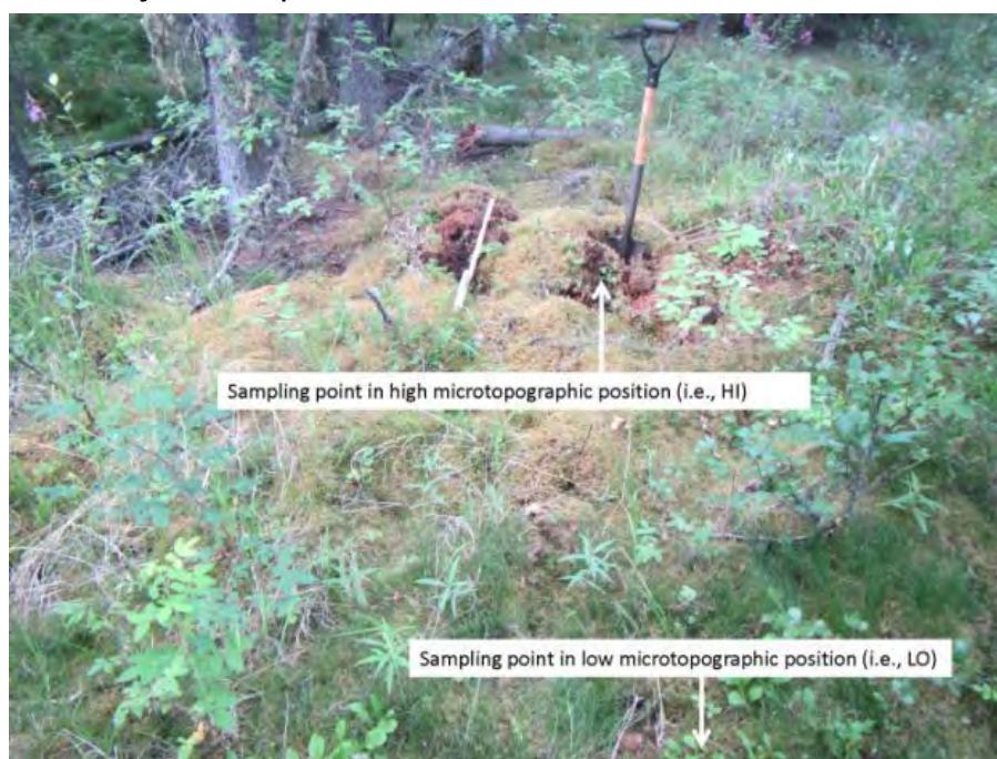
Figure 3. The sample layout displaying microtopographic high (HI) and low (LO) sample locations at the ERDC Farmers Loop Experimental Station. Note that adjacent sample locations are within one linear meter of each other.
