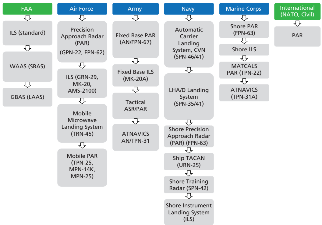
Figure 3.1 JPALS Interoperability
