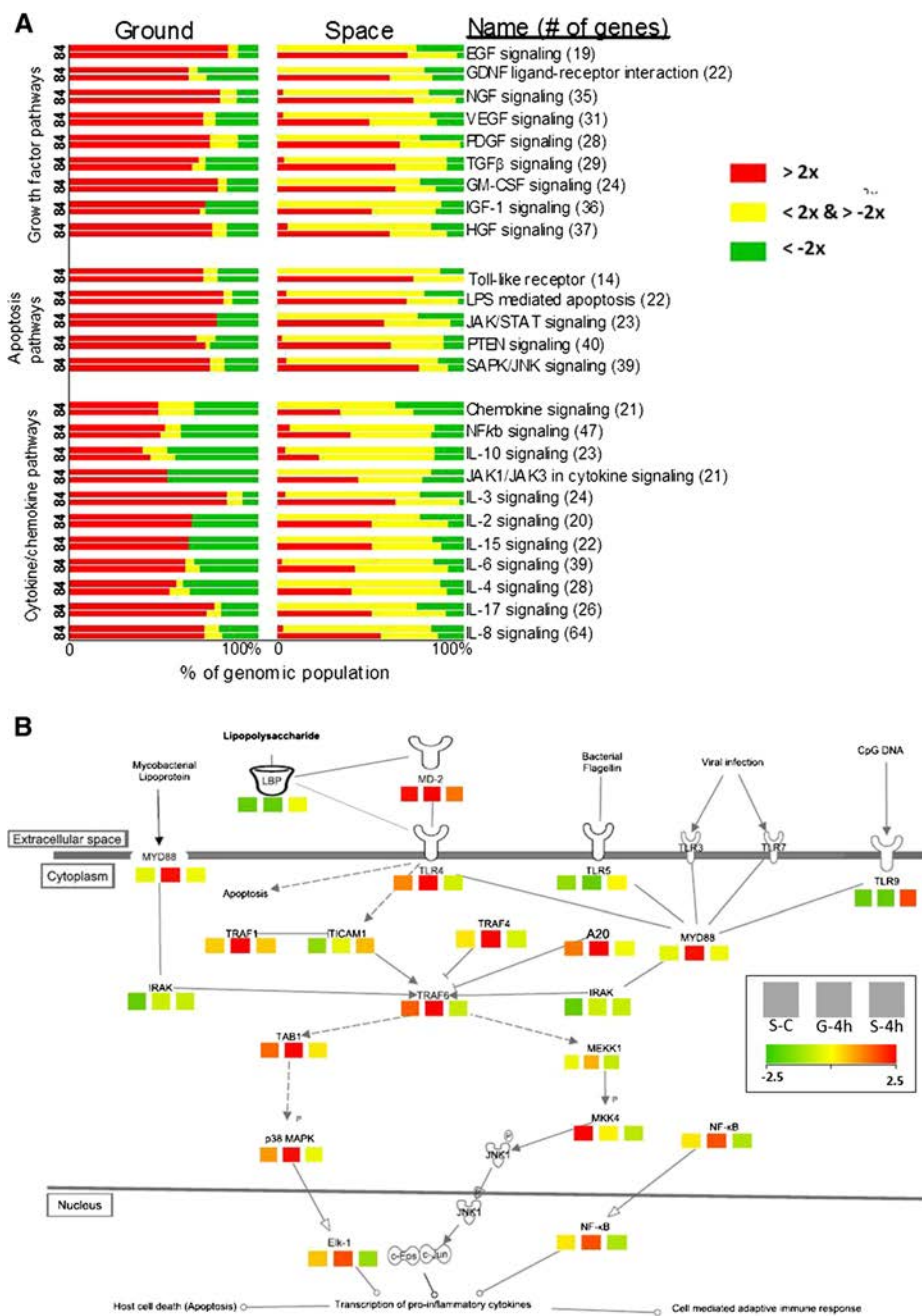
Figure 3 Enrichment profile of the immunologically relevant pathways significantly altered by Gol LPSμG with a focus on Toll like receptor (TLR) pathway co enriched by Gol LPSμG and Gol μG. A. Enrichment profile of the immunologically relevant pathways significantly altered in responding to LPS assault mediated by different gravitational forces. Twenty four most significantly enriched pathways were identified focusing on three parent nodes, namely cytokine/chemokine pathways (11 networks) apoptosis pathways (5 networks) and growth factor pathways (8 networks). For each network, there are four bars segregated into two columns (Ground and Space) and two rows (4 h and 8 h, which are noted as 4 and 8, respectively). The distributions of genomic regulations associated with each pathway are hereby documented for G 4 h, G 8 h, S 4 h and S 8 h and the pathways are batched into three parent pathways: cytokine/chemokine pathways, apoptosis pathways and growth factor pathways. The fraction of the elevated (fold change > 2) and suppressed (fold change < 2) transcripts are colored by red and green, respectively. The unchanged fractions are yellow. The color scheme is at the right. B. Toll like receptors (TLR) pathway. A schematic network of TLRs pathway is presented here. The TLRs pathway is significantly co enriched by both gene sets linked to LPS insult mediated by microgravity (Gol LPSμG) and exclusive effects of microgravity (Gol μG), respectively. There are three blocks beneath each gene name representing the transcriptomic regulations of S C (left most block), G 4 h (middle block) and S 4 h (right most block). G 8 h and S 8 h are omitted. The S C regulations normalized by G C (S C/G C) represent the exclusive impacts of microgravity. And, G 4 h and S 4 h normalized by respective controls (G 4 h/G C and S 4 h/S C) represent the influence of the gravitational shift on host response to LPS assault. The scale of the color scheme is included.
