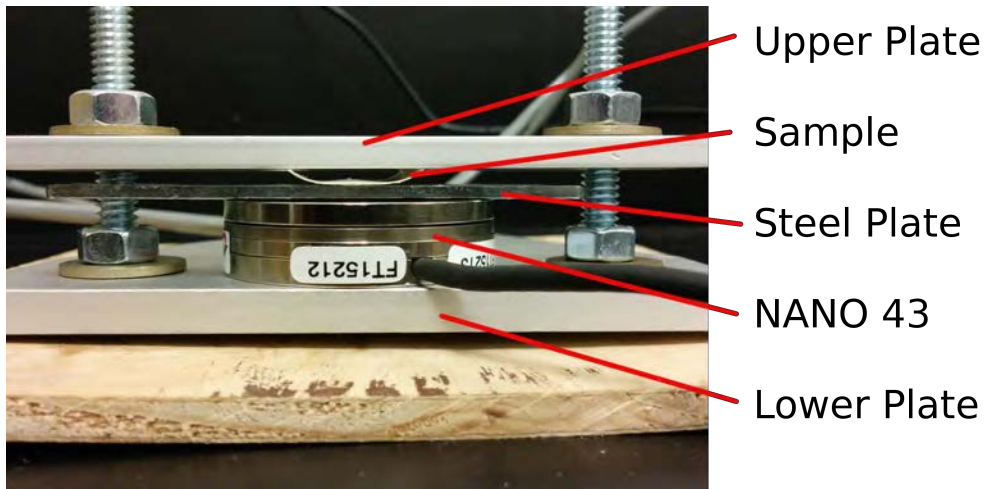
Figure 10. NANO 43 Flat Stress Relaxation Test Setup
