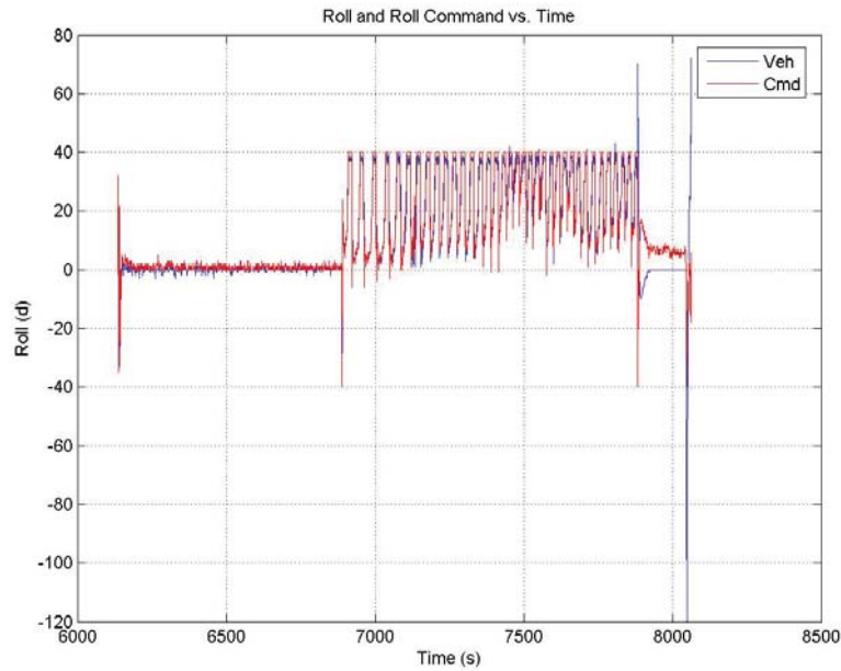
Figure 9: Roll control
