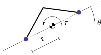
Figure 3. Simplified system used to derive feedback law
