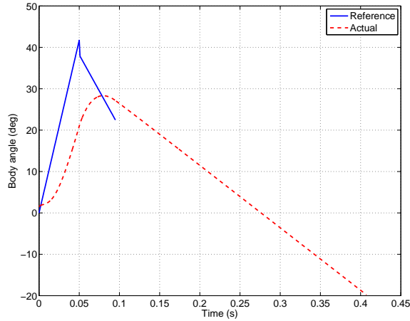
Figure 10. Reference trajectory for and actual values of body angle during the rear leg stance phase and the flight phase. The system is airborne after approximately 0.1 seconds, at which point the body rotates at nearly a constant angular velocity, i.e., with the spine remaining close to its neutral position. The front leg contacts the ground at the end of the trajectory shown.
