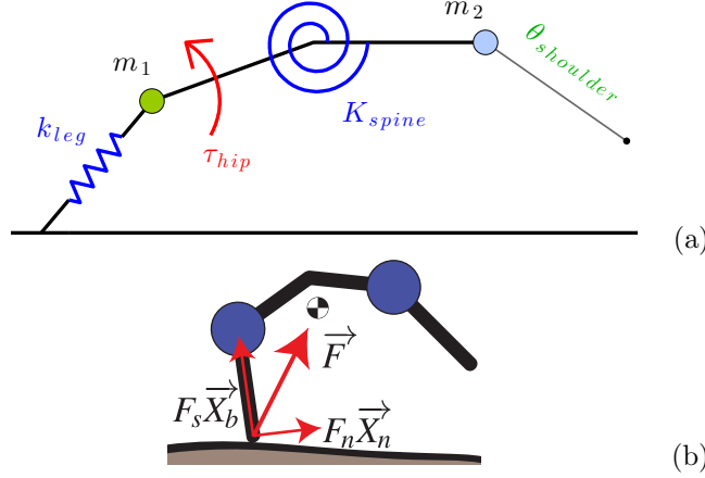
Figure 2. (a) Schematic model of the planar quadruped model showing the point masses, springs, and hip actuator. Dampers in parallel with the springs are not illustrated, for compactness and clarity. Only the first three links affect the dynamics, since the last link (past \theta_{shoulder} ) is modeled as massless. (b) Simplified view showing ground reaction force vector, orthogonal force components, and center of mass. Note that the magnitude of F_s is determined by the compression of the leg spring, while F_n is directly affected by \tau_{hip} .
