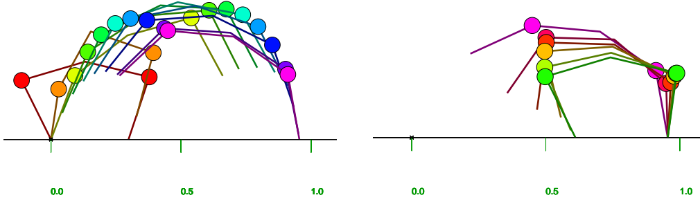
Figure 8. Animation of stable gait. Poses shown are snapshots at increments of 0.05 seconds, with a final frame included when impact of a leg with the ground occurs, ending a given phase of the gait. The left image includes the stance phase for the rear leg and the subsequent flight phase of the system, while the right image shows the stance phase for the front leg, in which the rear leg is reset for the next push-off.
