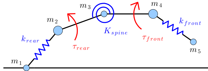
Figure 1. Planar 5-Mass Model Schematic, with a passive spine, torques at front and rear hips, and a small unsprung mass at each of the feet.
