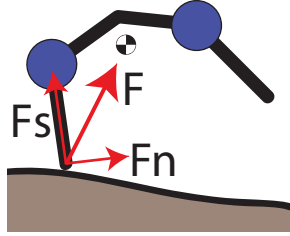
Figure 7. Ground reaction force vector F , and components F_s and F_n
