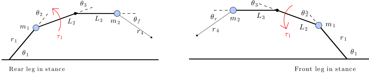
Figure 4. Definitions of angles and lengths for the two-mass planar model. Spring-damper assembly at the stance leg and at the flexible spine are not shown, for clarity. Lengths L_2 , L_3 and r_4 are constant lengths, while r_1 varies with leg spring length. The model is symmetry, front to back, so that relabelling occurs at each impact, as shown. Impact dynamics of the front leg result in an instantaneous lift-off of the rear foot, so that there is at most one leg in contact with the ground during steady bounding of the model.
