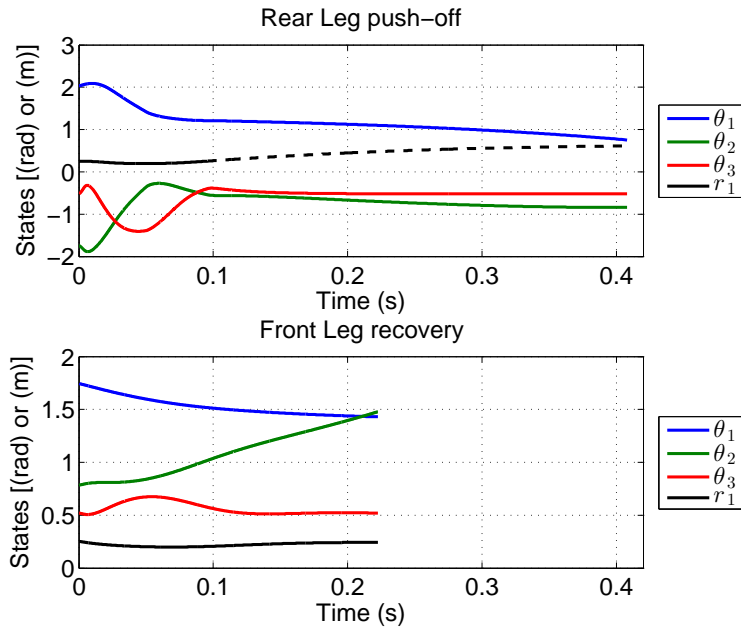
Figure 9. Joints and sprung leg length over time. Top plot corresponds to push-off and flight phases (at left in Fig. 8), and data in bottom plot corresponds to the phase in which front leg touches the ground (at right in Fig. 8). The black lines shows the distance from each respective ground contact (rear or front stance leg) to the next hip joint, and the dashed line indicates when this distance exceeds the neutral spring length, at which point the true leg is at its undeflected lengths and the system is in its flight phase.
