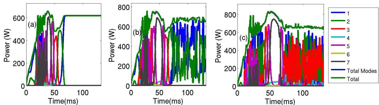
Figure 2. Evolution of the output modal composition of co-pumped amplifiers in time. The launched pump powers were (a) 700 Watts, (b) 800 Watts, and (c) 900 Watts. The launched seed contained 15.0 Watts in the fundamental mode and 0.75 Watts in the first higher order mode with no frequency shift between them. The modal decomposition is relative to the cold fiber modes identified in Figure 1.
