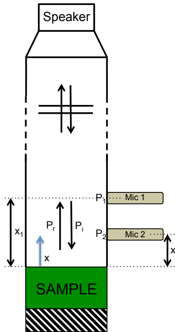
Figure 5.1: The impedance tube, here shown in a vertical orientation, has a speaker housed at the top, two microphones flush mounted to the inner wall of the tube, and a test sample that is rigid mounted to the lower end of the tube. The speaker launches sound toward the test sample which is measured by the two microphones.
