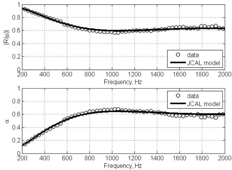
Figure 5.2: (Top) Reflection and (Bottom) Absorption coefficient of blue sand. Sample thickness is equal to 5cm, \phi = 0.41 , particle radius r = 250 \mu m . Gray circles are impedance tube data. Black line is the JCAL model with parameters estimated using the cell model
